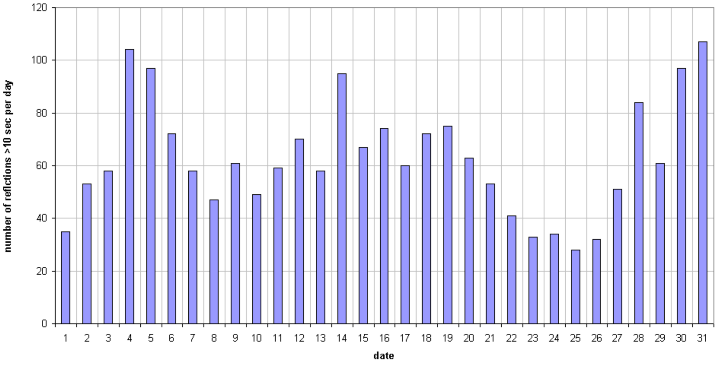
49.99MHz - RadioMeteors May 2017 daily totals of all overdense reflections Felix Verbelen (Kamphenhout)
