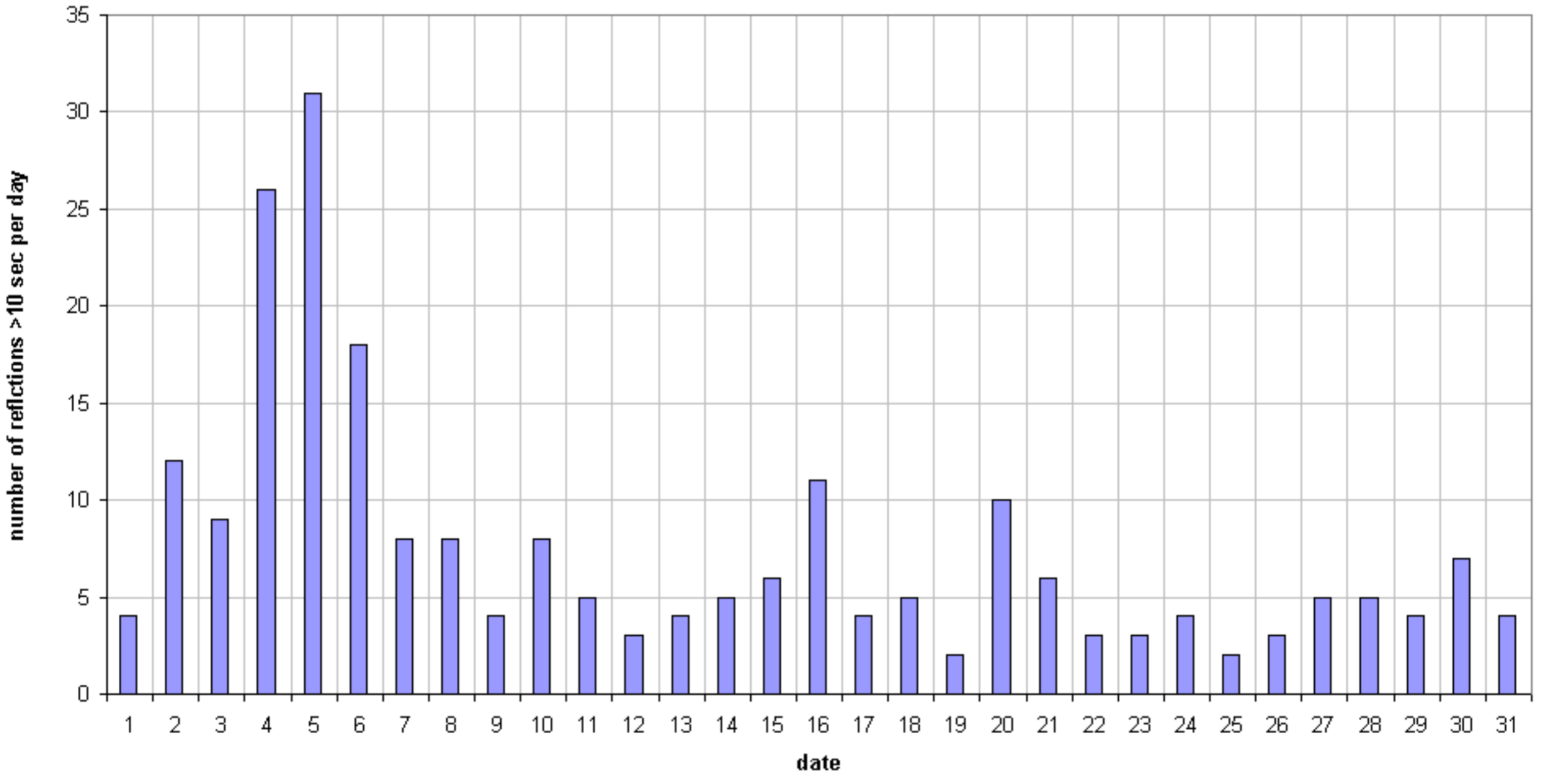
49.99MHz - RadioMeteors May 2017 daily totals of reflections longer than 10 seconds Felix Verbelen (Kamphenhout)
