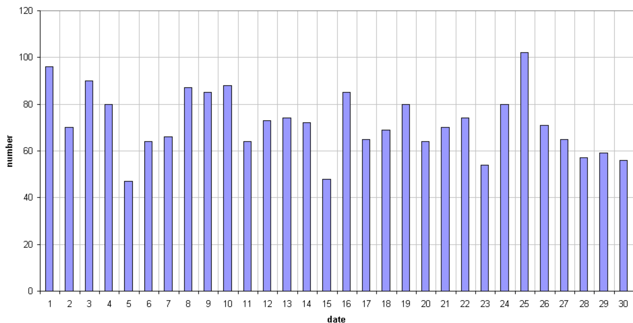
49.99MHz - RadioMeteors September 2018 daily totals of all overdense reflections Felix Verbelen (Kamphenhout)
