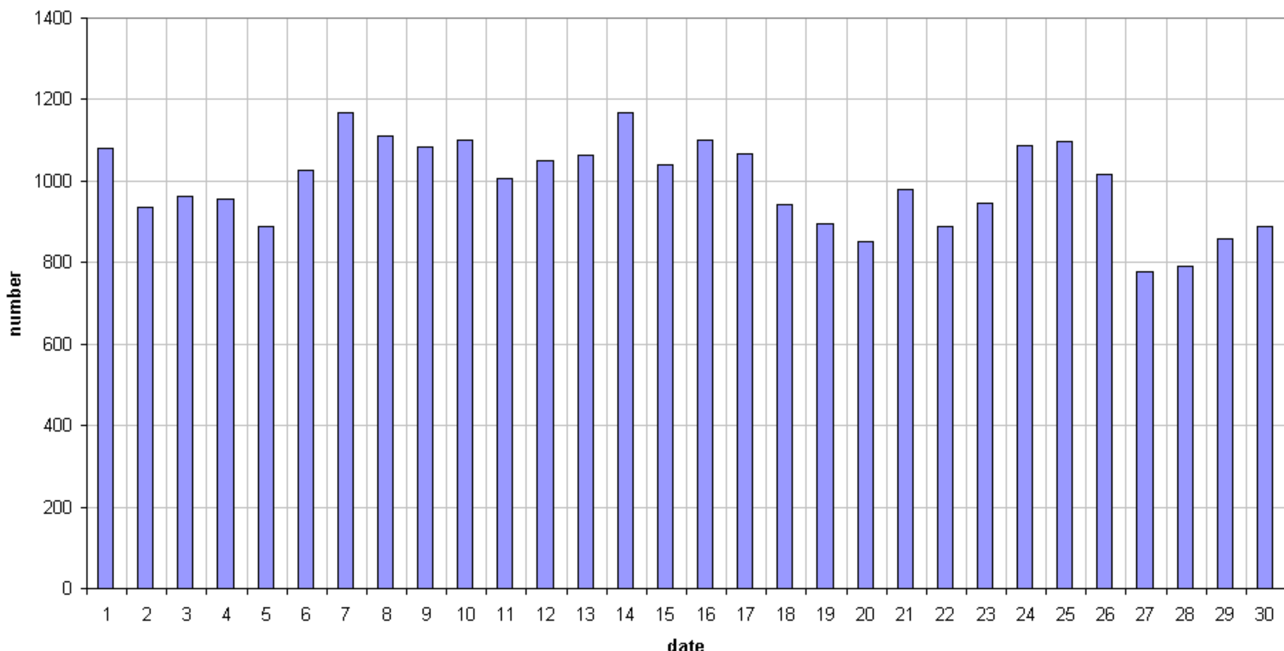
49.99MHz - RadioMeteors September 2018 daily totals of "all" reflections (automatic count_Mette15_7Hz) Felix Verbelen (Kamphenhout)
