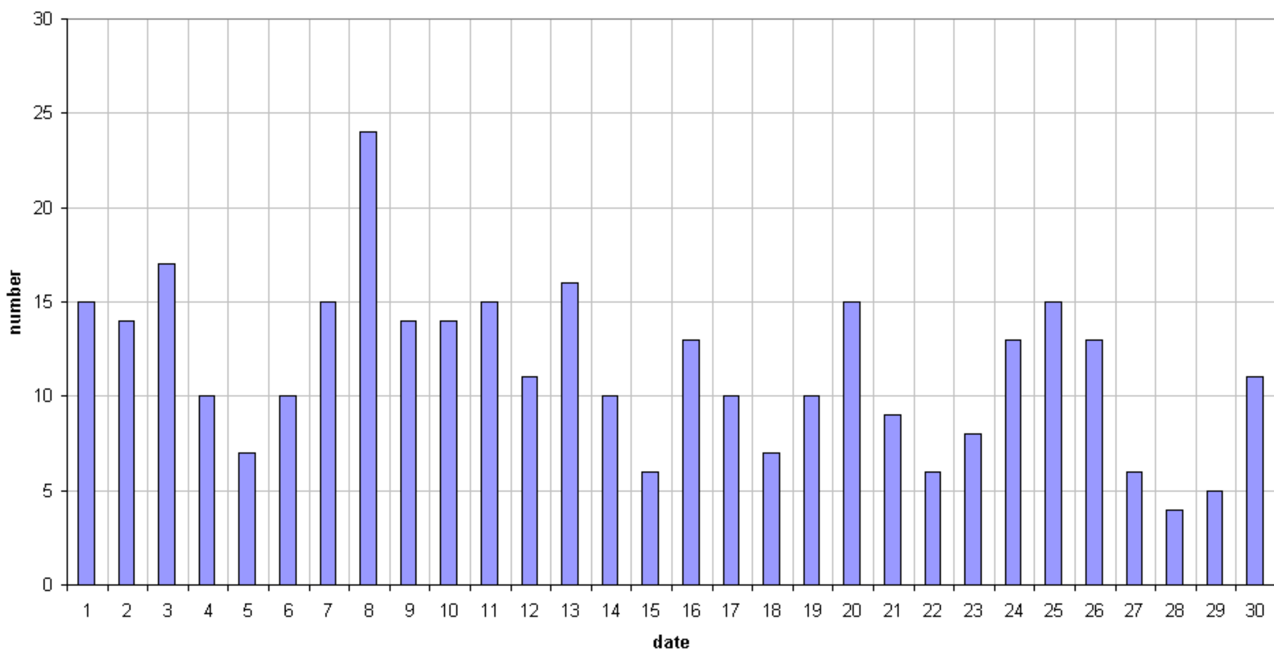
49.99MHz - RadioMeteors September 2018 daily totals of reflections longer than 10 seconds Felix Verbelen (Kamphenhout)
