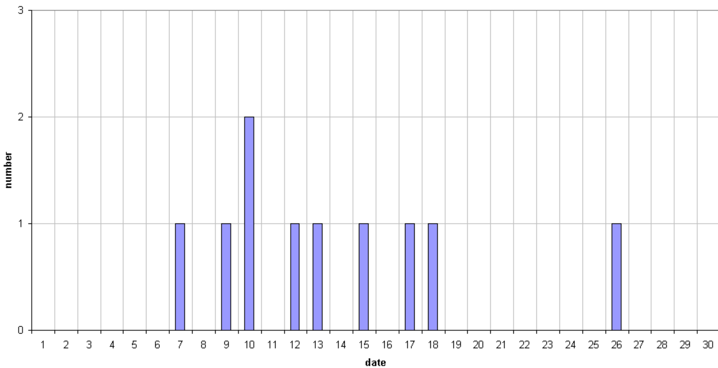
49.99MHz - RadioMeteors September 2018 daily totals of reflections longer than 1 minute Felix Verbelen (Kamphenhout)
