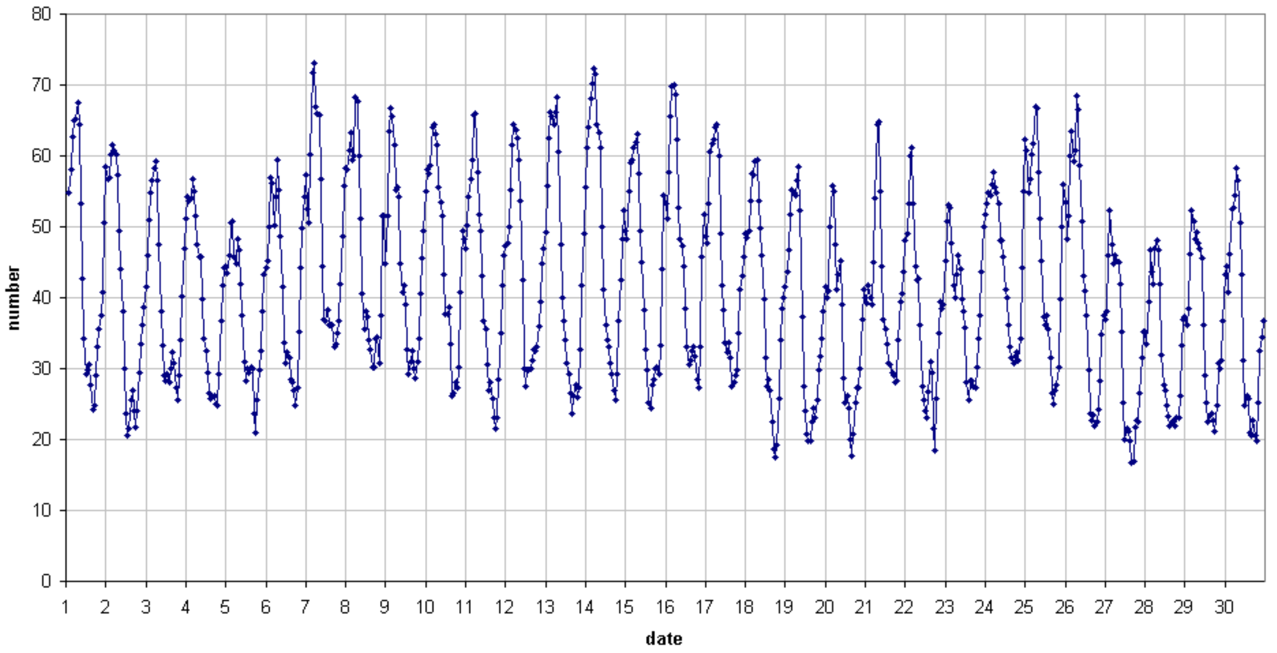
49.99 MHz - RadioMeteors September 2018 number of "all" reflections per hour (weighted average) (automatic count_Mette15_7Hz) Felix Verbelen (Kamphenhout)
