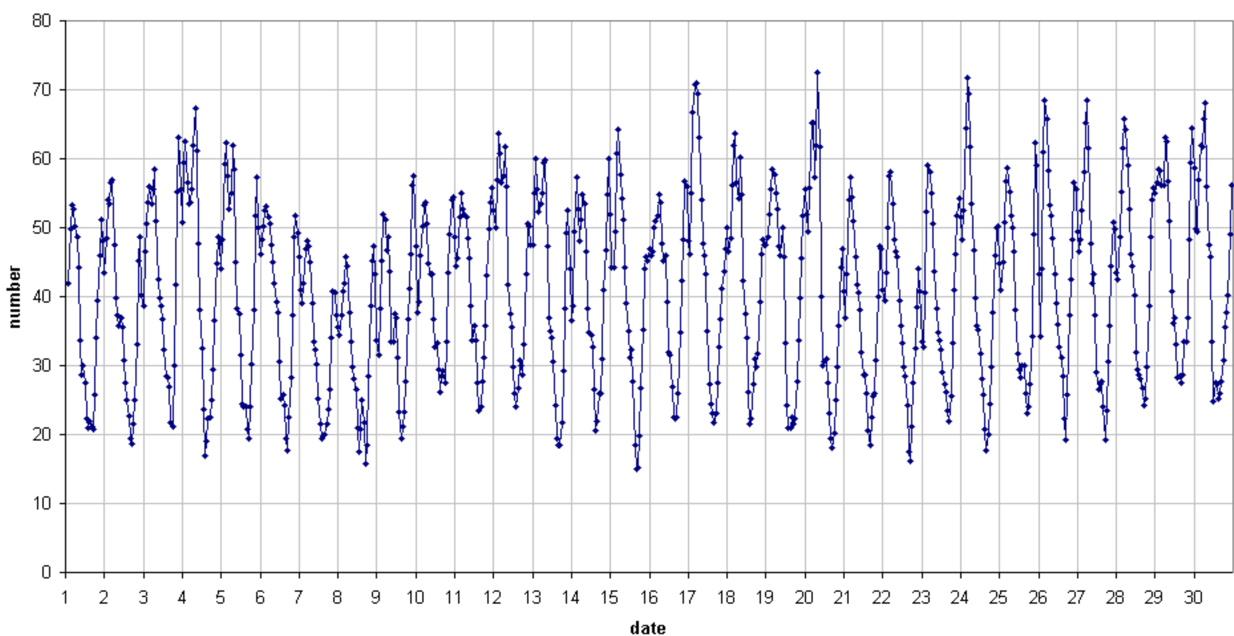
49.99 MHz - RadioMeteors November 2018 number of "all" reflections per hour (weighted average) (automatic count_Mette5_7Hz) Felix Verbelen (Kamphenhout)
