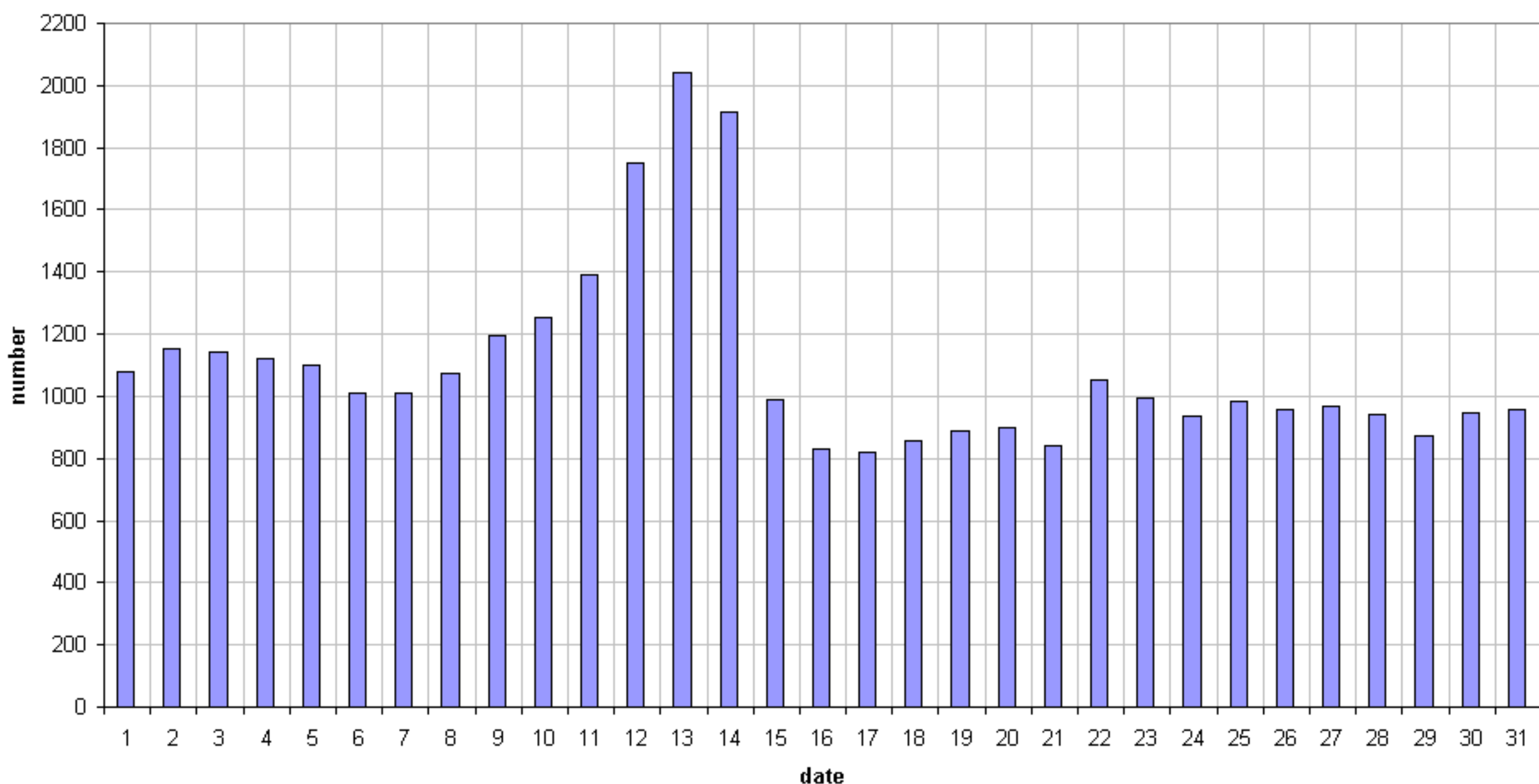
49.99MHz - RadioMeteors December 2018 daily totals of "all" reflections (automatic count_Mette16_7Hz) Felix Verbelen (Kampenhout)
