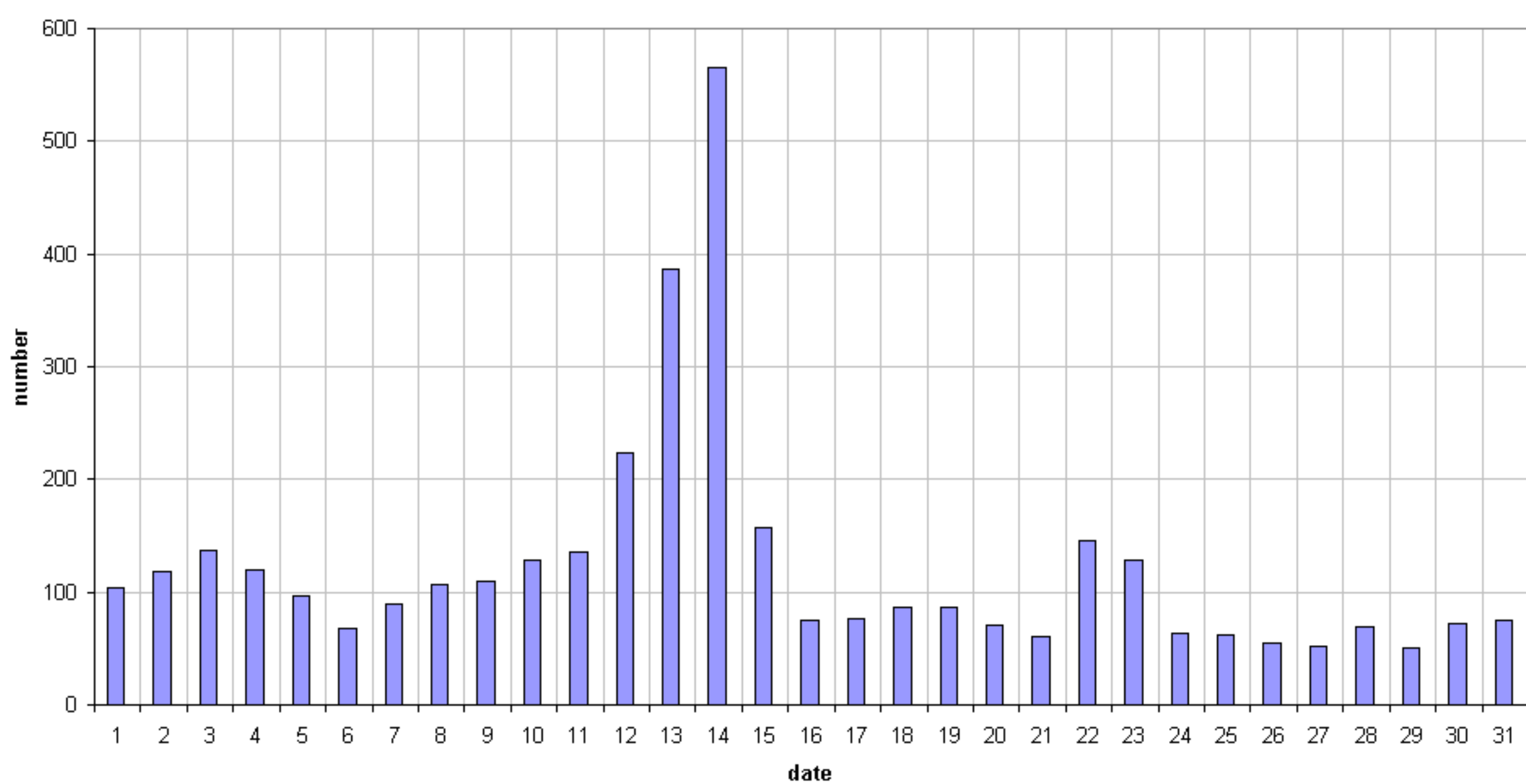
49.99MHz - RadioMeteors December 2018 daily totals of all overdense reflections Felix Verbelen (Kampenhout)
