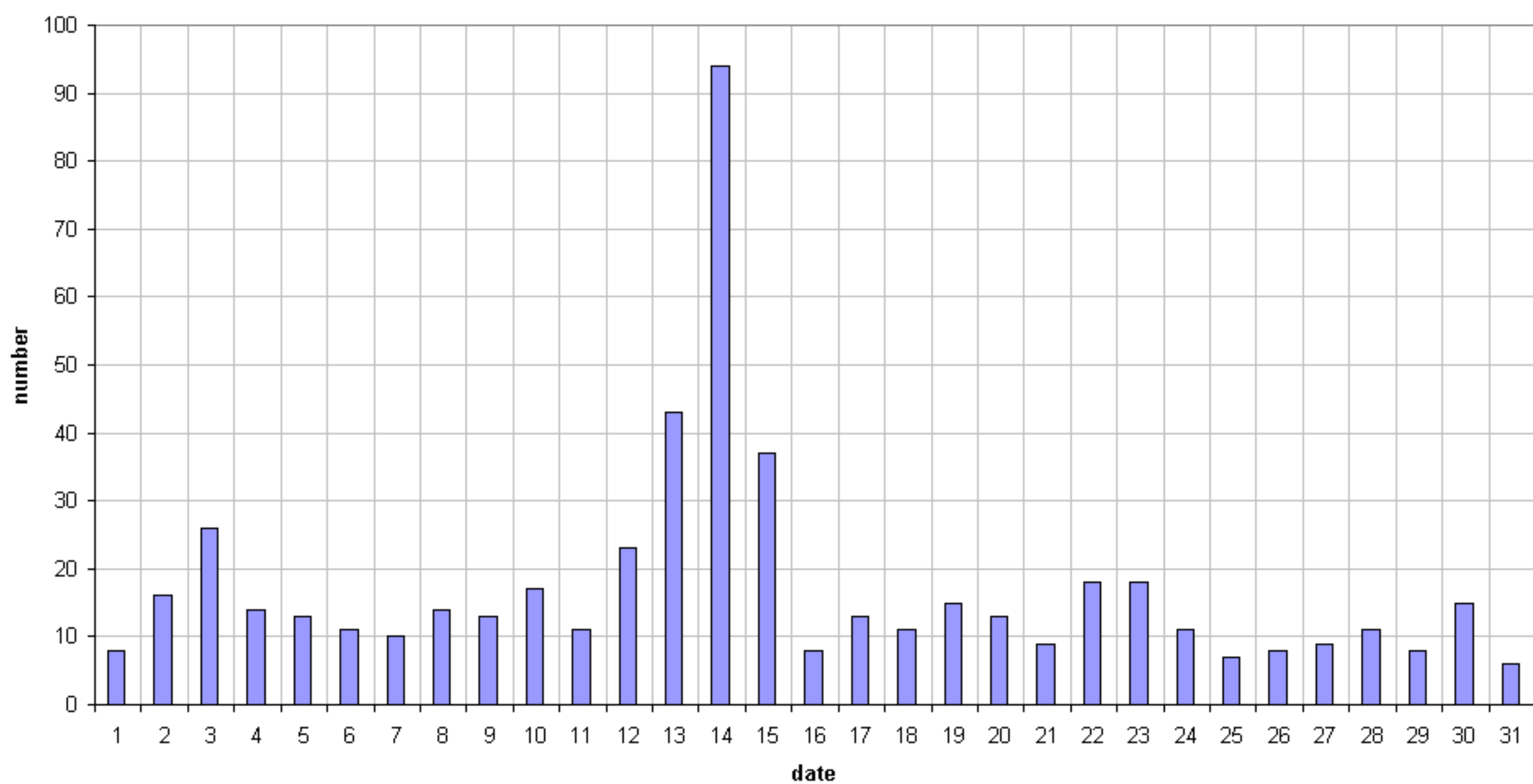
49.99MHz - RadioMeteors December 2018 daily totals of reflections longer than 10 seconds Felix Verbelen (Kampenhout)
