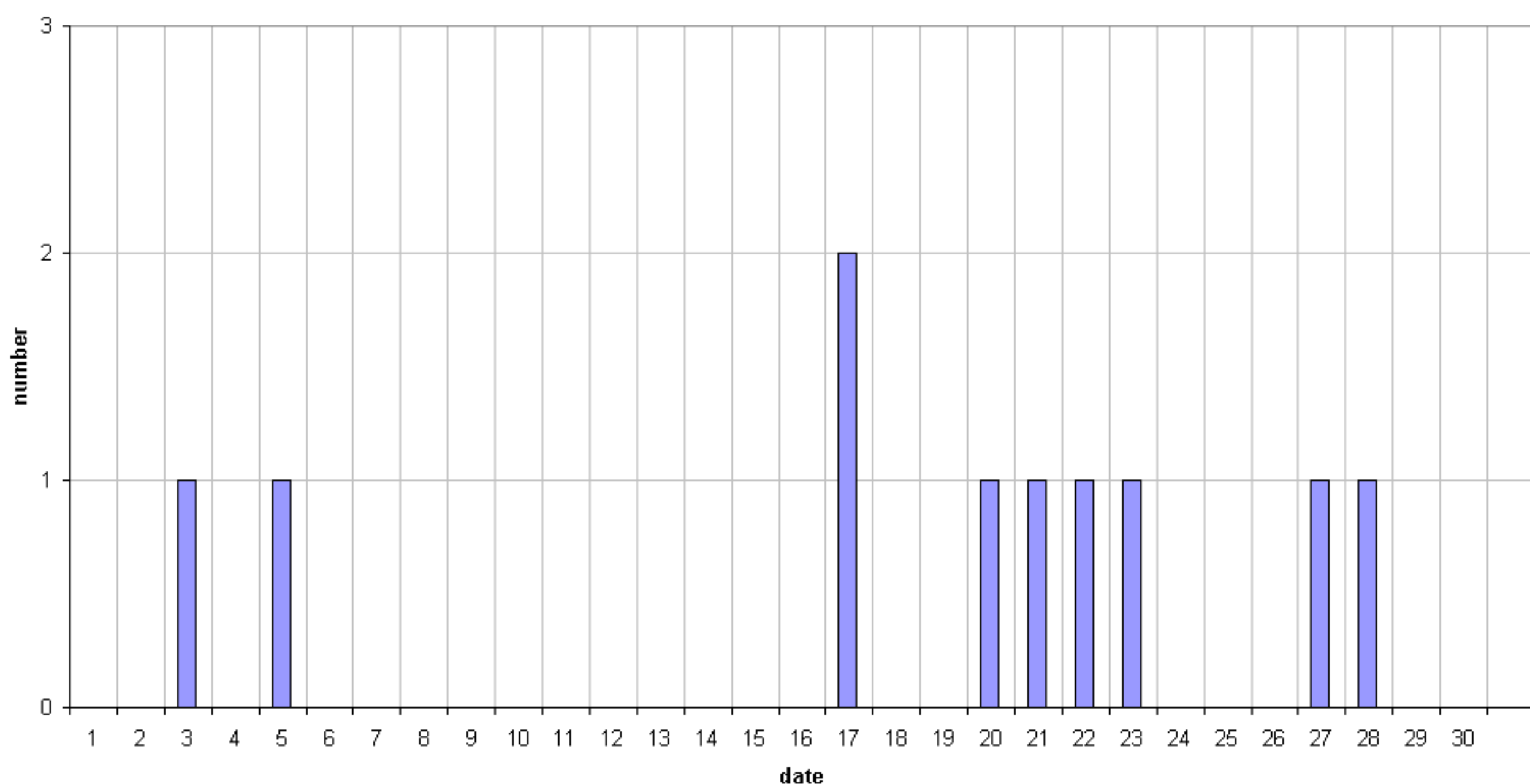
49.99MHz - RadioMeteors December 2018 daily totals of reflections longer than 1 minute Felix Verbelen (Kampenhout)
