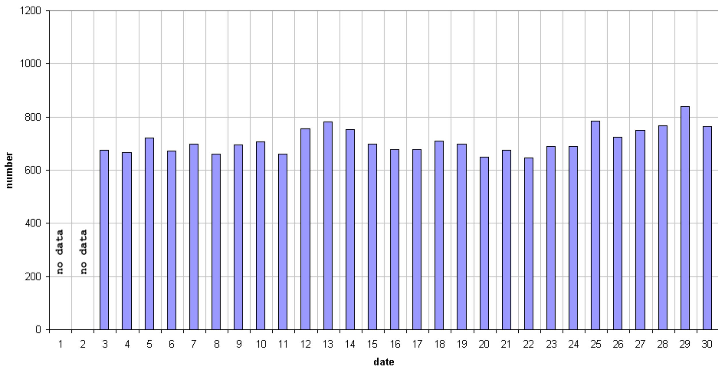
49.99MHz - RadioMeteors April 2019 daily totals of "all" reflections (automatic count_Mettel5_7Hz) Felix Verbelen (Kamphenhout)
