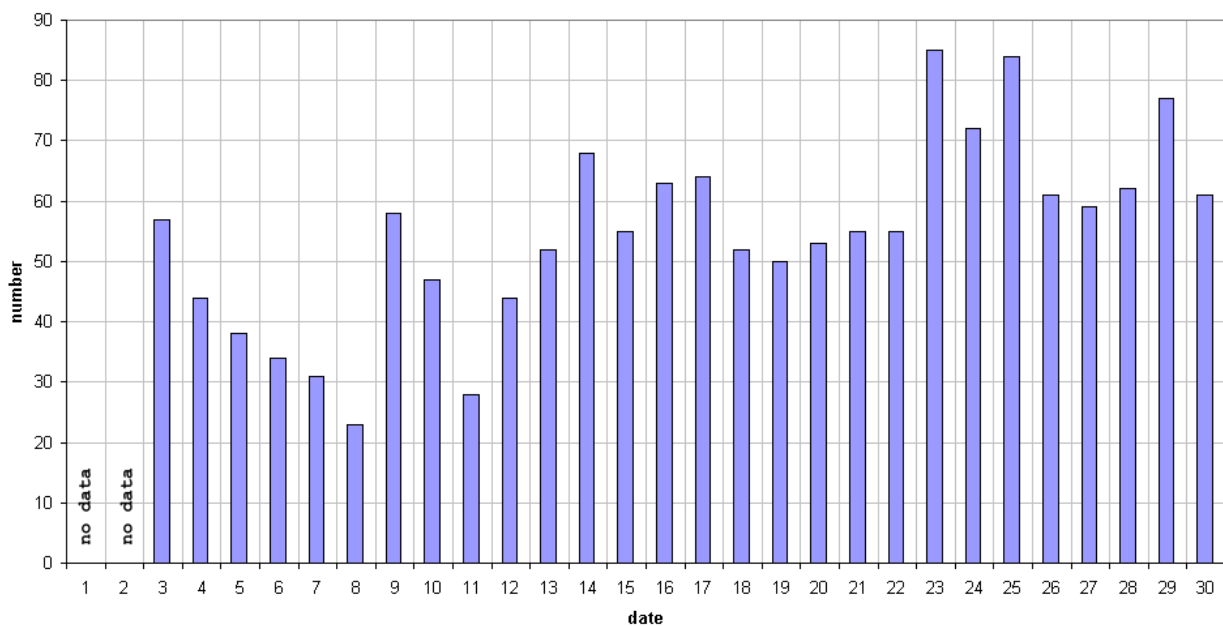
49.99MHz - RadioMeteors April 2019 daily totals of all overdense reflections Felix Verbelen (Kamphenhout)
