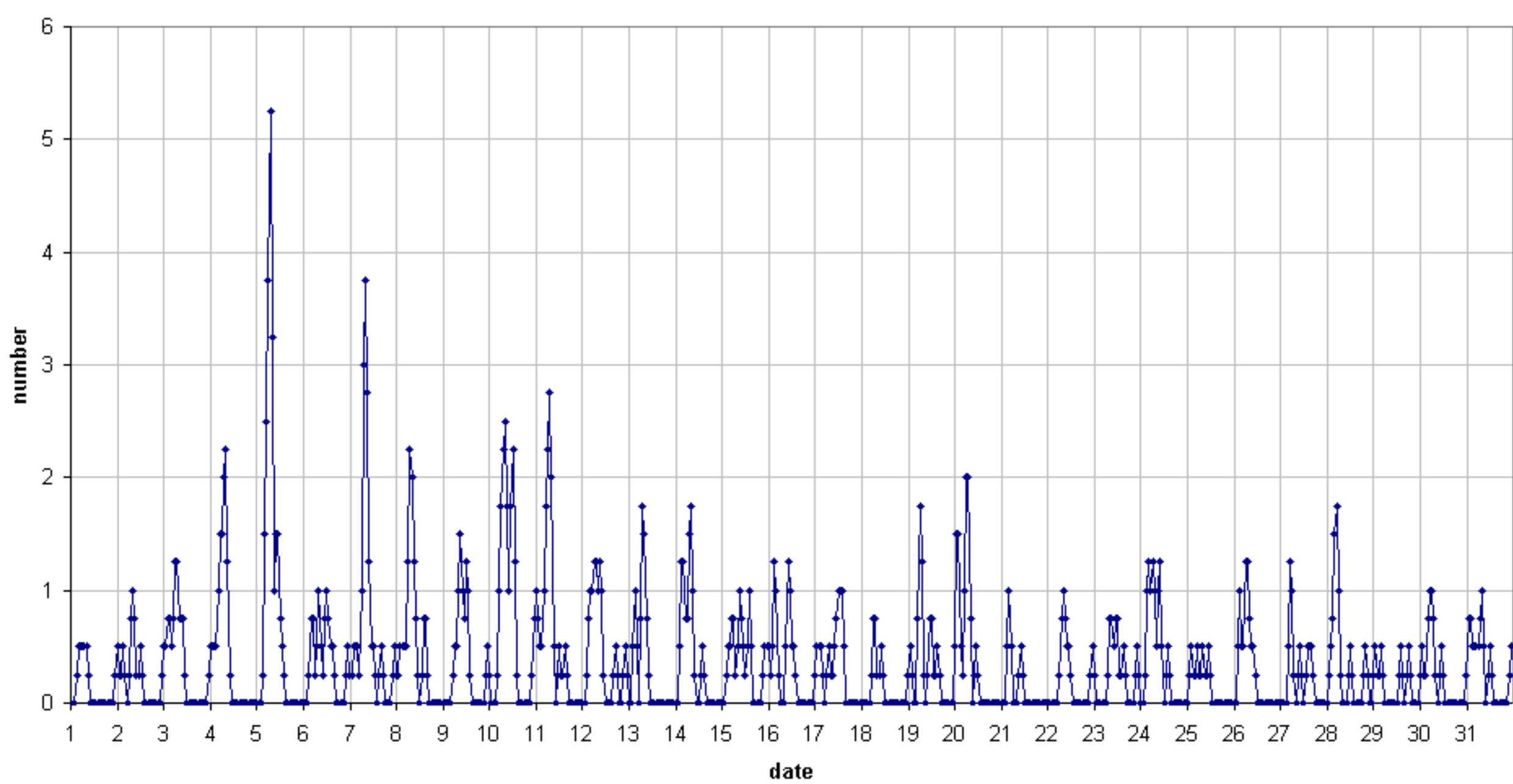
49.99MHz - RadioMeteors May 2019 number of reflections >10 seconds per hour (weighted average) Felix Verbelen (Kamphenhout)
