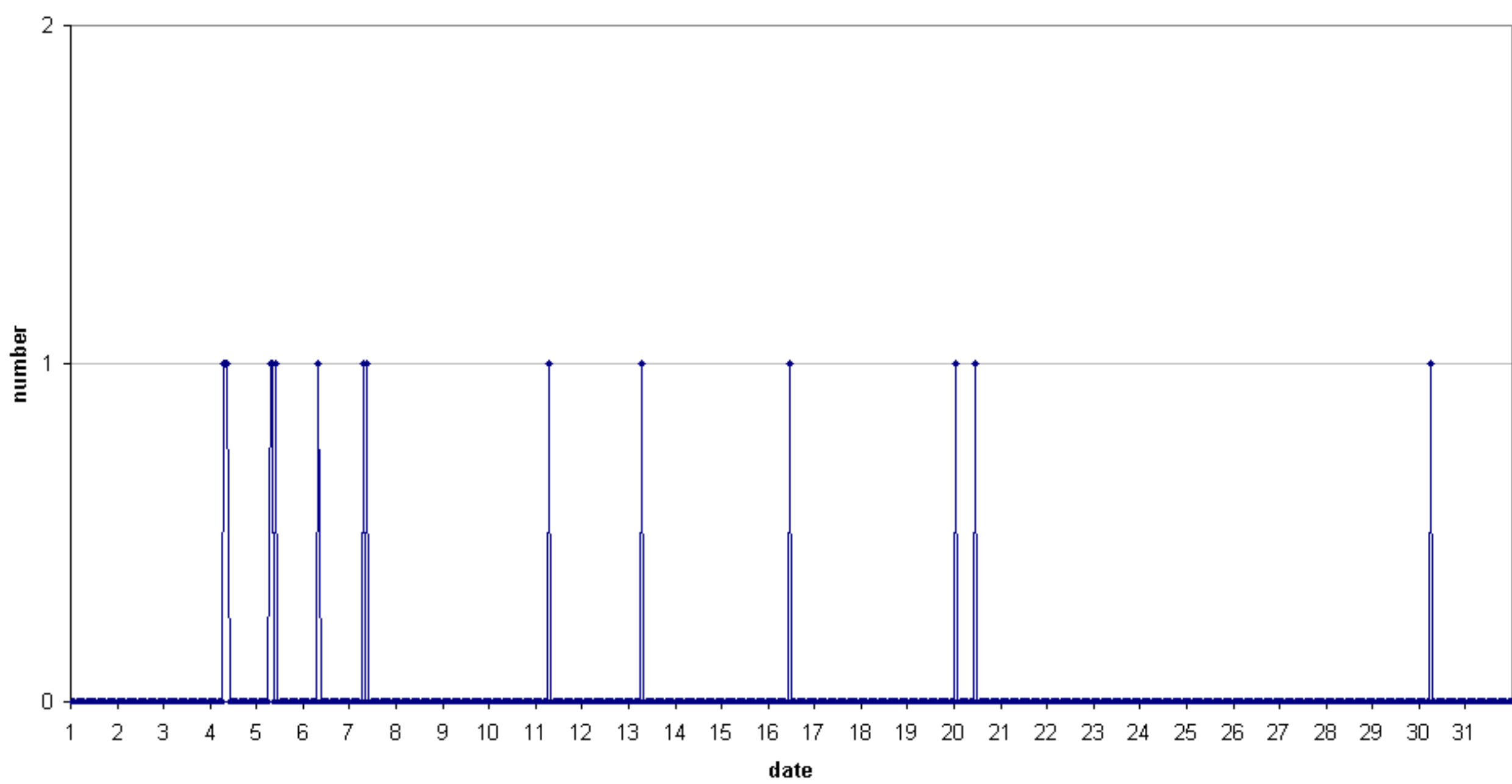
49.99MHz - RadioMeteors May 2019 hourly totals of overdense reflections longer than 1 minute Felix Verbelen (Kamphenhout/BE)
