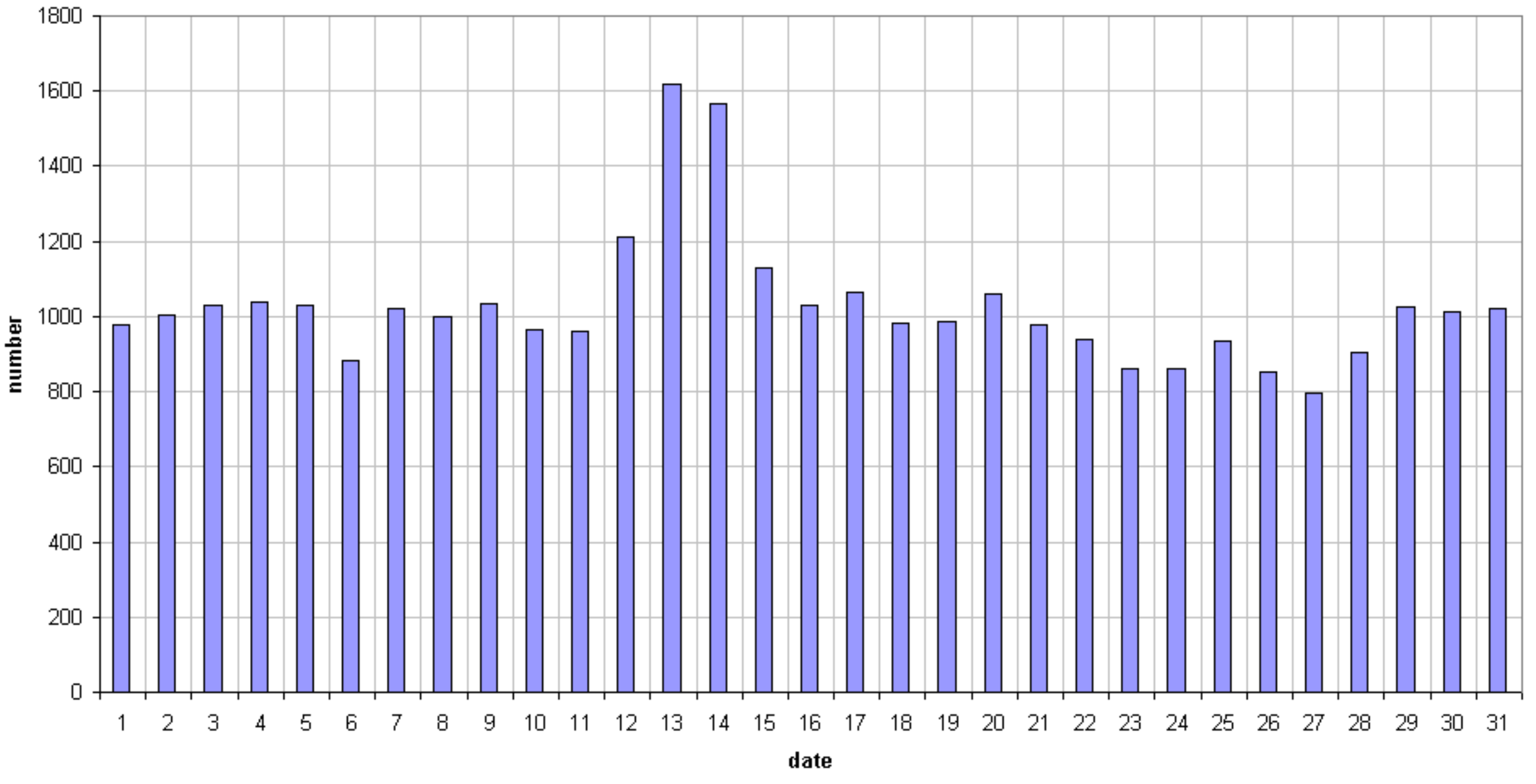
49.99MHz - RadioMeteors August 2019 daily totals of "all" reflections (automatic count_Mette15_7Hz) Felix Verbelen (Kamphenhout)
