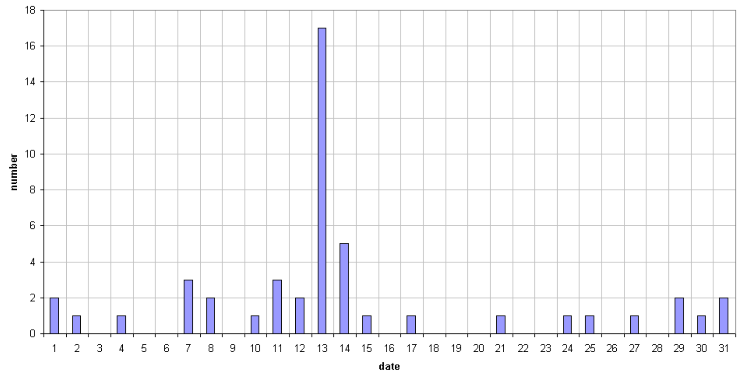
49.99MHz - RadioMeteors August 2019 daily totals of reflections longer than 1 minute Felix Verbelen (Kamphenhout)
