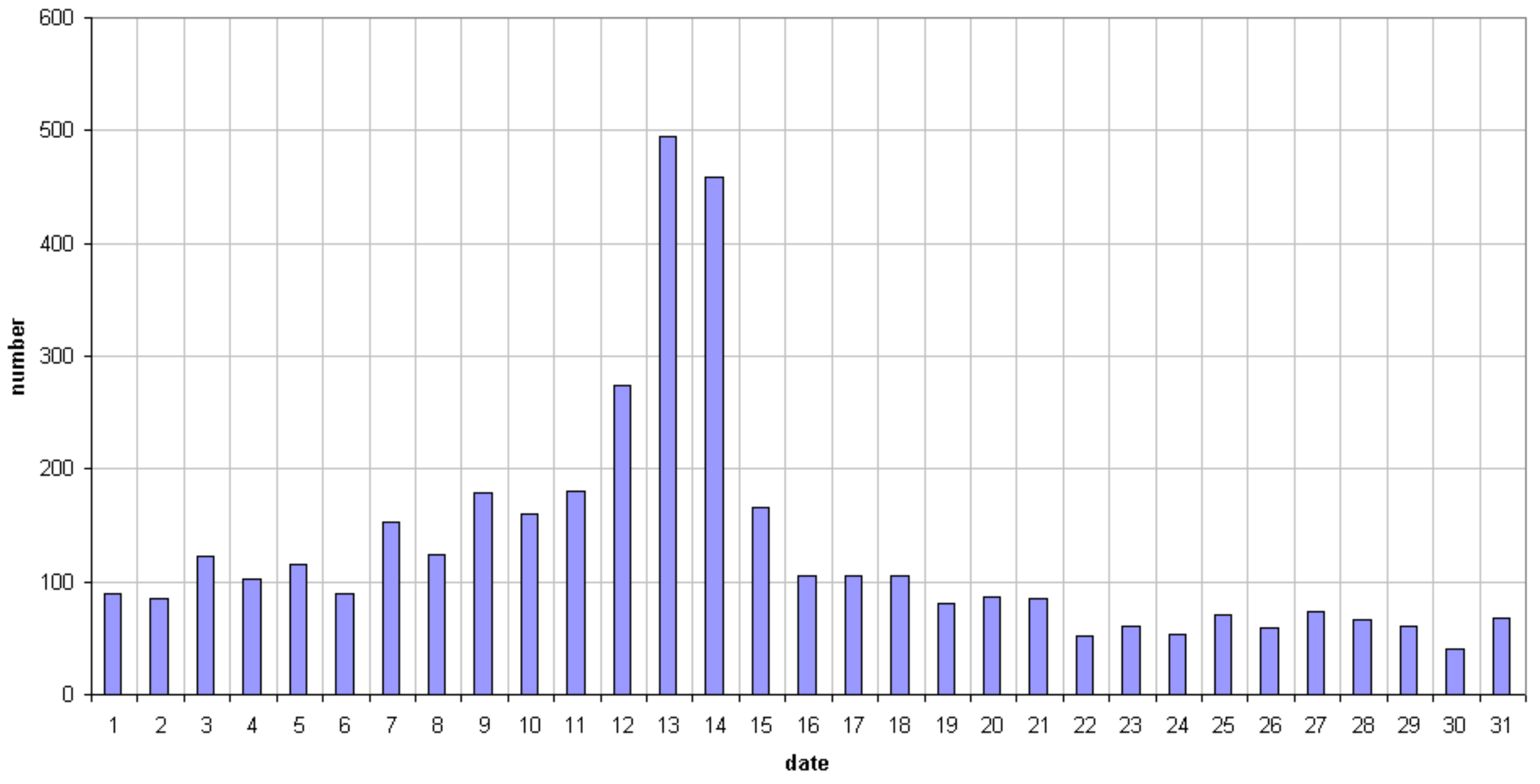
49.99MHz - RadioMeteors August 2019 daily totals of all overdense reflections Felix Verbelen (Kamphenhout)
