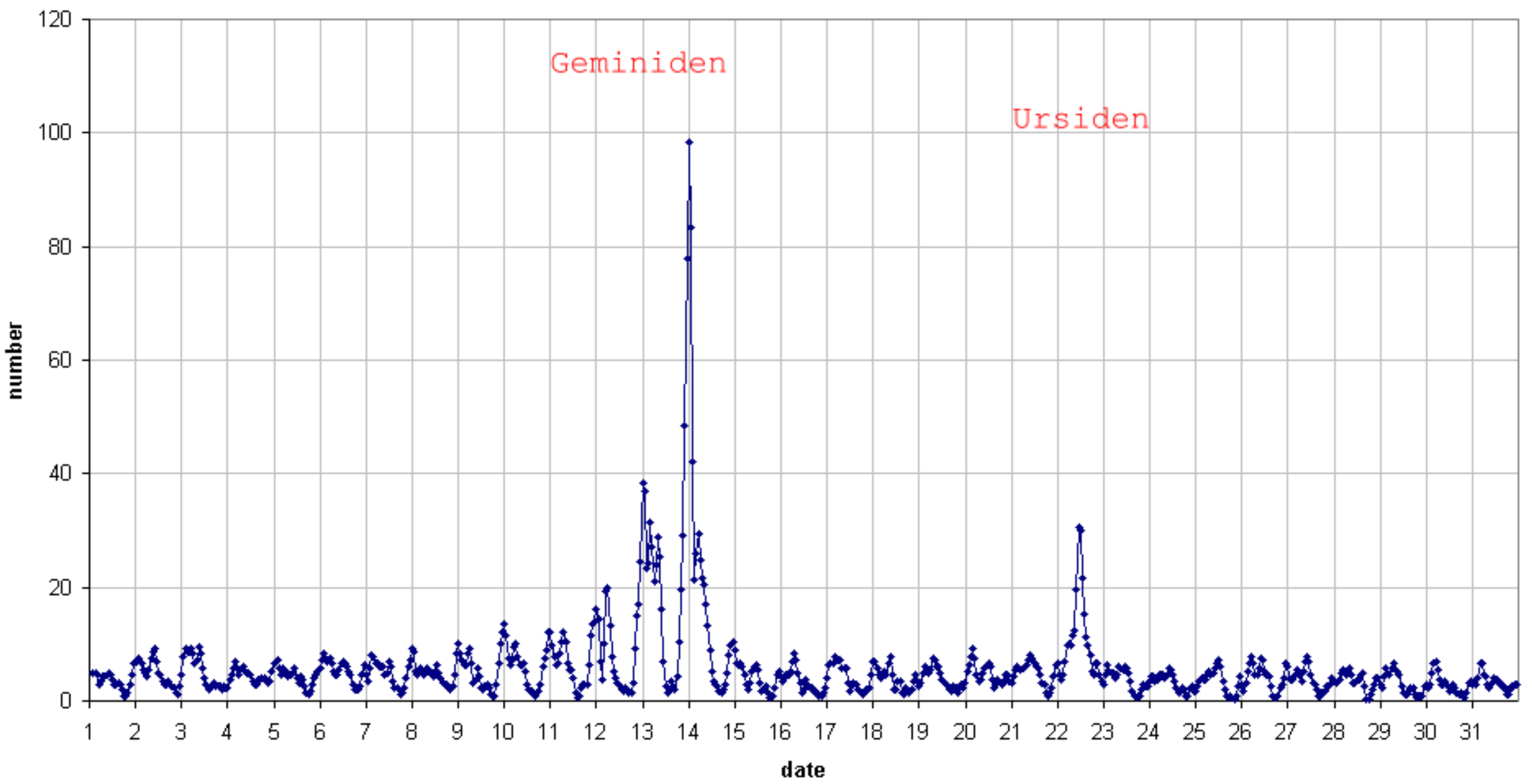
49.99MHz - Radiometeors December 2016 number of "all overdense reflections" per hour (weighted average)_(manual count) Felix Verbelen (Kampenhout)
