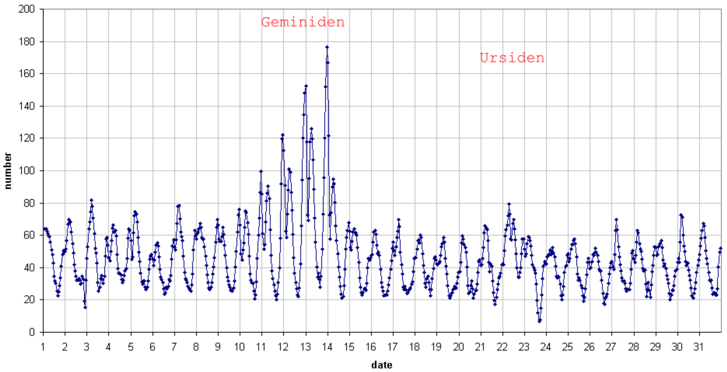
49.99 MHz - Radiometeors December 2016 number of "all reflections" per hour (weighted average) (automatic count_Mettel4_7Hz) Felix Verbelen (Kampenhout)
