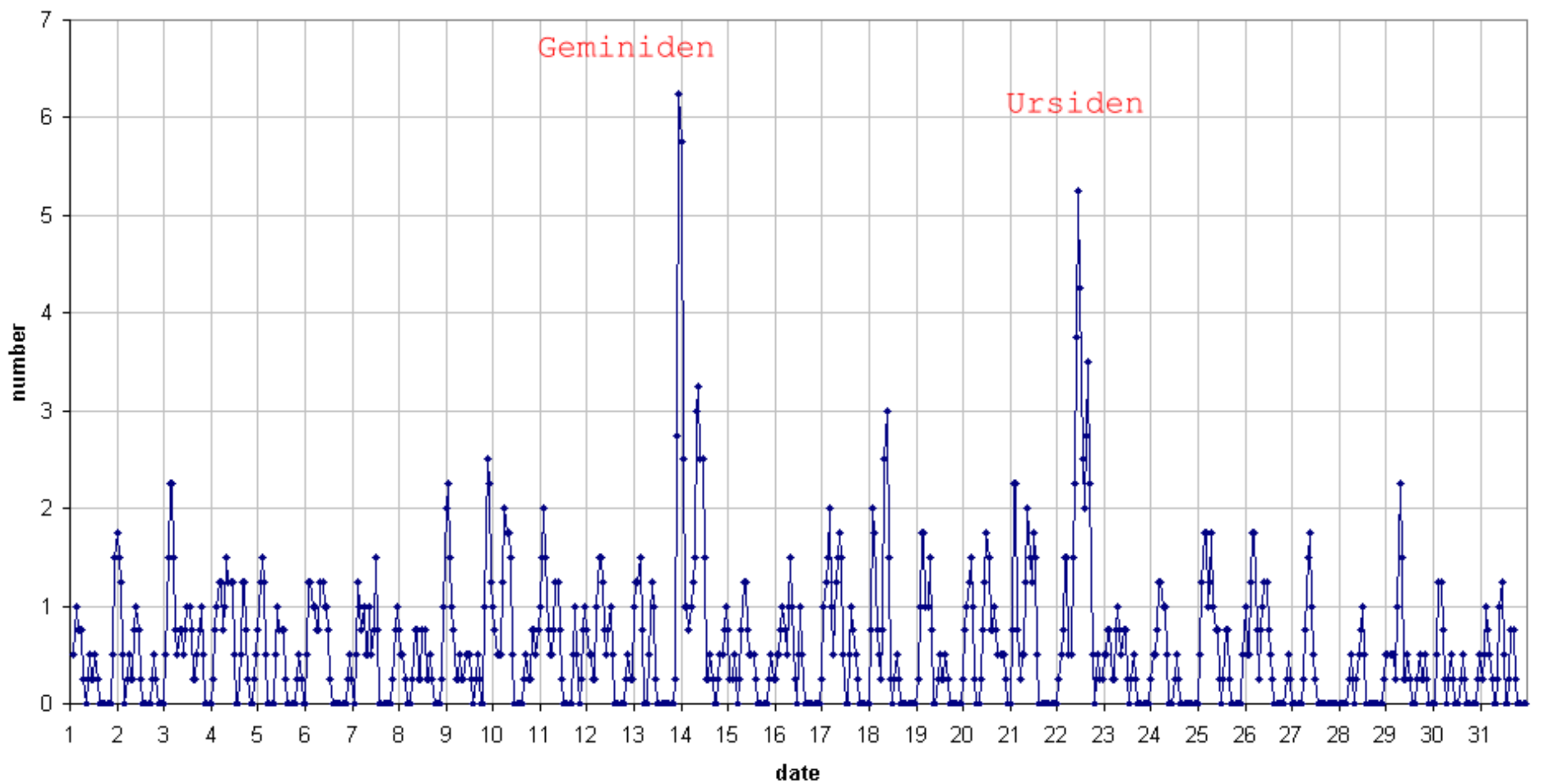
49.99MHz - Radiometeors December 2016 number of "reflections >10 seconds" per hour (weighted average)_(manual count) Felix Verbelen (Kampenhout)
