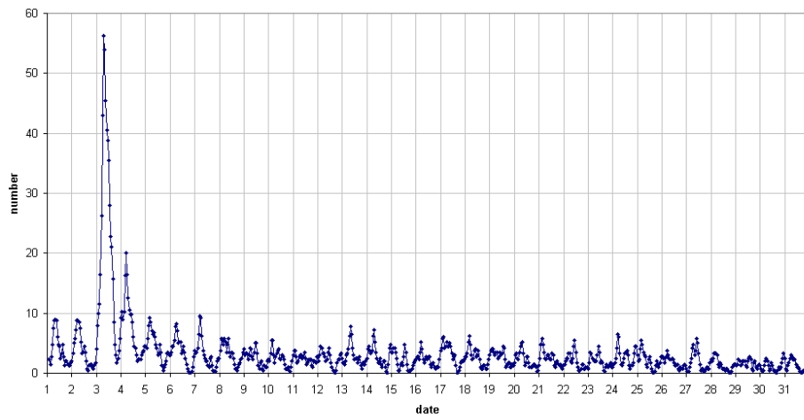
49.99MHz - RadioMeteors January 2017 number of overdense reflections per hour (weighted average) Felix Verbelen (Kampenhou)
