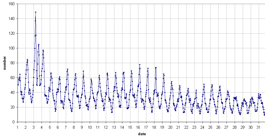
49.99 MHz - RadioMeteors January 2017 number of all reflections per hour (weighted average) (automatic count_Mette4_7Hz) Felix Verbelen (Kampenhou)
