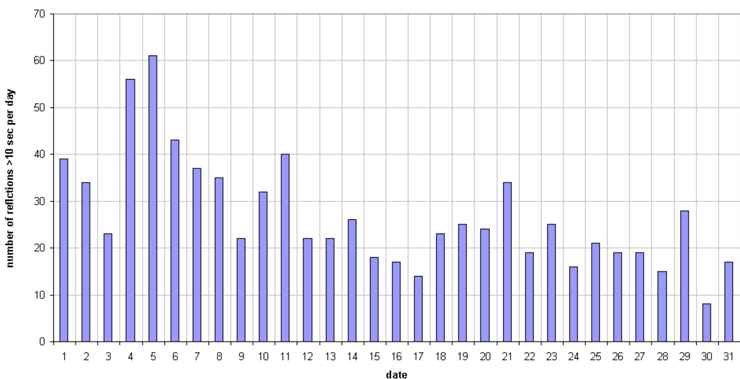
49.99MHz - RadioMeteors March 2017 daily totals of all overdense reflections Felix Verbelen (Kamphenhout)
