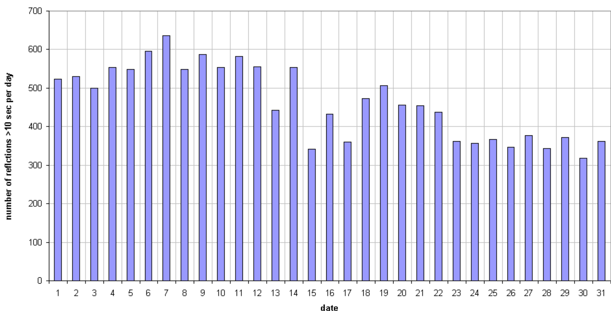
49.99MHz - RadioMeteors March 2017 daily totals of "all" reflections (automatic count_Mettel4_7Hz) Felix Verbelen (Kamphenhout)
