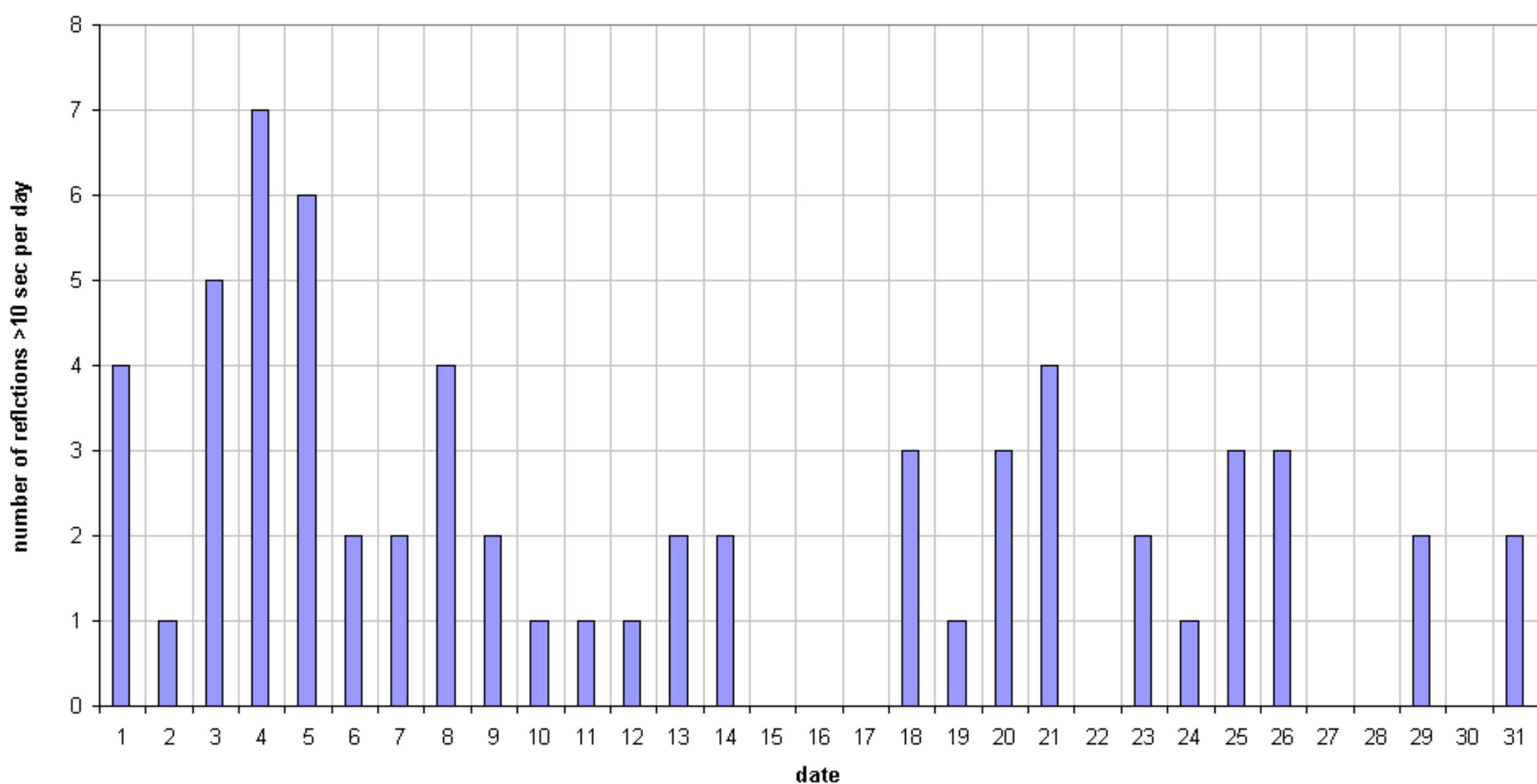
49.99MHz - RadioMeteors March 2017 daily totals of reflections longer than 10 seconds Felix Verbelen (Kamphenhout)
