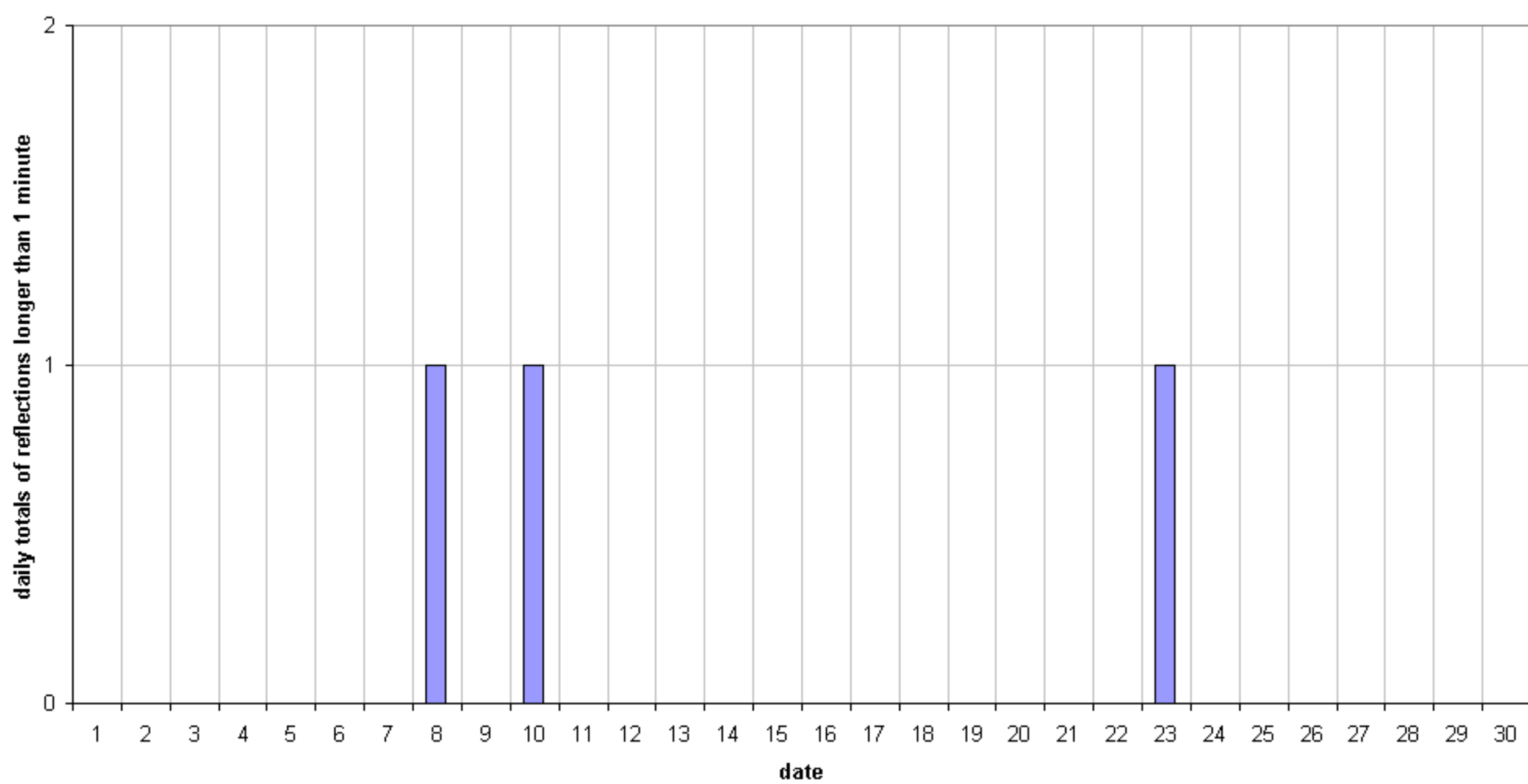
49.99MHz - RadioMeteors April 2017 daily totals of reflections longer than 1 minute Felix Verbelen (Kampenhout)
