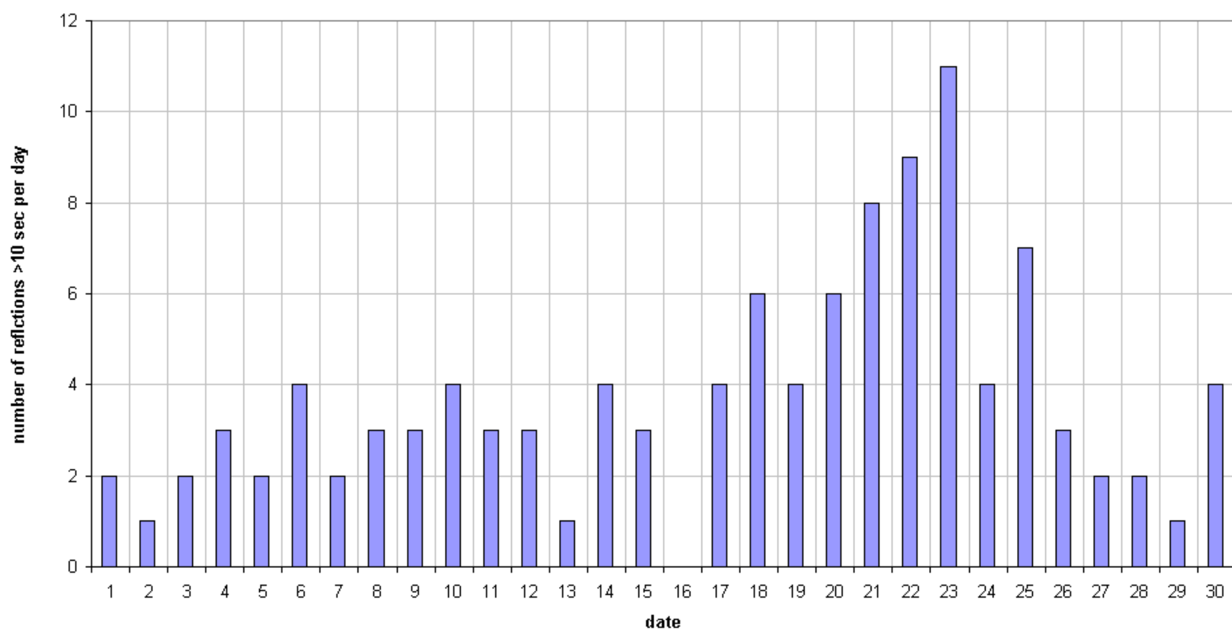
49.99MHz - RadioMeteors April 2017 daily totals of reflections longer than 10 seconds Felix Verbelen (Kampenhout)
