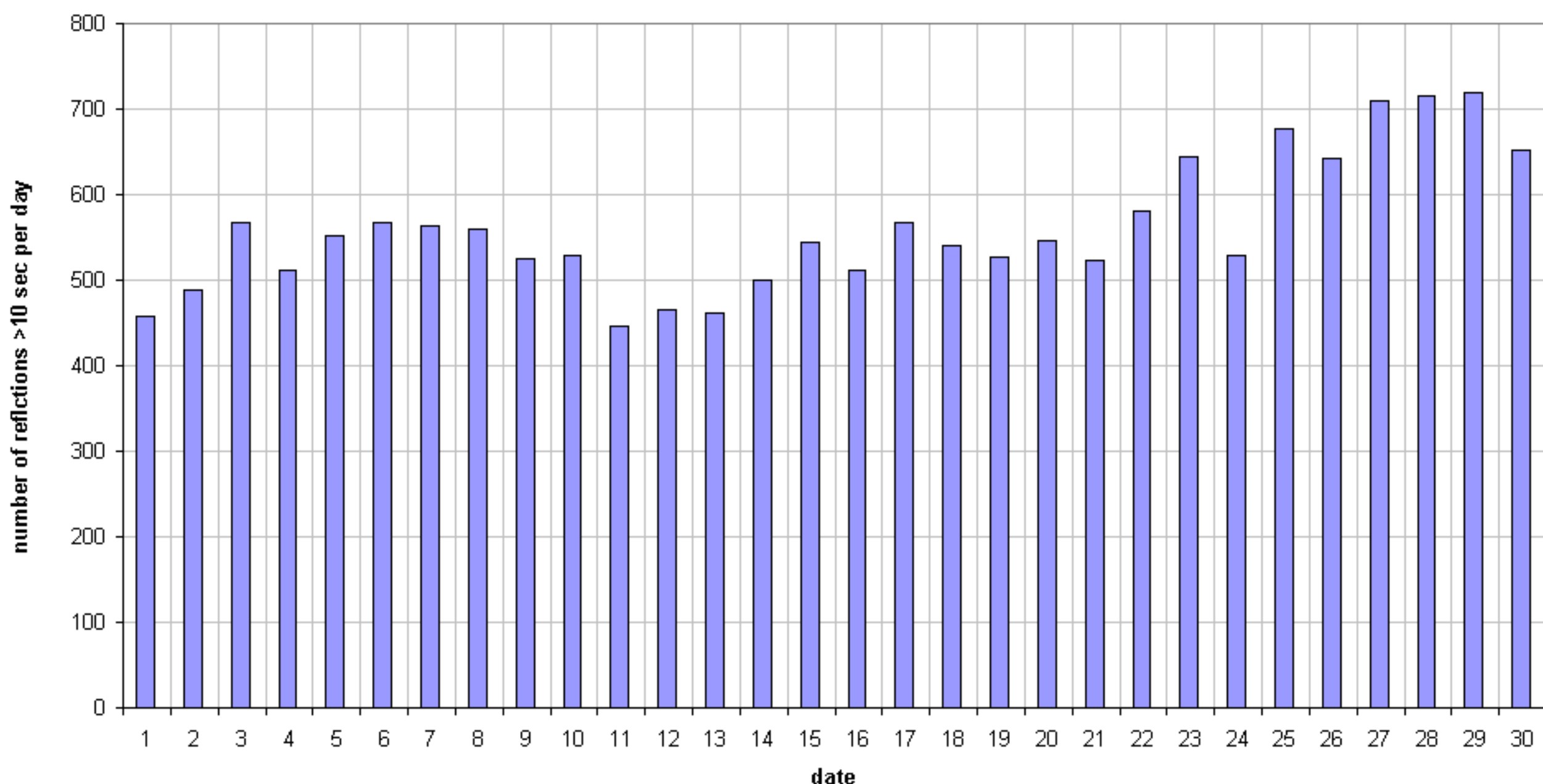
49.99MHz - RadioMeteors April 2017 daily totals of "all" reflections (automatic count_Mette4_7Hz) Felix Verbelen (Kampenhout)
