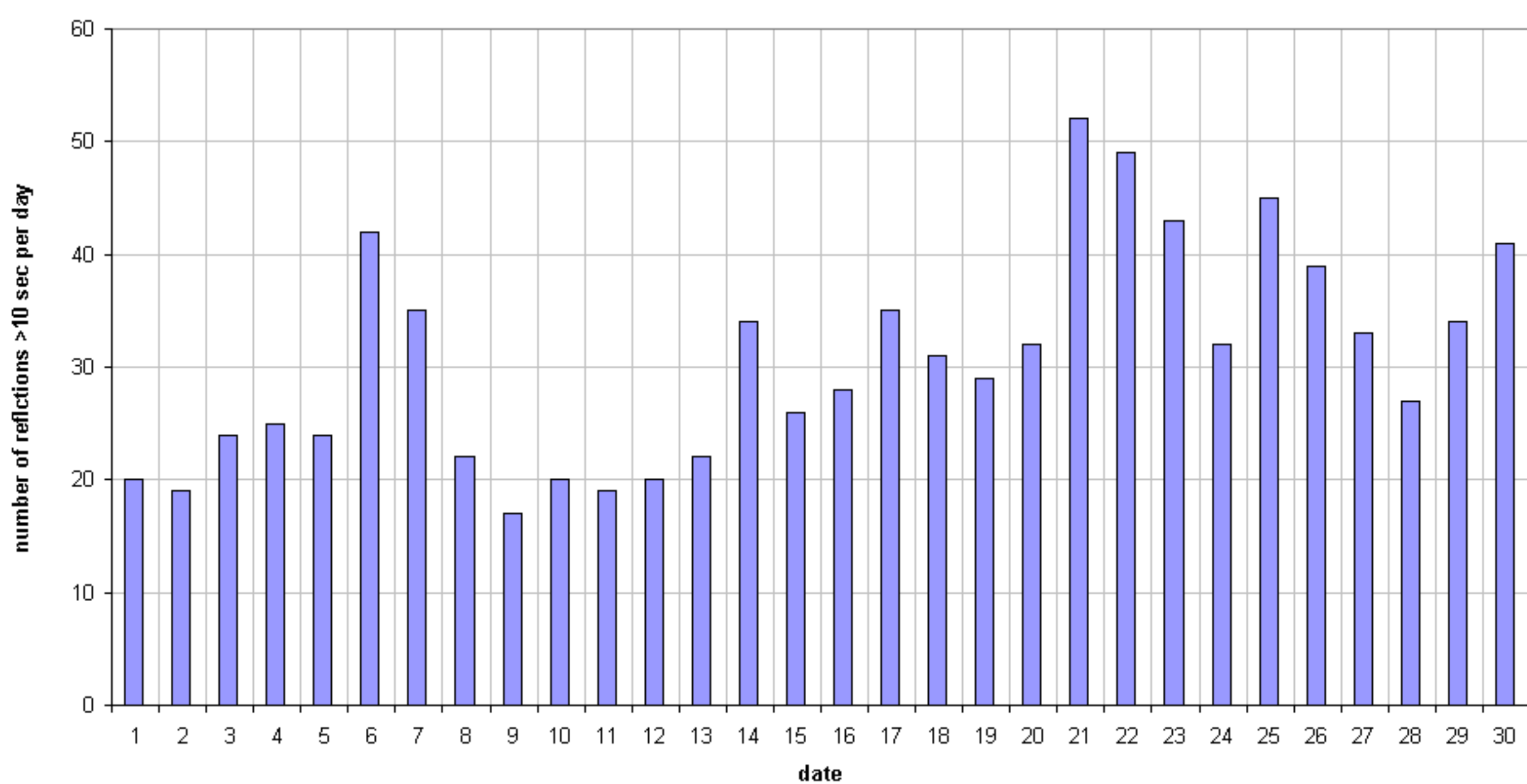
49.99MHz - RadioMeteors April 2017 daily totals of all overdense reflections Felix Verbelen (Kampenhout)
