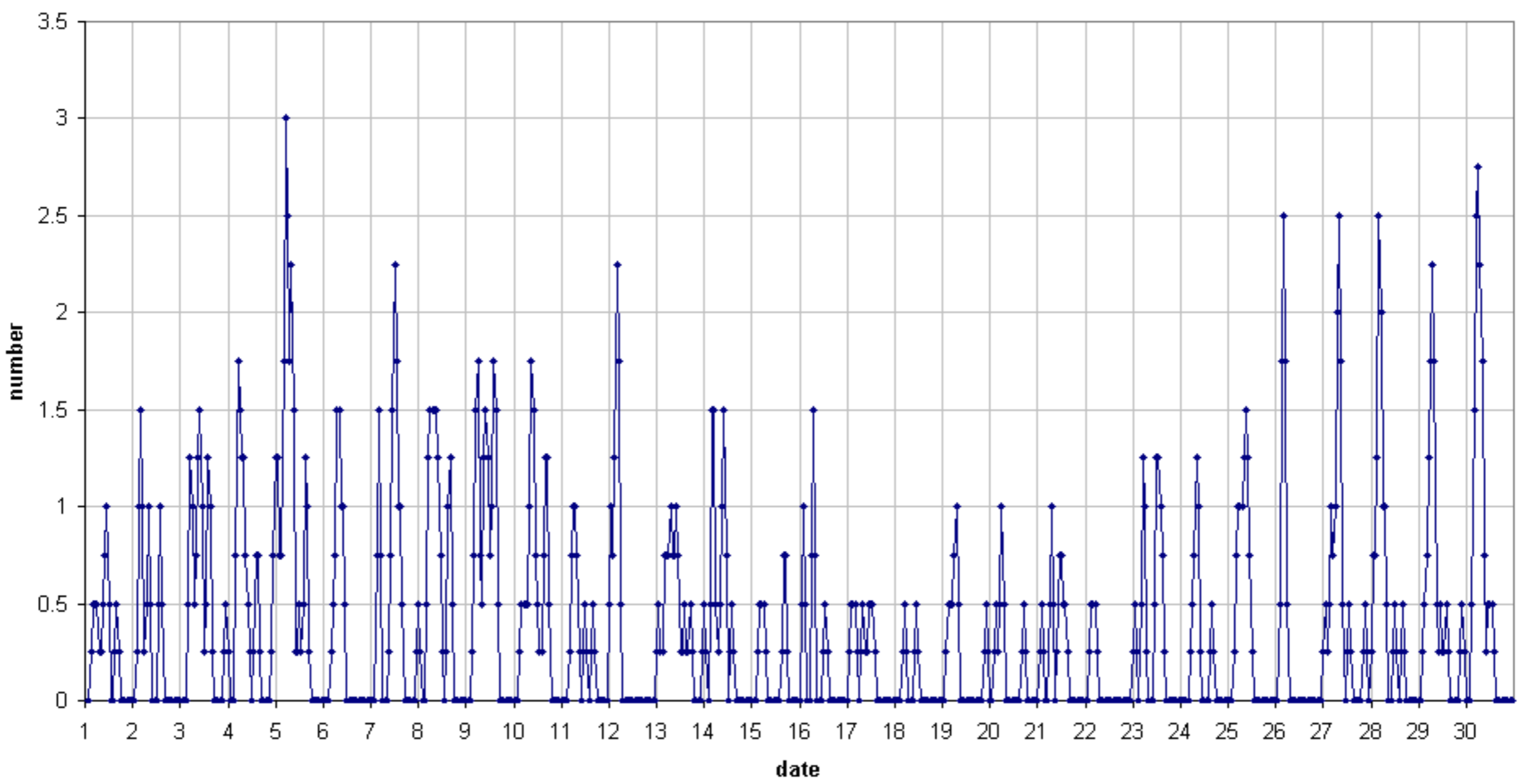
49.99MHz - RadioMeteors June 2017 number of reflections >10 seconds per hour (weighted average) Felix Verbelen (Kamphenhout)
