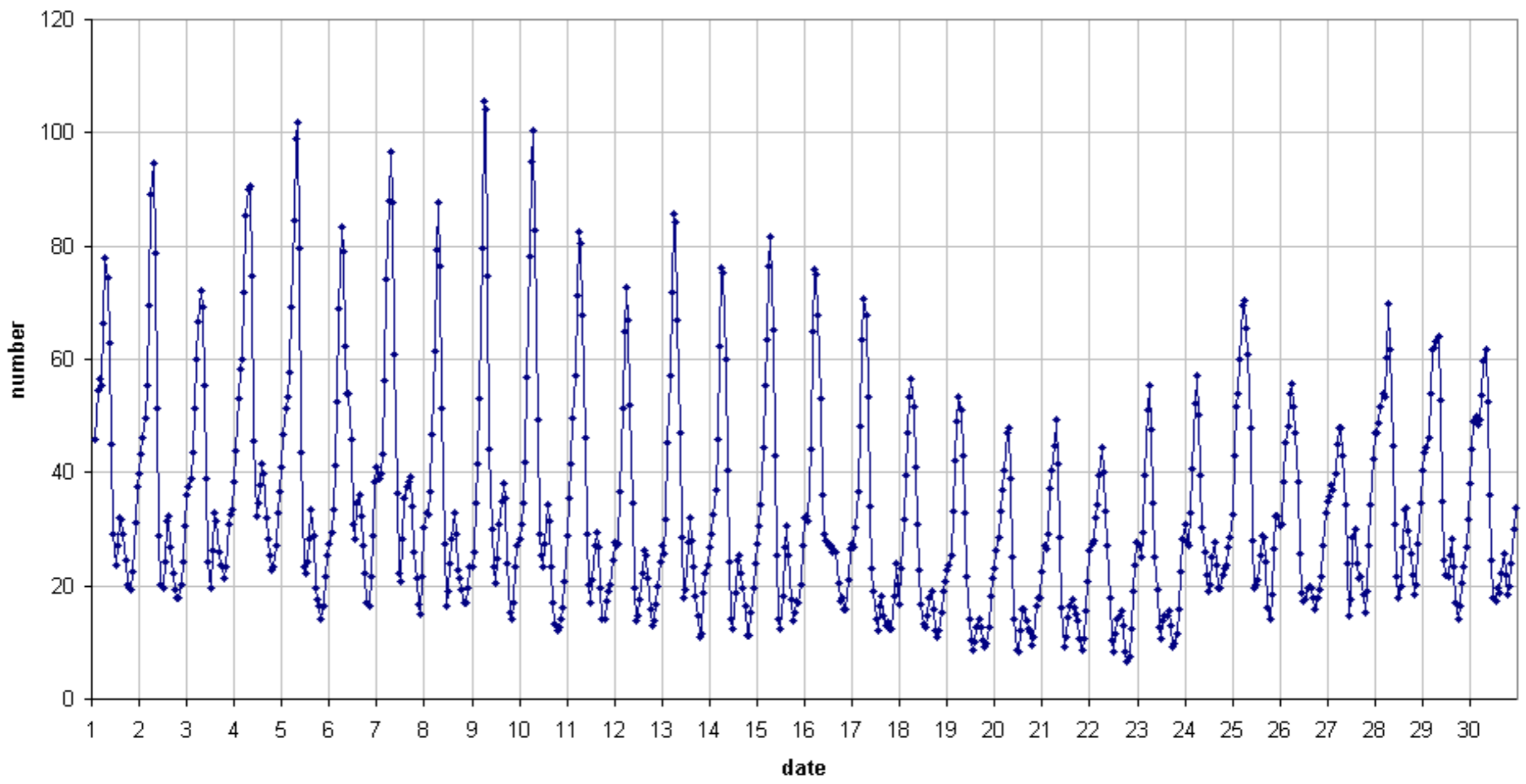
49.99 MHz - RadioMeteors June 2017 number of all reflections per hour (weighted average) (automatic count_Mette15_7Hz) Felix Verbelen (Kamphenhout)
