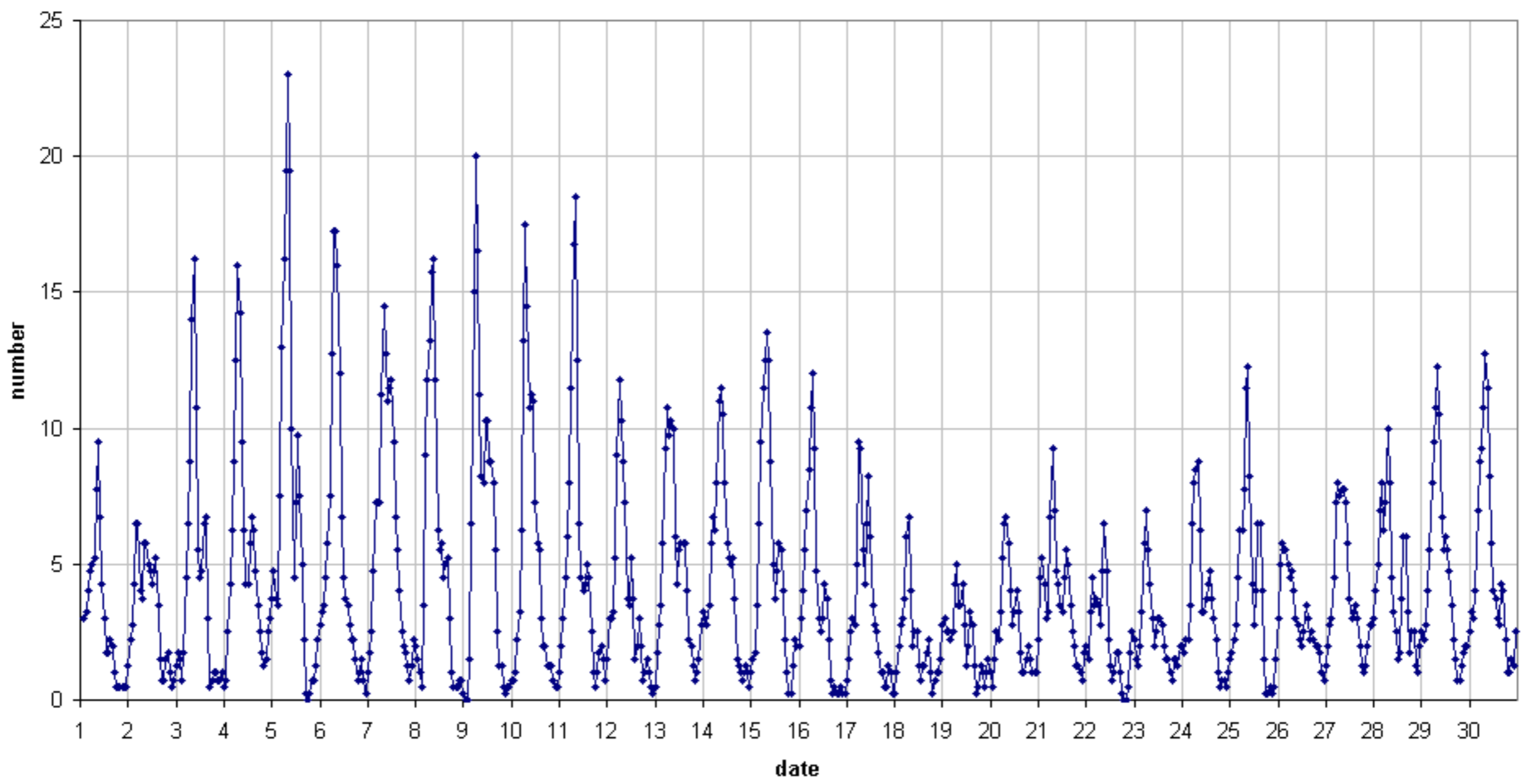
49.99MHz - RadioMeteors June 2017 number of overdense reflections per hour (weighted average) Felix Verbelen (Kamphenhout)
