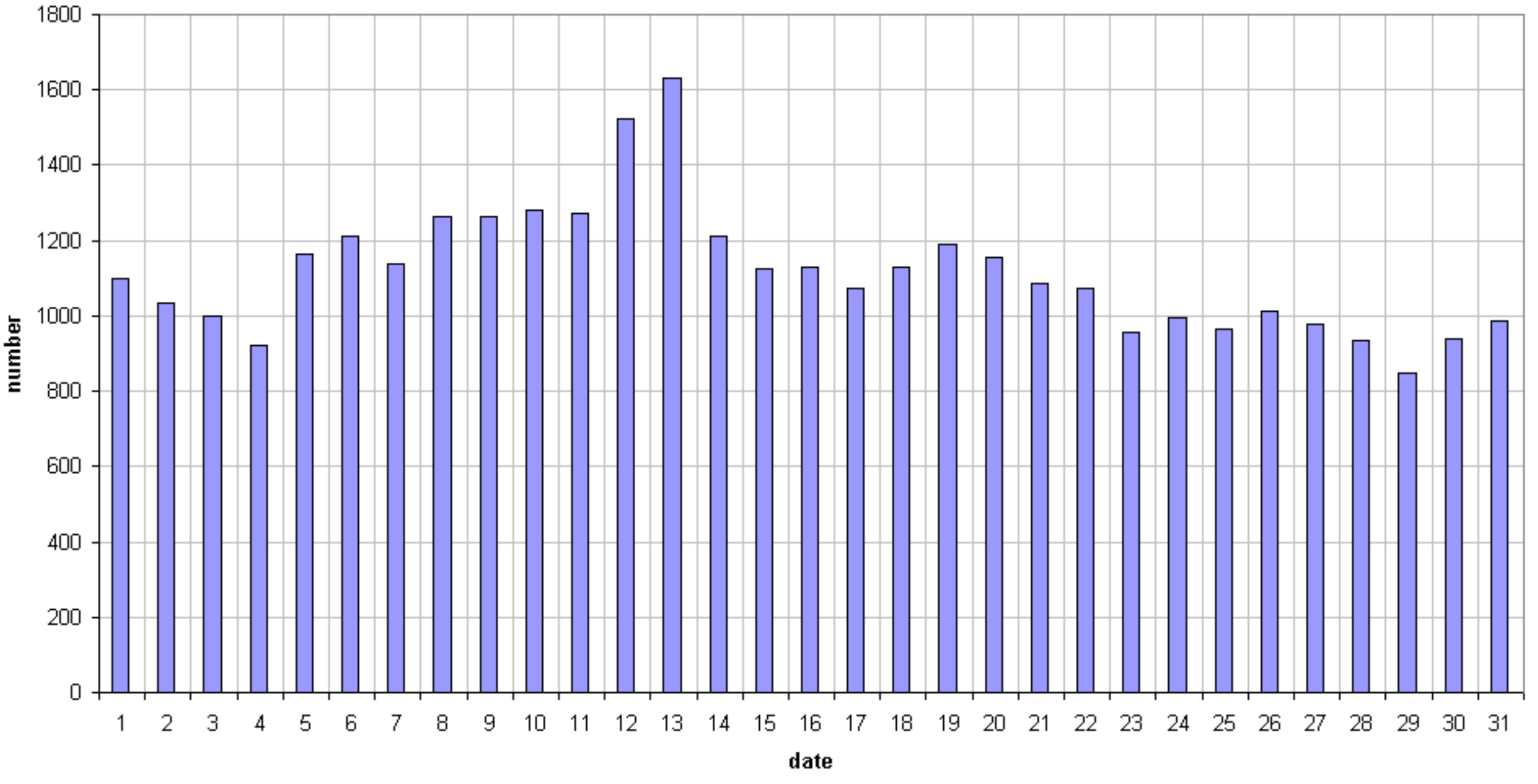
49.99MHz - RadioMeteors August 2017 daily totals of "all" reflections (automatic count_Mette15_7Hz) Felix Verbelen (Kamphenhout)
