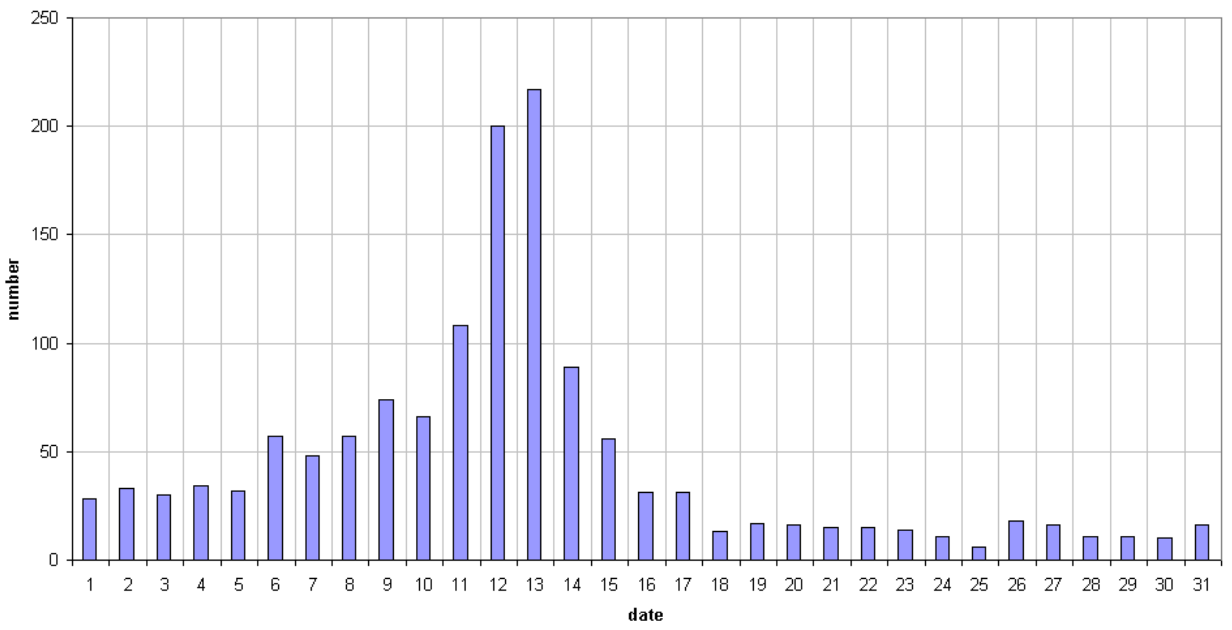
49.99MHz - RadioMeteors August 2017 daily totals of reflections longer than 10 seconds Felix Verbelen (Kamphenhout)
