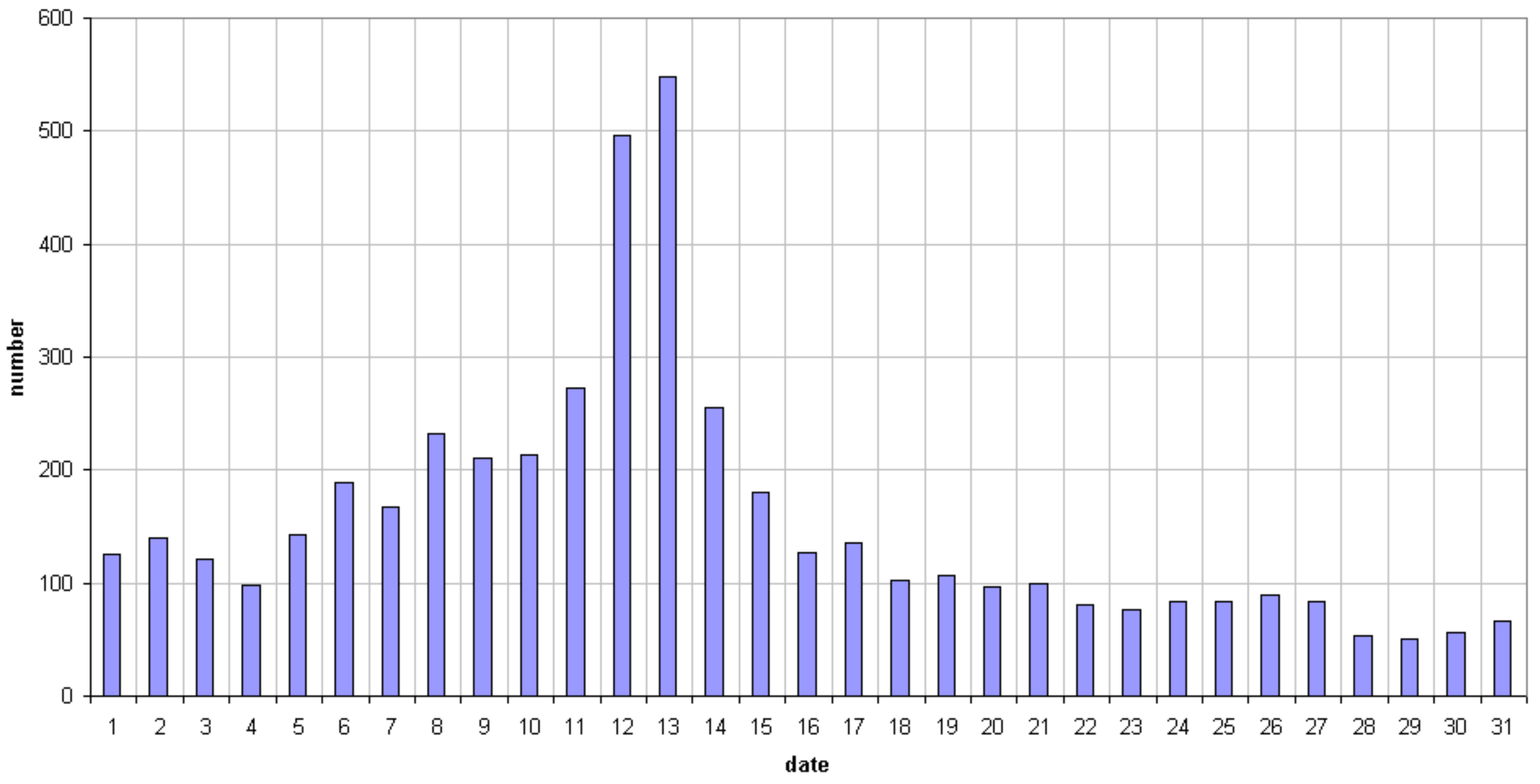
49.99MHz - RadioMeteors August 2017 daily totals of all overdense reflections Felix Verbelen (Kamphenhout)
