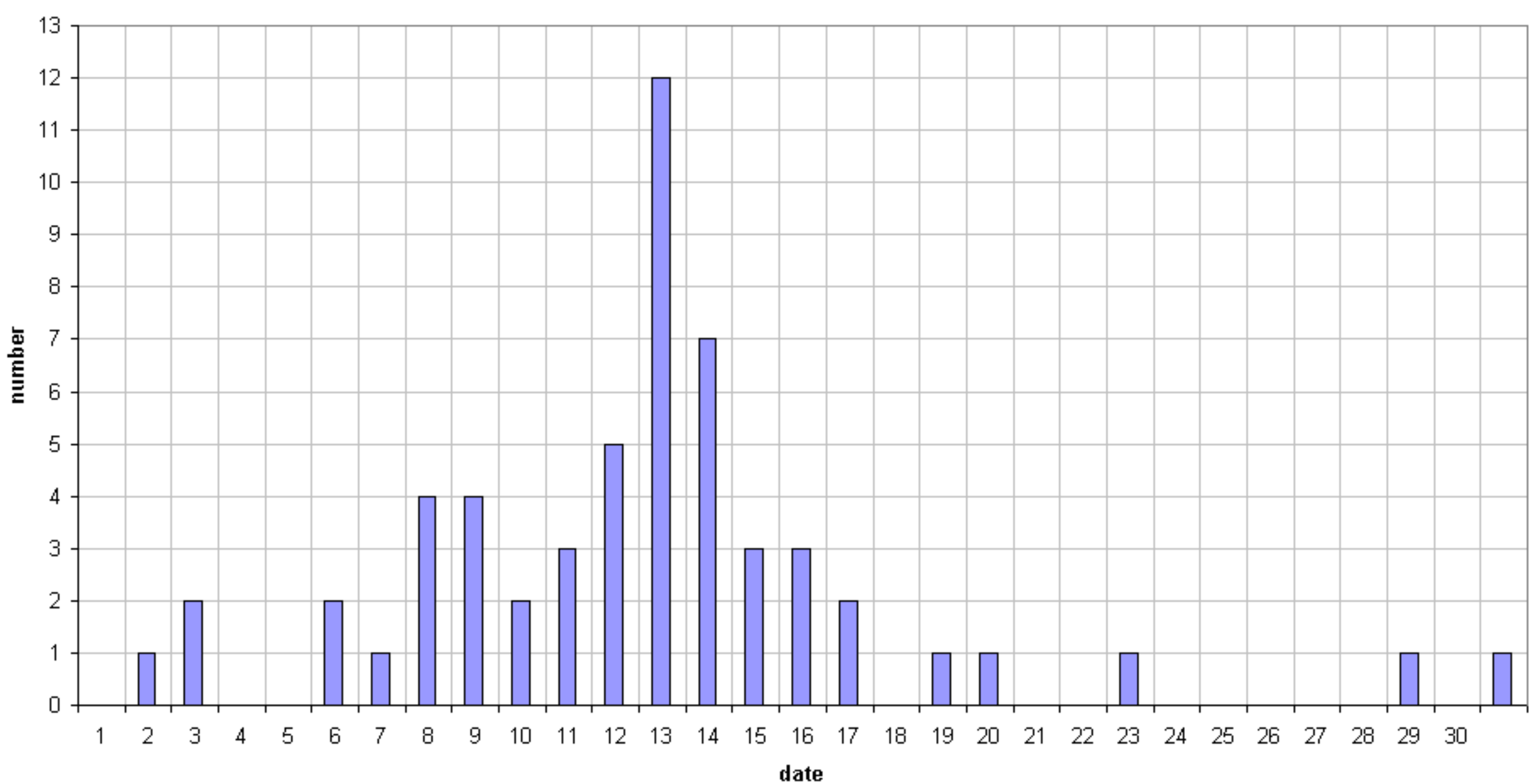
49.99MHz - RadioMeteors August 2017 daily totals of reflections longer than 1 minute Felix Verbelen (Kamphenhout)
