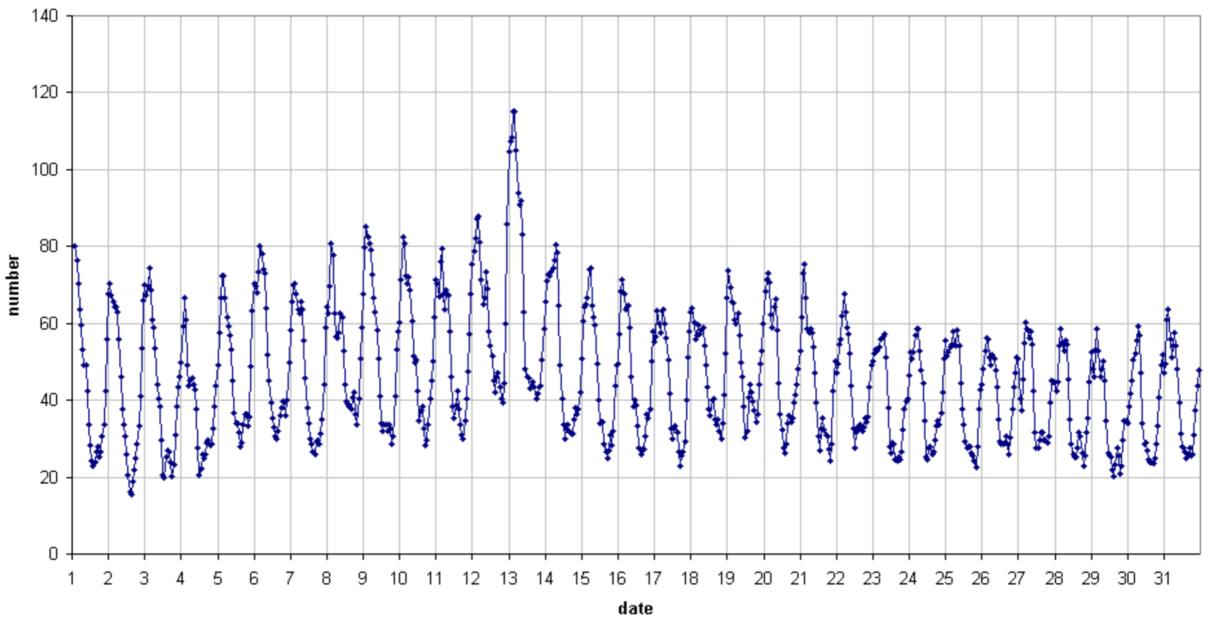
49.99 MHz - RadioMeteors August 2017 number of "all" reflections per hour (weighted average) (automatic count_Mettel5_7Hz) Felix Verbelen (Kampenhout)
