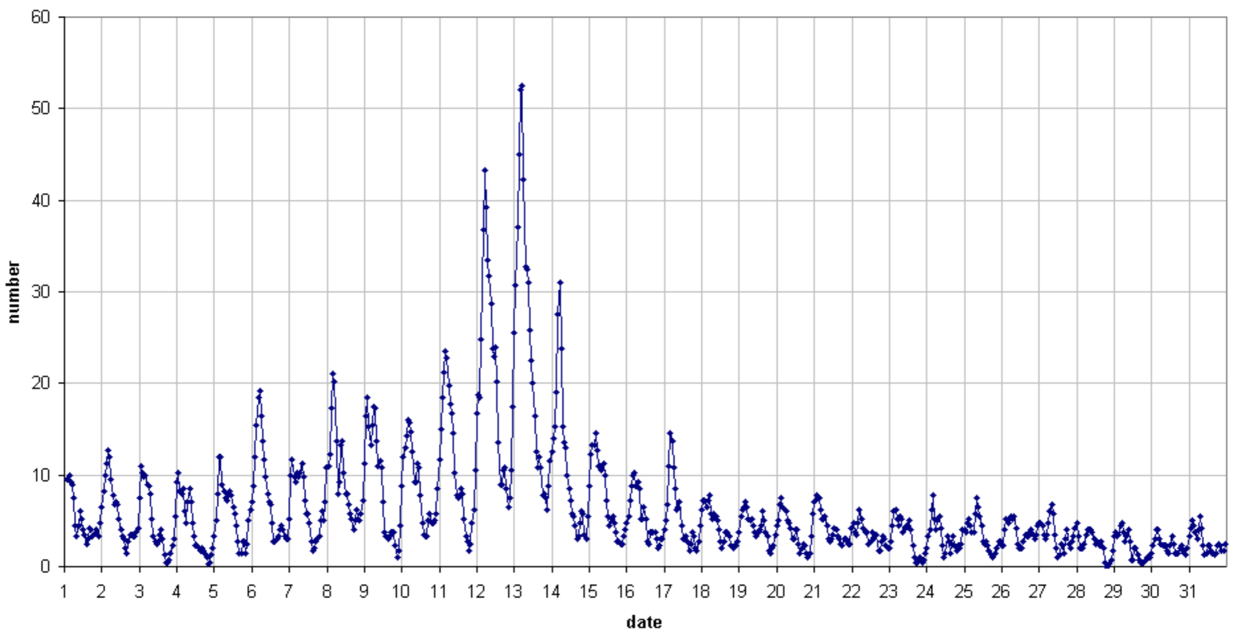
49.99MHz - RadioMeteors August 2017 number of overdense reflections per hour (weighted average) Felix Verbelen (Kampenhout)
