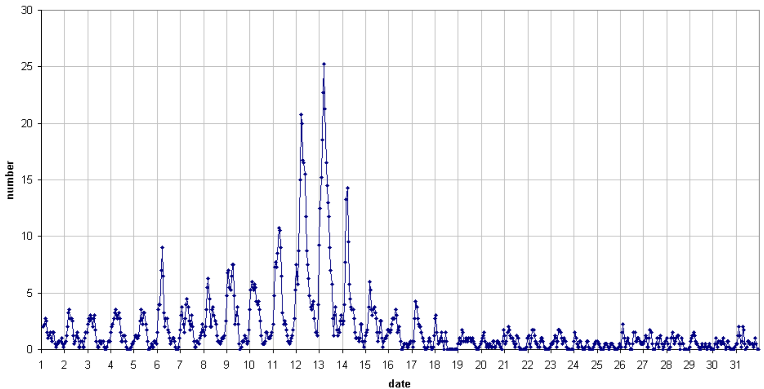
49.99MHz - RadioMeteors August 2017 number of reflections >10 seconds per hour (weighted average) Felix Verbelen (Kampenhout)
