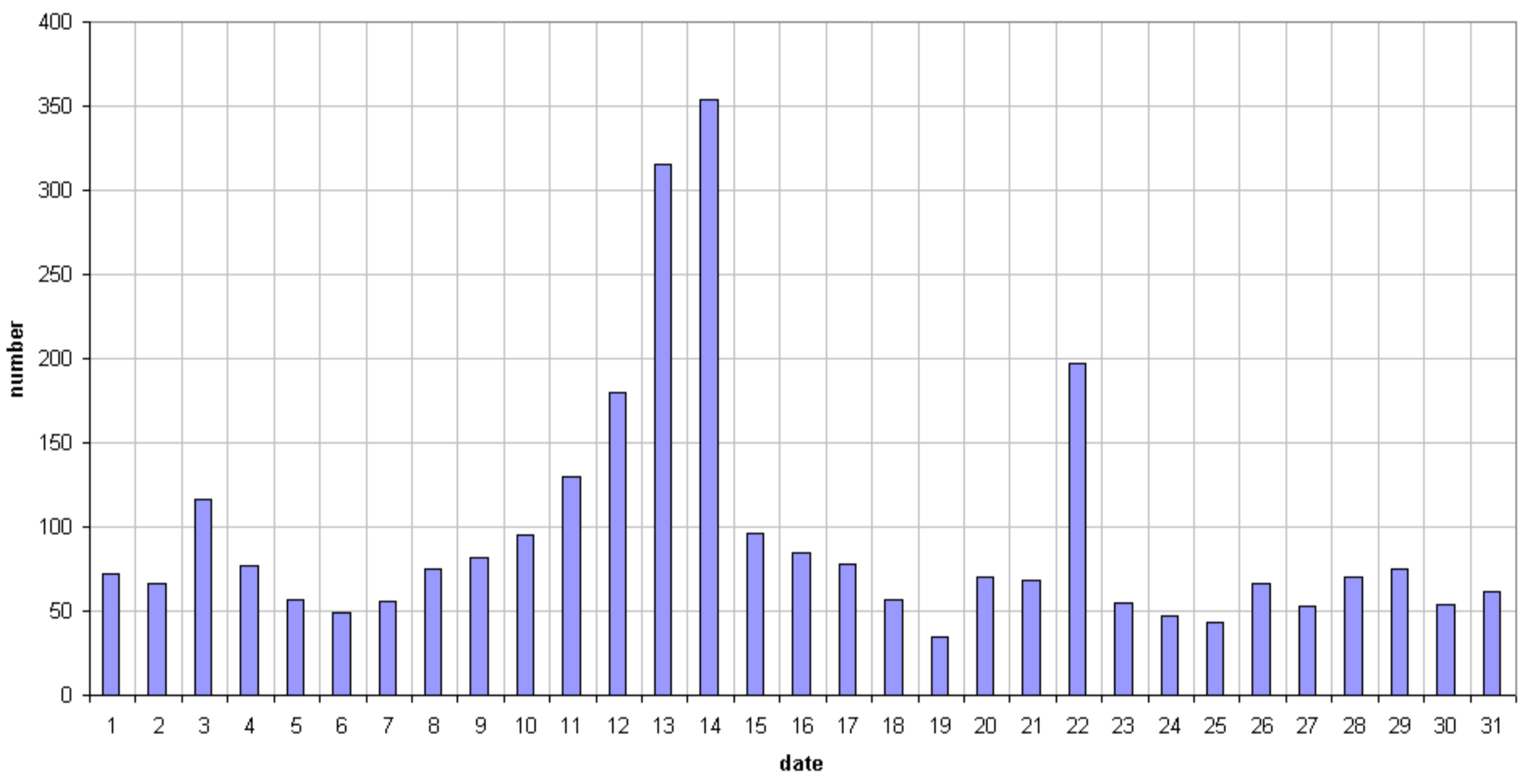
49.99MHz - Radiometeors December 2017 daily totals of all overdense reflections Felix Verbelen (Kampenhout)
