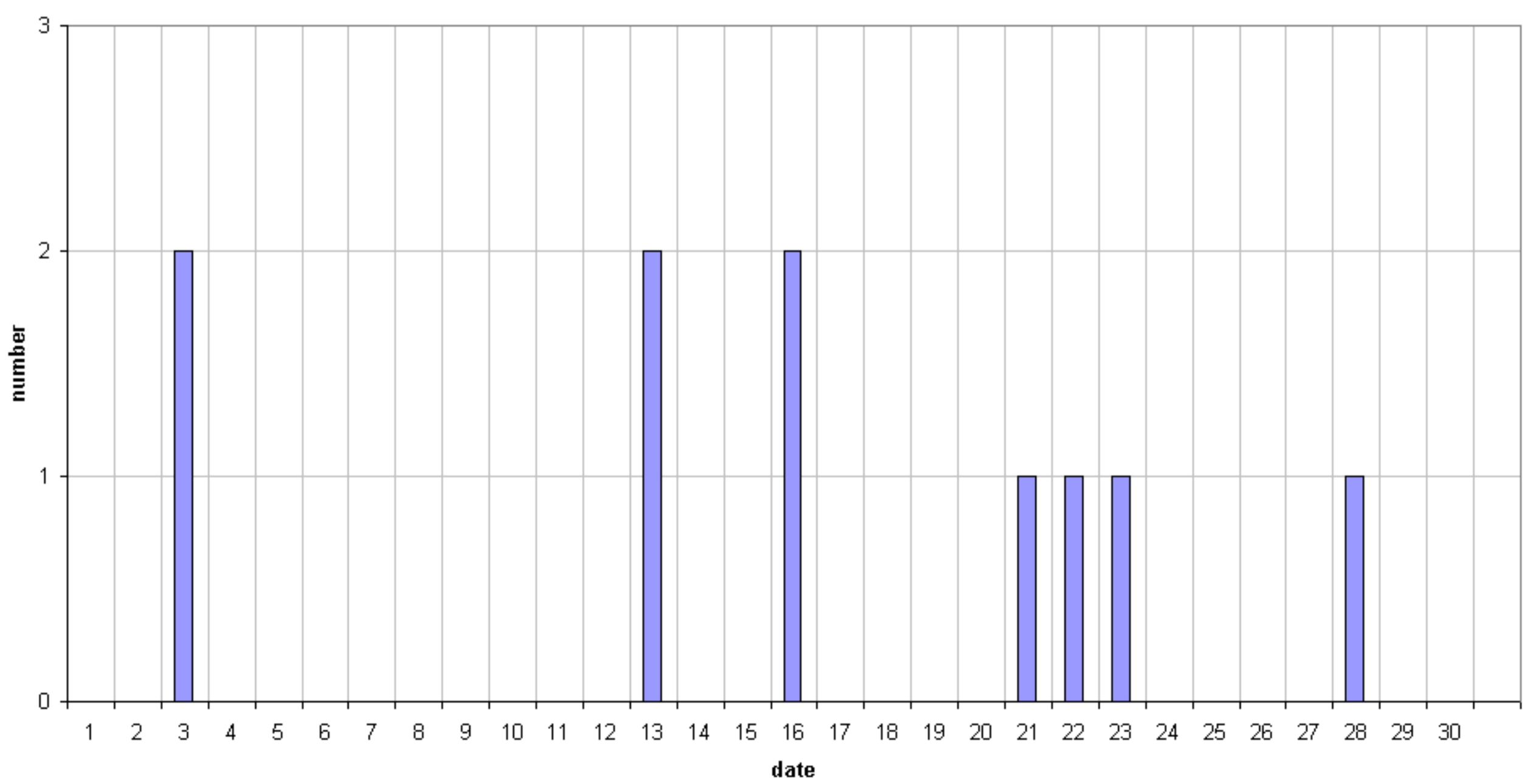
49.99MHz - Radiometeors December 2017 daily totals of reflections longer than 1 minute Felix Verbelen (Kampenhout)
