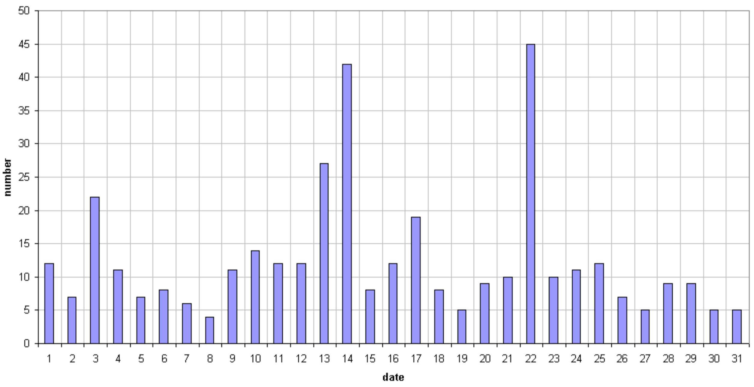
49.99MHz - Radiometeors December 2017 daily totals of reflections longer than 10 seconds Felix Verbelen (Kampenhout)
