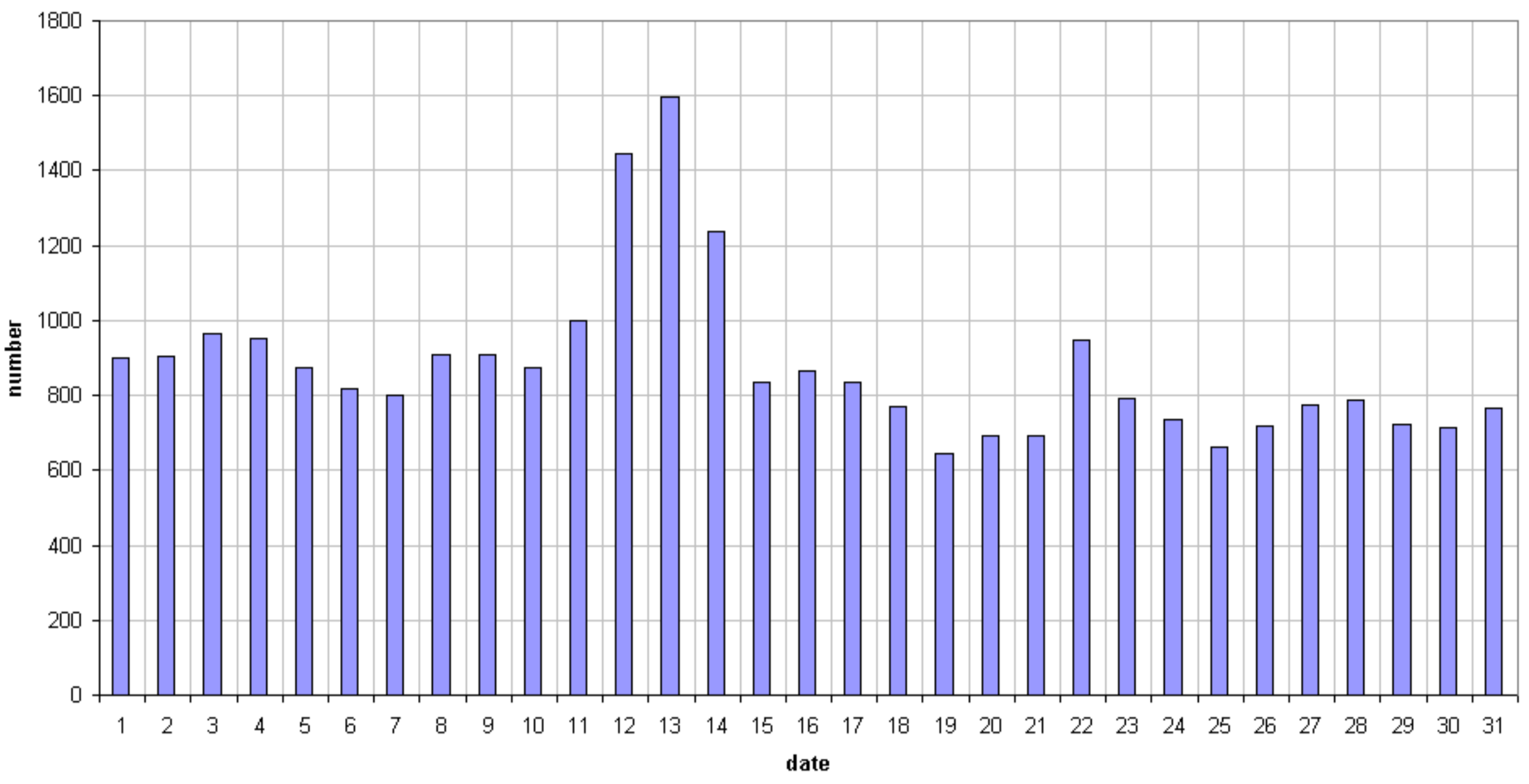
49.99MHz - Radiometeors December 2017 daily totals of "all" reflections (automatic count_Mette15_7Hz) Felix Verbelen (Kampenhout)
