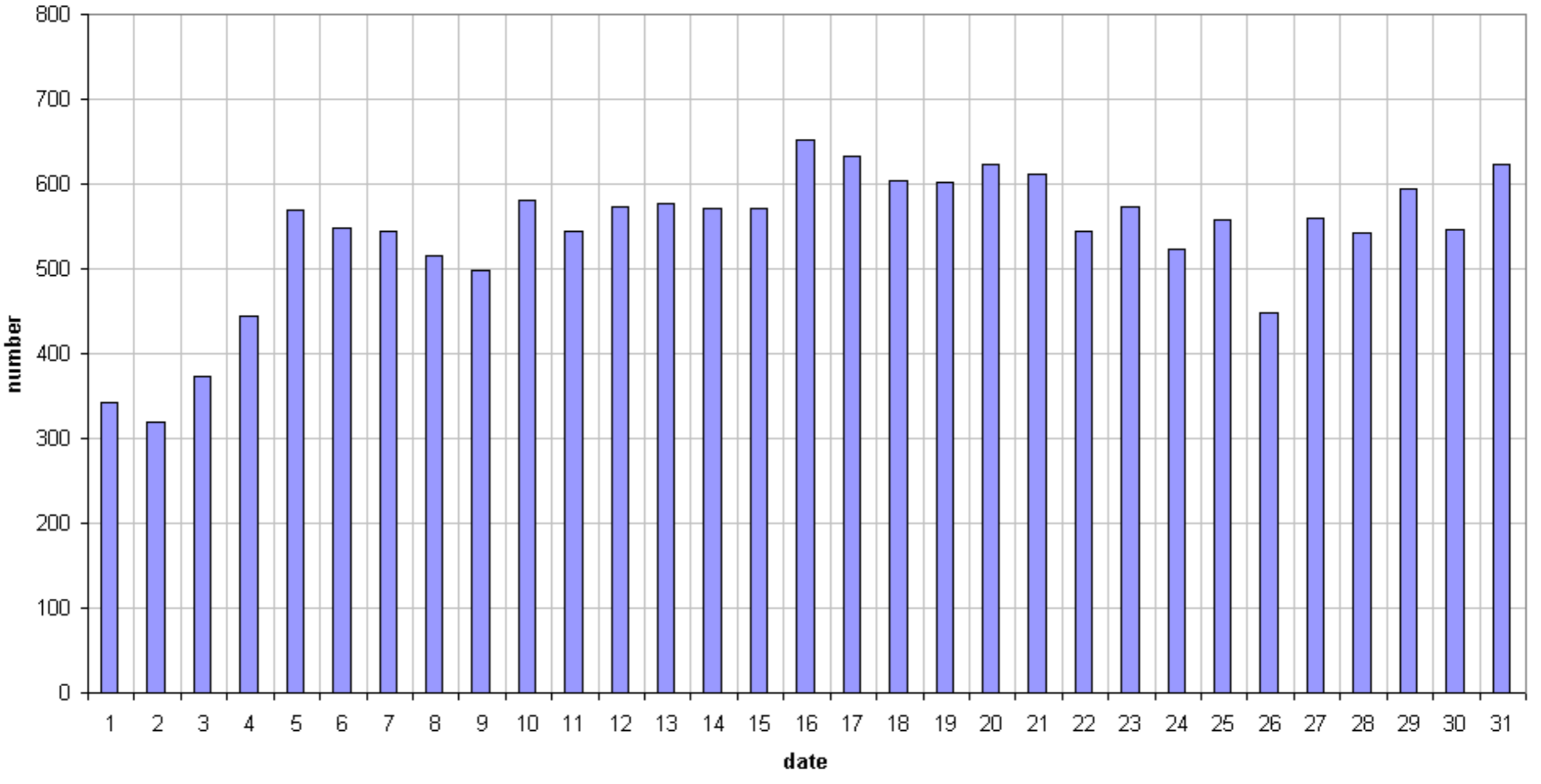
49.99MHz - RadioMeteors March 2018 daily totals of "all" reflections (automatic count_Mette15_7Hz) Felix Verbelen (Kampenhout)
