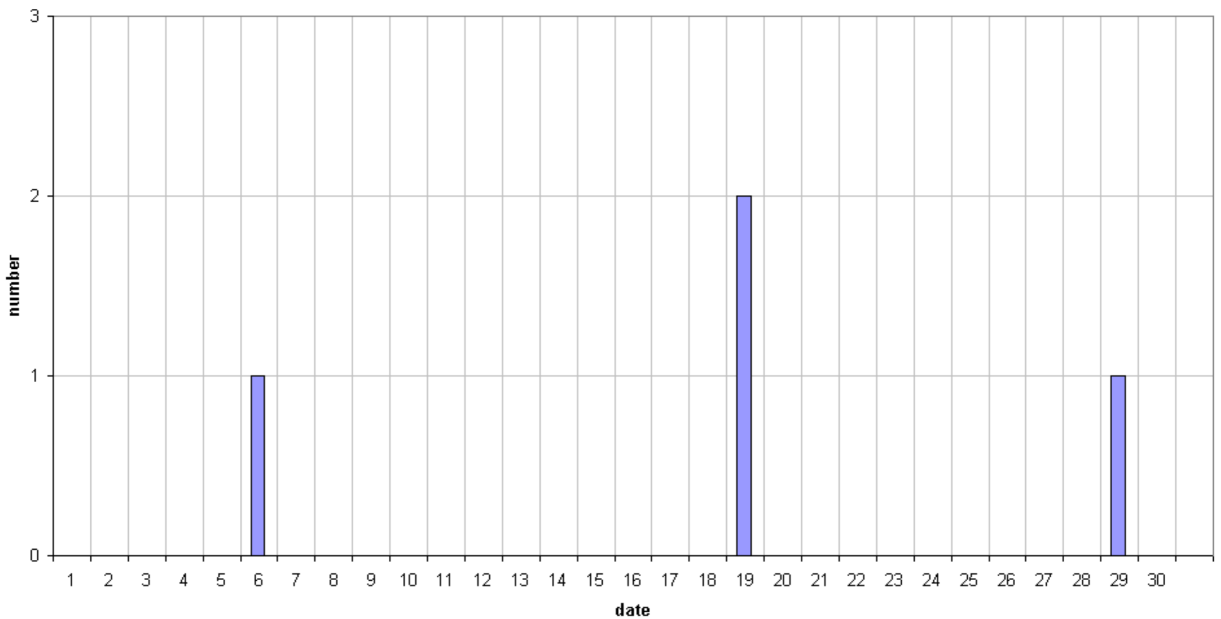
49.99MHz - RadioMeteors March 2018 daily totals of reflections longer than 1 minute Felix Verbelen (Kampenhout)
