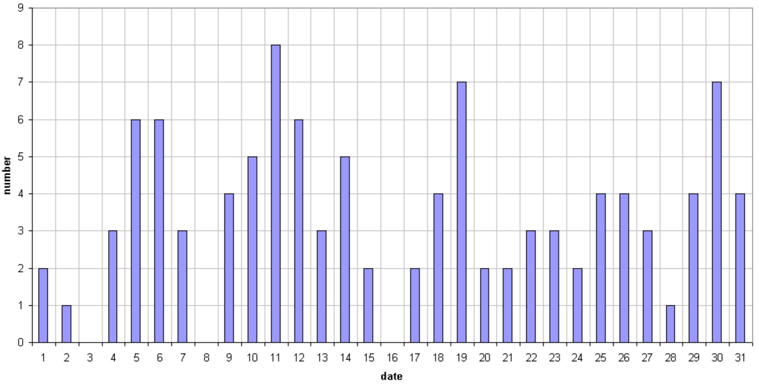
49.99MHz - RadioMeteors March 2018 daily totals of reflections longer than 10 seconds Felix Verbelen (Kampenhout)
