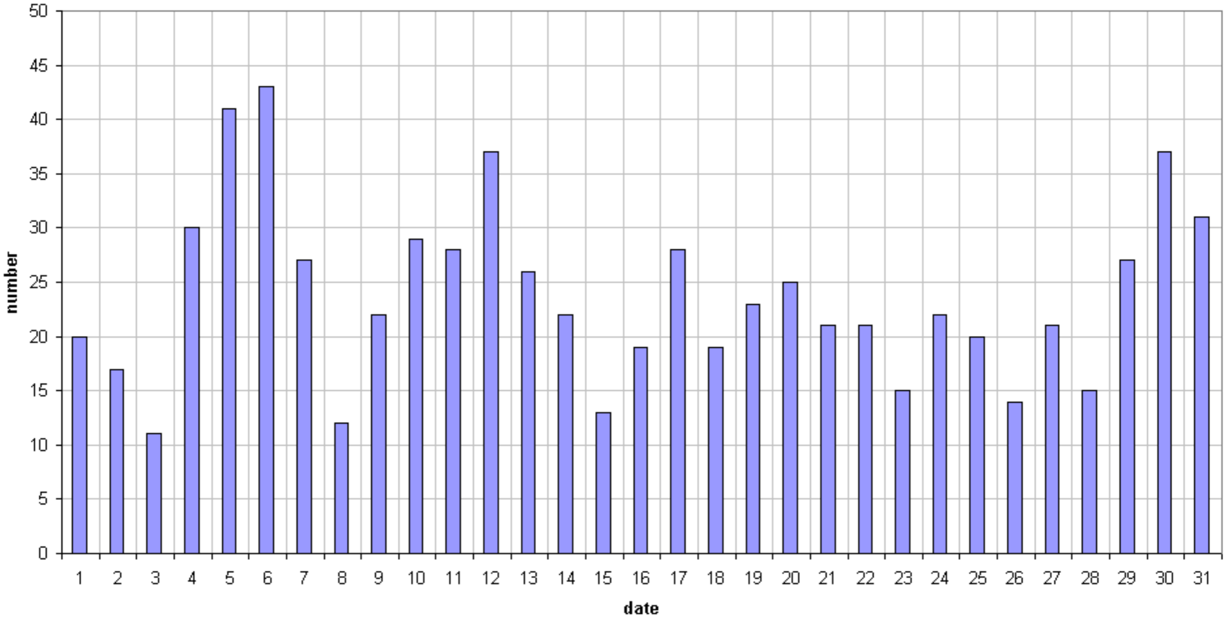
49.99MHz - RadioMeteors March 2018 daily totals of all overdense reflections Felix Verbelen (Kampenhout)
