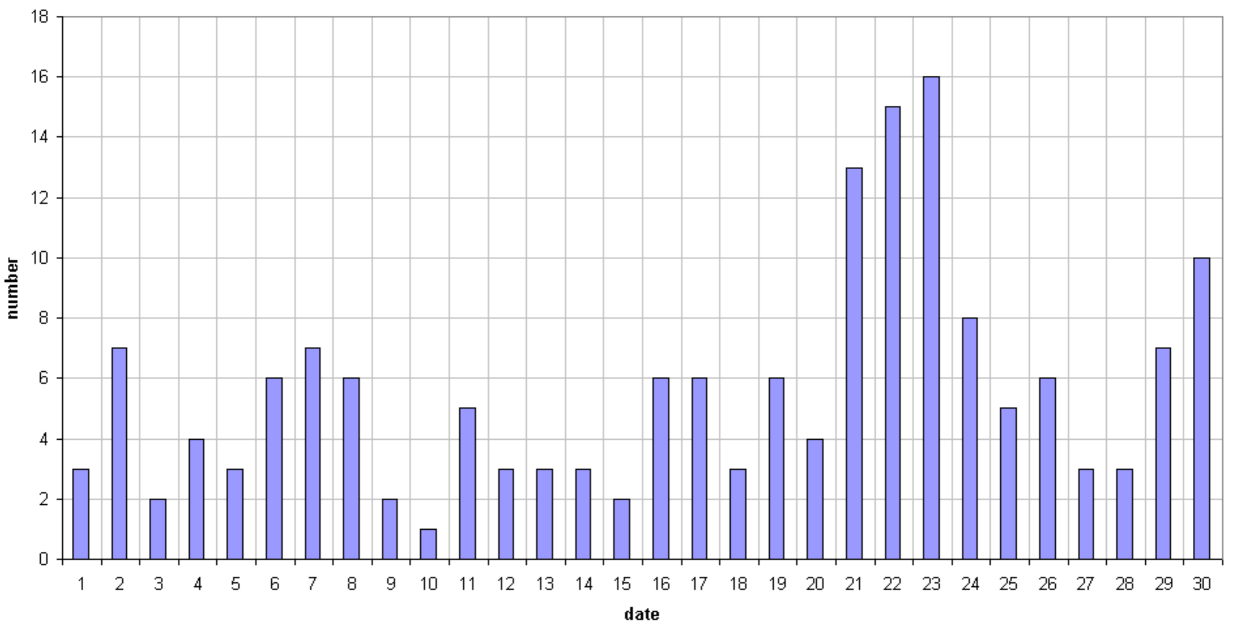
49.99MHz - RadioMeteors April 2018 daily totals of reflections longer than 10 seconds Felix Verbelen (Kampenhout)
