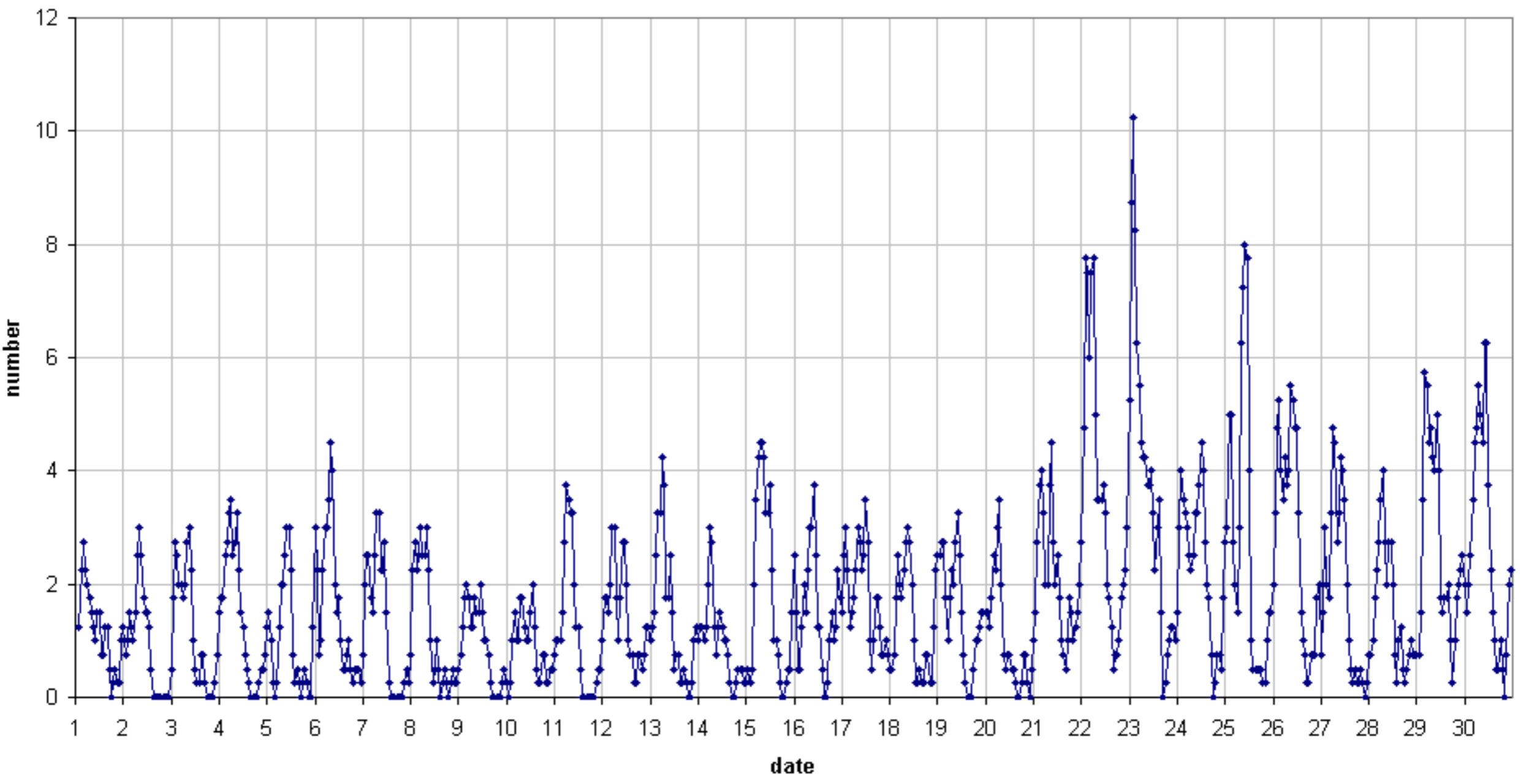
49.99MHz - RadioMeteors April 2018 number of overdense reflections per hour (weighted average) Felix Verbelen (Kampenhout)
