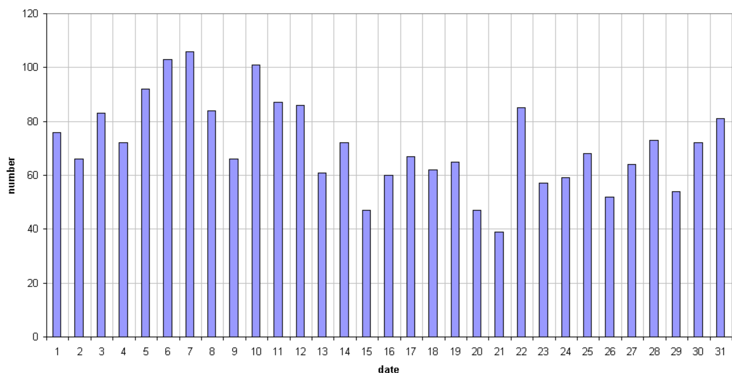
49.99MHz - RadioMeteors May 2018 daily totals of all overdense reflections Felix Verbelen (Kampenhout)
