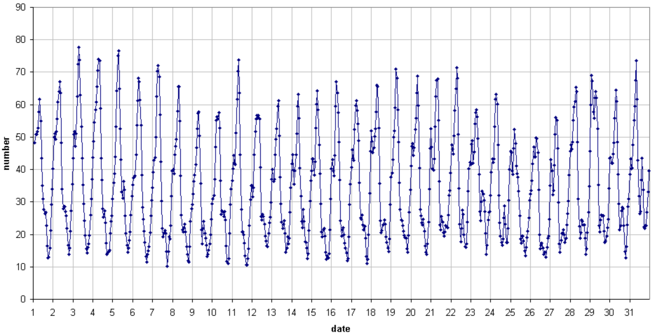
49.99 MHz - RadioMeteors May 2018 number of "all" reflections per hour (weighted average) (automatic count_Mette15_7Hz) Felix Verbelen (Kamphenhout)
