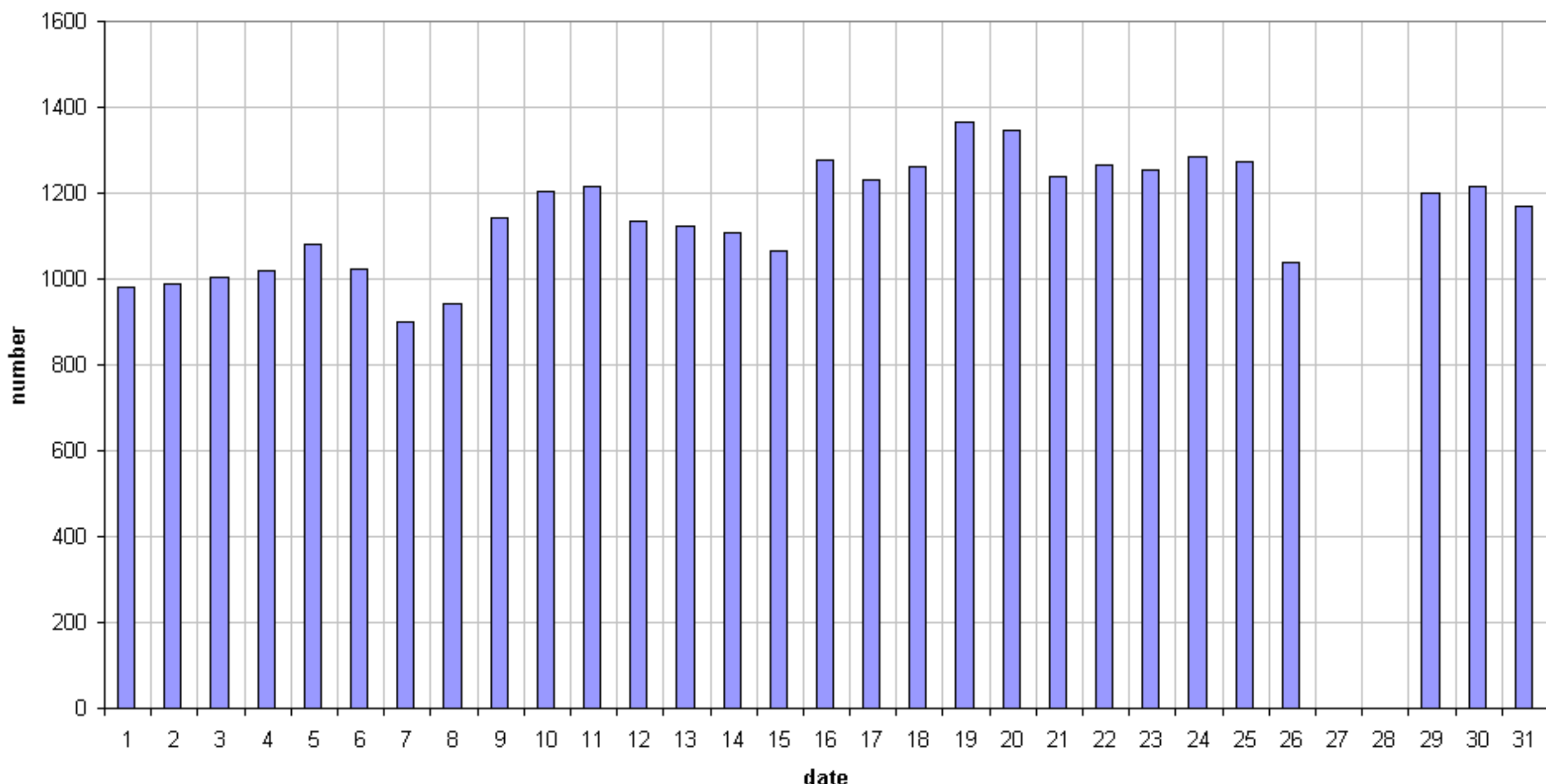
49.99MHz - RadioMeteors July 2018 daily totals of "all" reflections (automatic count_Mette15_7Hz) Felix Verbelen (Kampenhout)
