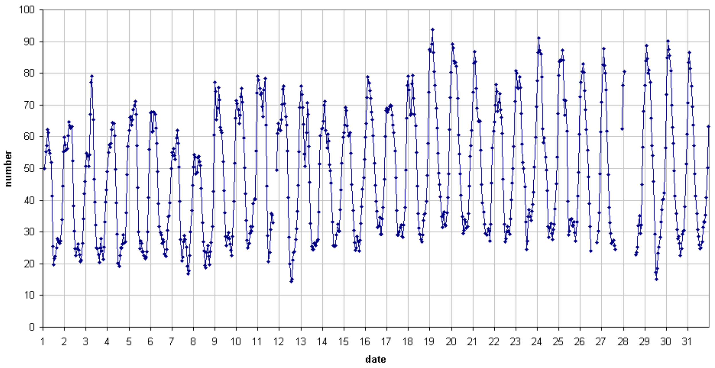
49.99 MHz - RadioMeteors July 2018 number of "all" reflections per hour (weighted average) (automatic count_Mette15_7Hz) Felix Verbelen (Kampenhout)
