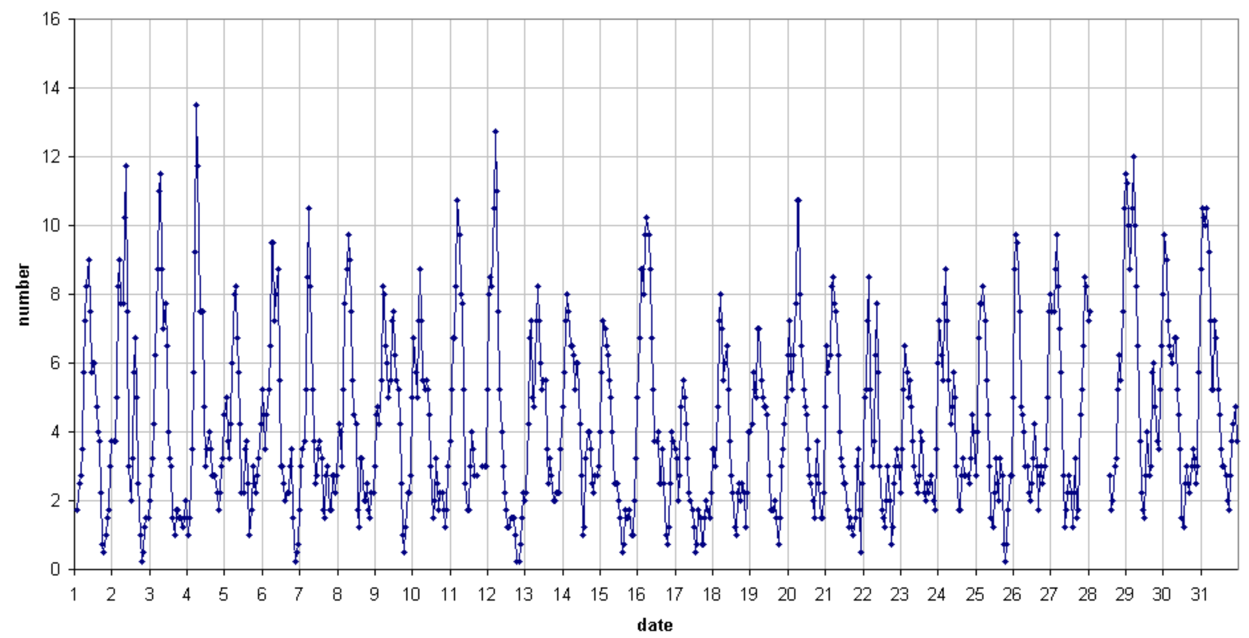
49.99MHz - RadioMeteors July 2018 number of overdense reflections per hour (weighted average) Felix Verbelen (Kampenhout)
