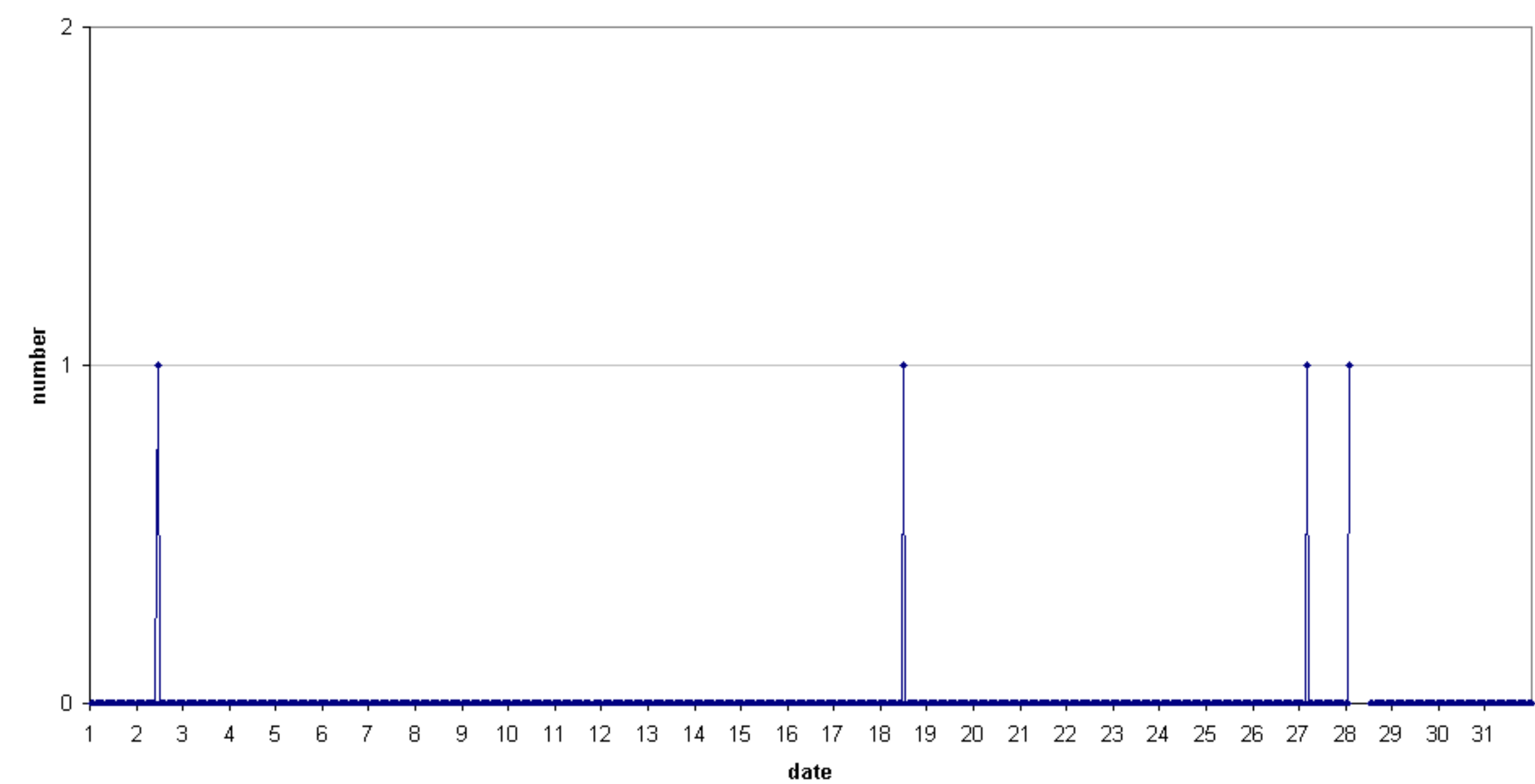
49.99MHz - RadioMeteors July 2018 hourly totals of overdense reflections longer than 1 minute Felix Verbelen (Kampenhout/BE)
