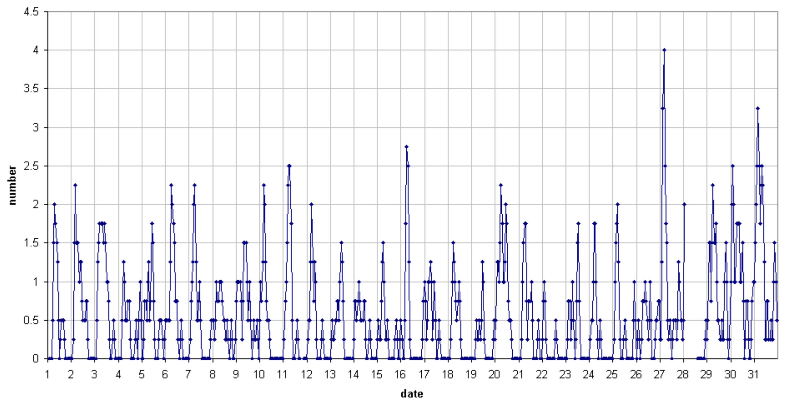
49.99MHz - RadioMeteors July 2018 number of reflections >10 seconds per hour (weighted average) Felix Verbelen (Kampenhout)
