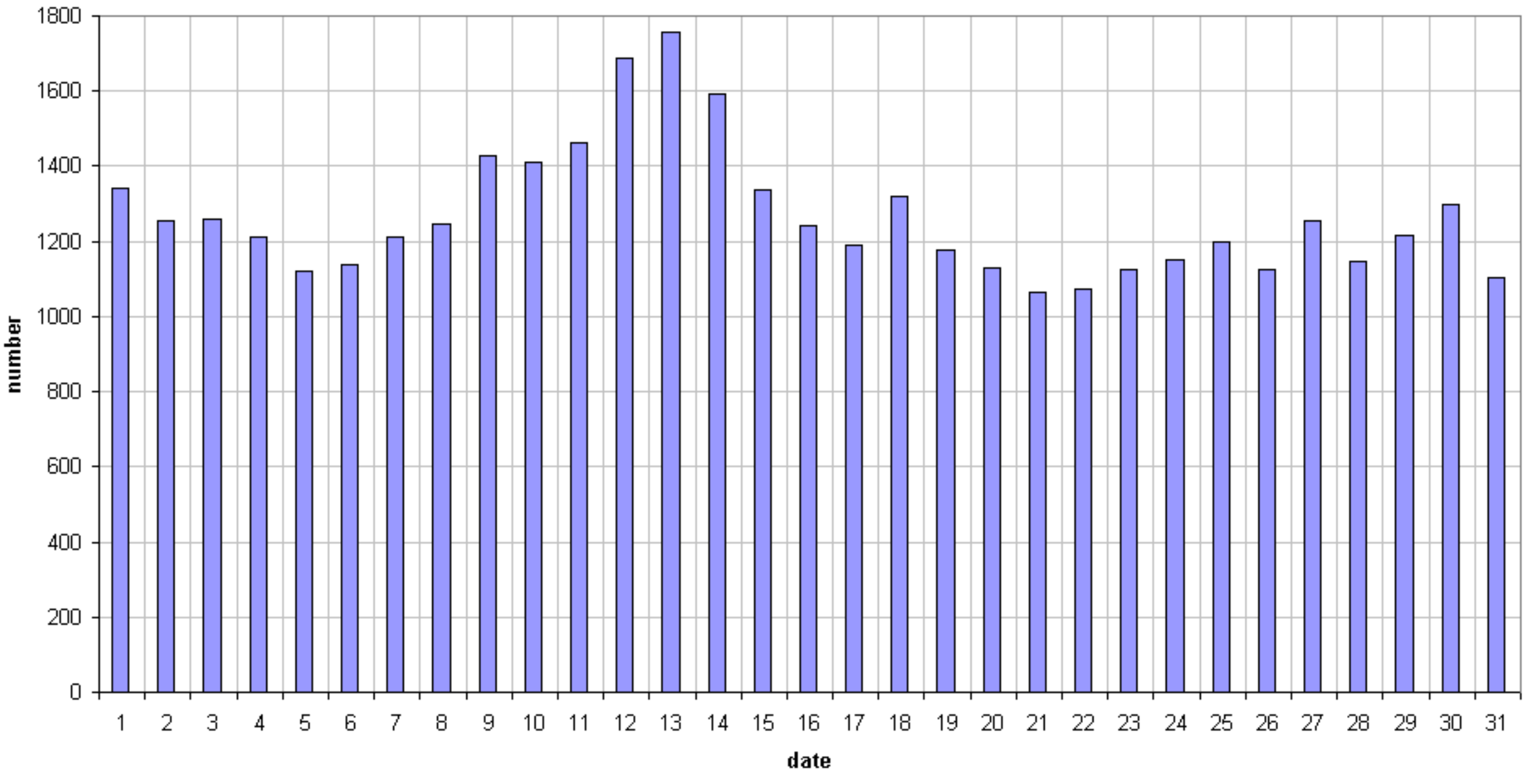
49.99MHz - RadioMeteors August 2018 daily totals of "all" reflections (automatic count_Mette15_7Hz) Felix Verbelen (Kampenhout)
