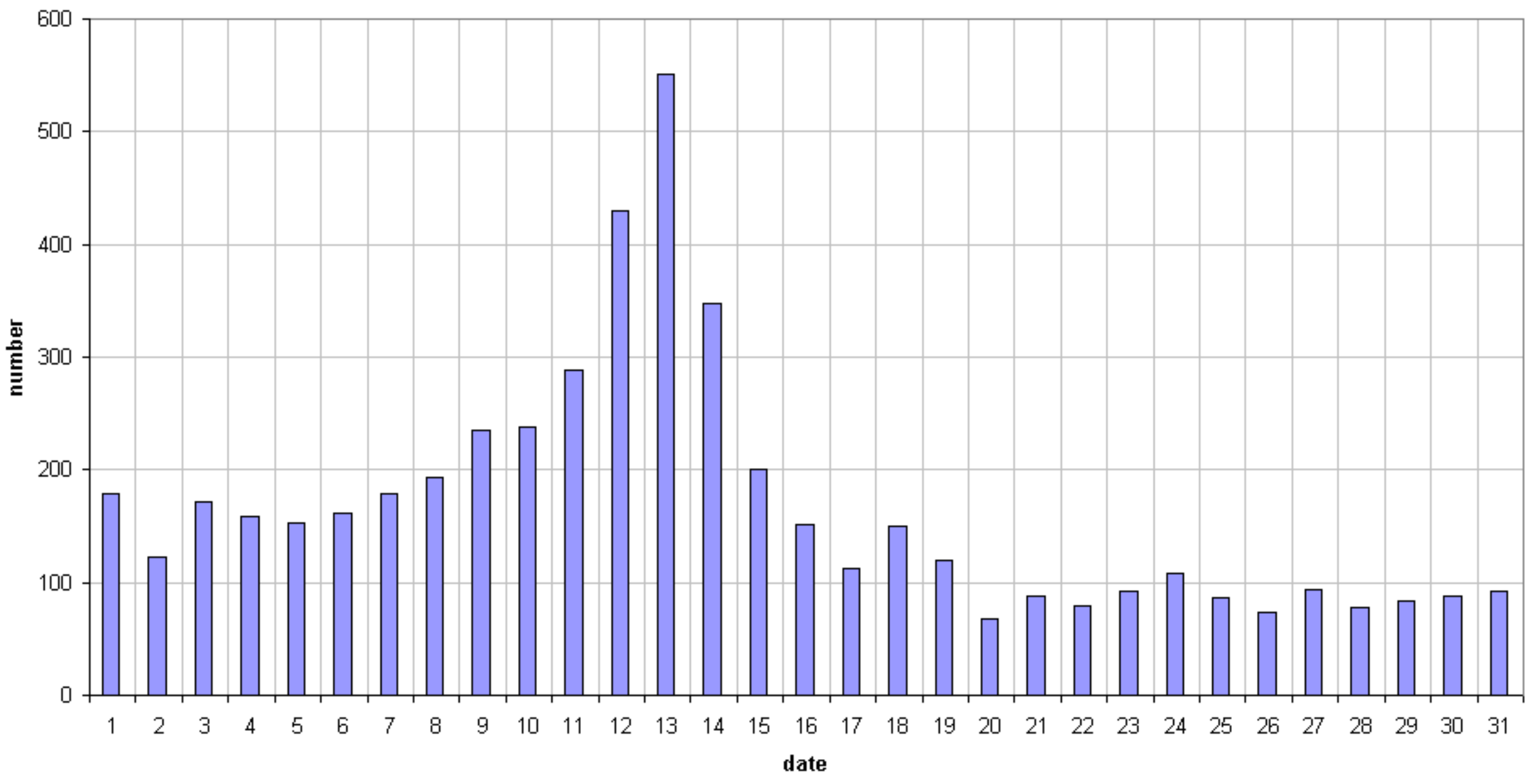
49.99MHz - RadioMeteors August 2018 daily totals of all overdense reflections Felix Verbelen (Kampenhout)
