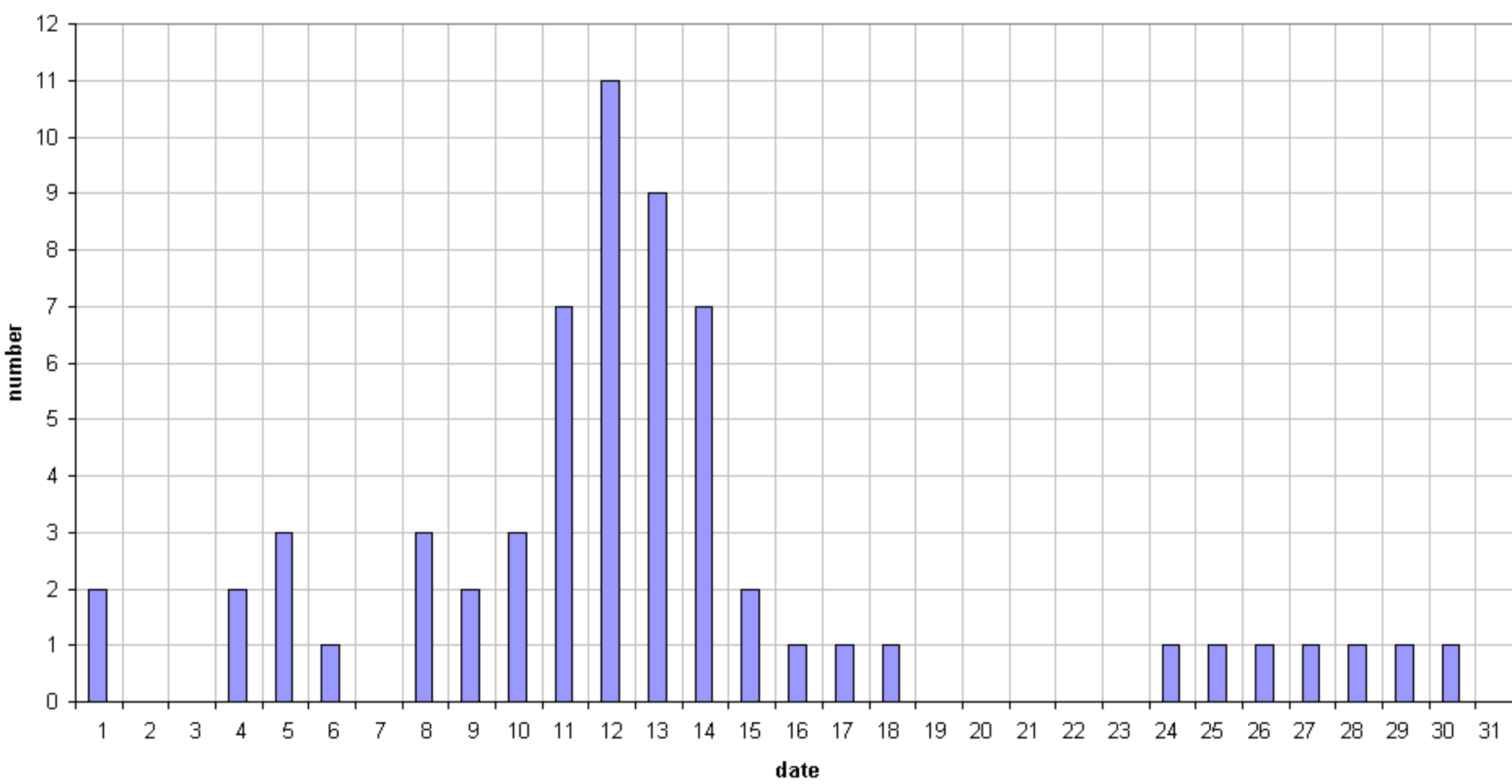
49.99MHz - RadioMeteors August 2018 daily totals of reflections longer than 1 minute Felix Verbelen (Kampenhout)
