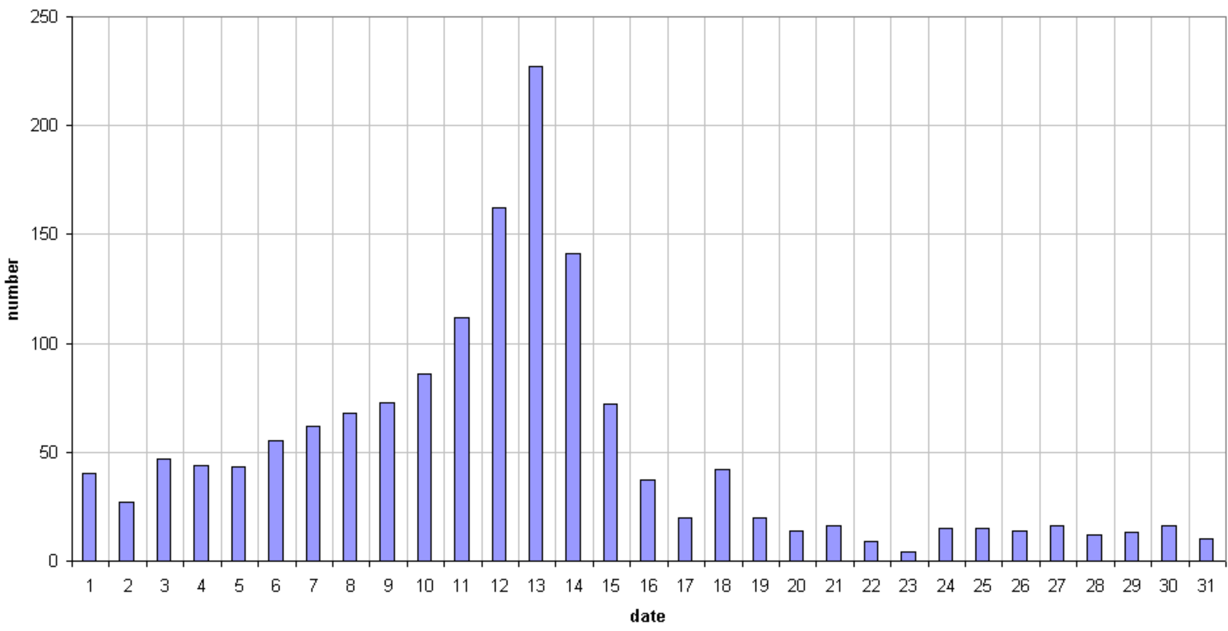
49.99MHz - RadioMeteors August 2018 daily totals of reflections longer than 10 seconds Felix Verbelen (Kampenhout)
