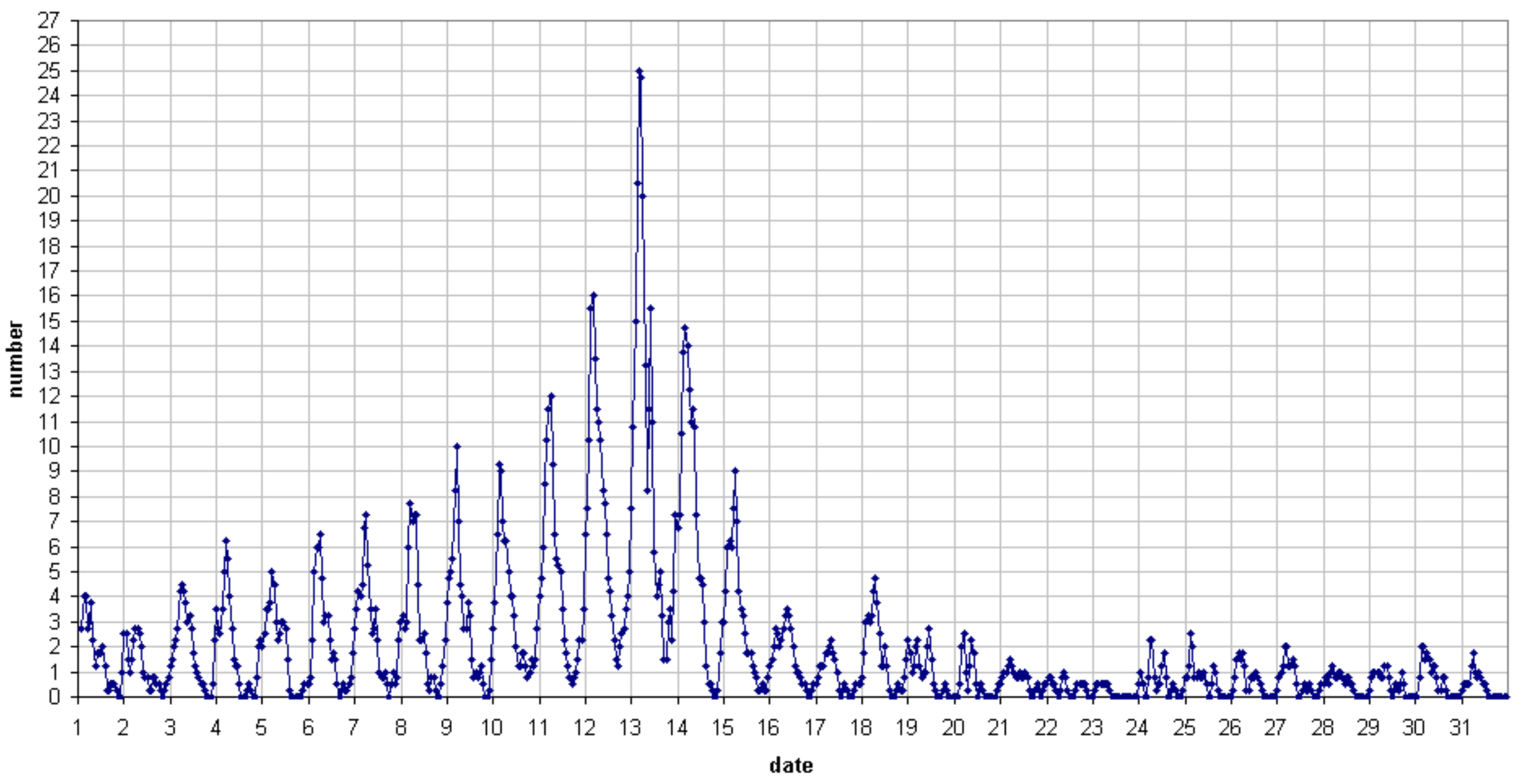
49.99MHz - RadioMeteors August 2018 number of reflections >10 seconds per hour (weighted average) Felix Verbelen (Kampenhou)
