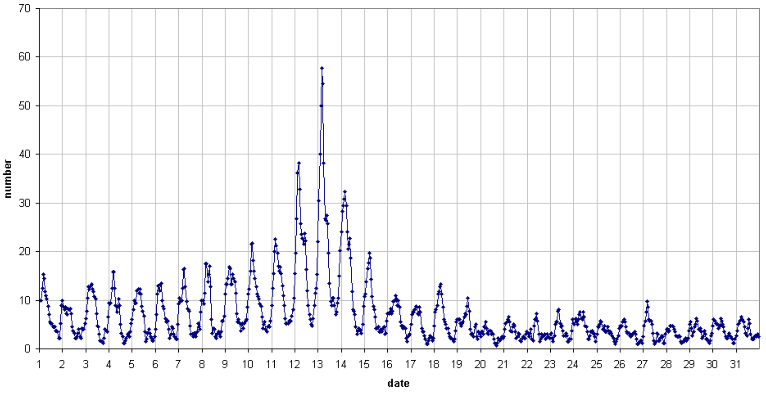
49.99MHz - RadioMeteors August 2018 number of overdense reflections per hour (weighted average) Felix Verbelen (Kampenhou)
