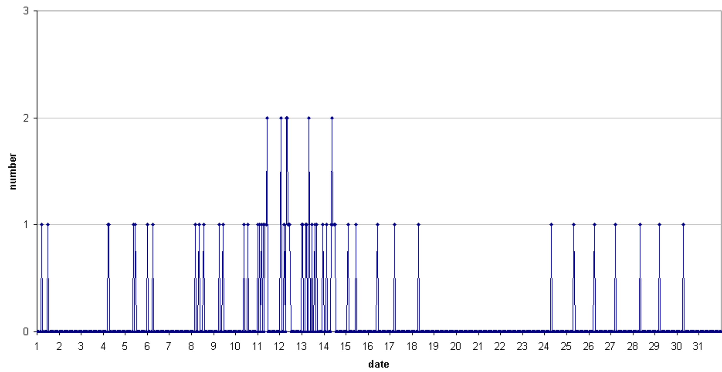
49.99MHz - RadioMeteors August 2018 hourly totals of overdense reflections longer than 1 minute Felix Verbelen (Kampenhou/BE)
