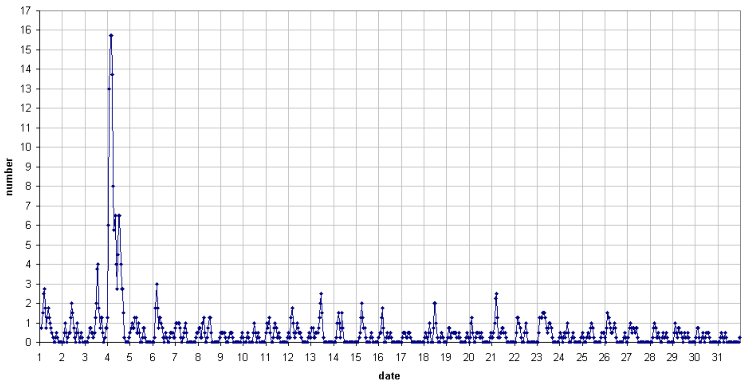
49.99MHz - RadioMeteors January 2019 number of reflections >10 seconds per hour (weighted average) Felix Verbelen (Kampenhout)
