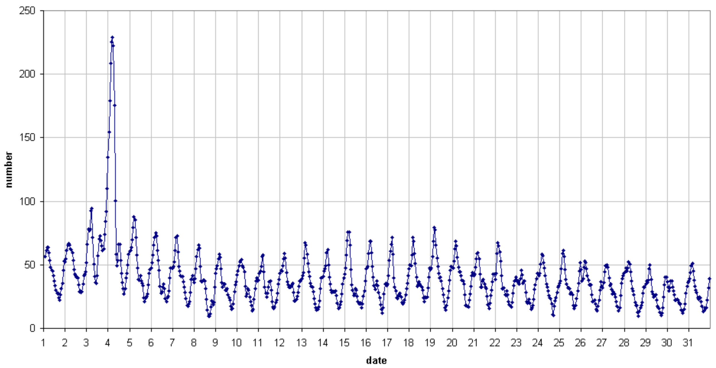
49.99 MHz - RadioMeteors January 2019 number of "all" reflections per hour (weighted average) (automatic count_Mette15_7Hz) Felix Verbelen (Kampenhout)
