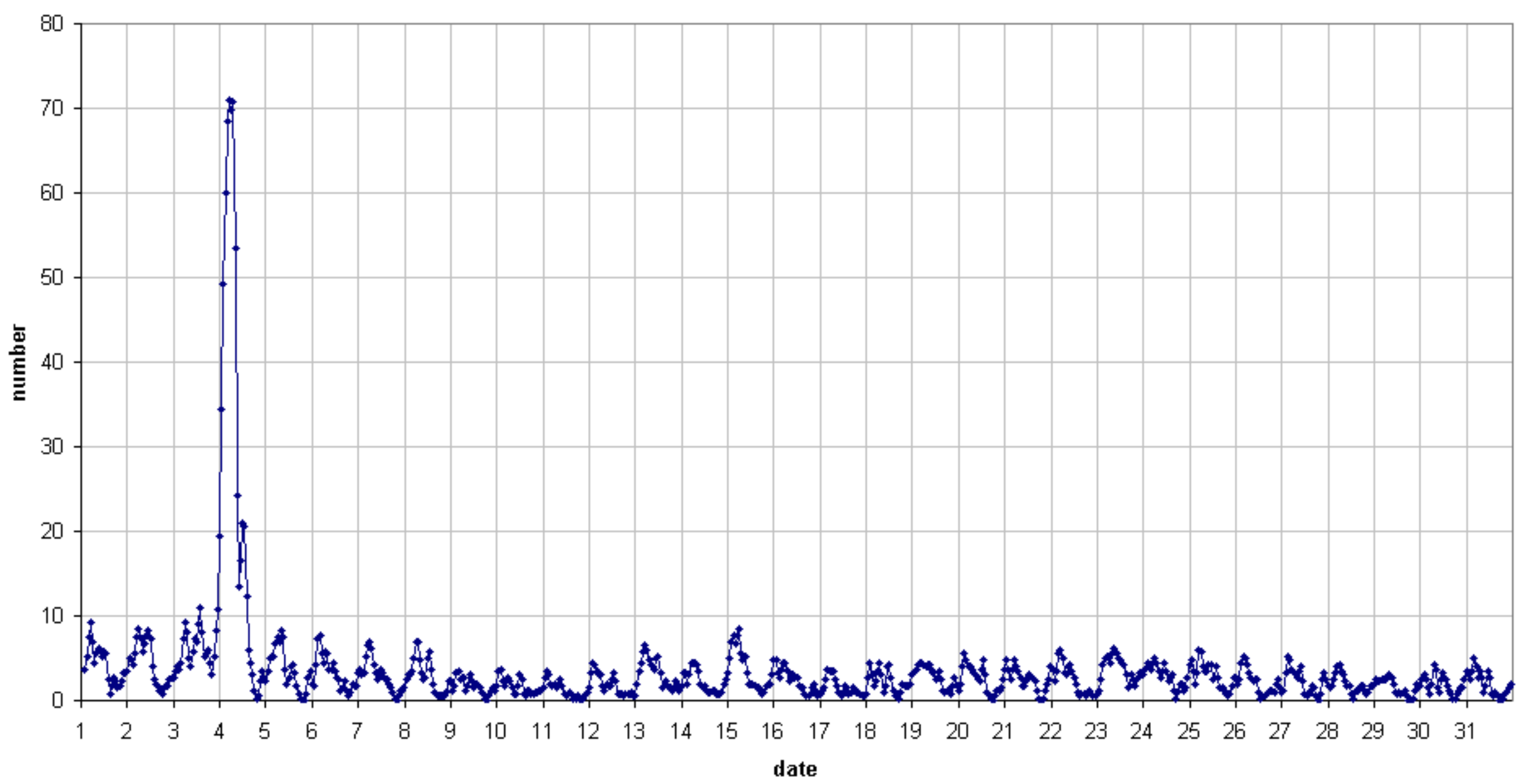
49.99MHz - RadioMeteors January 2019 number of overdense reflections per hour (weighted average) Felix Verbelen (Kampenhout)
