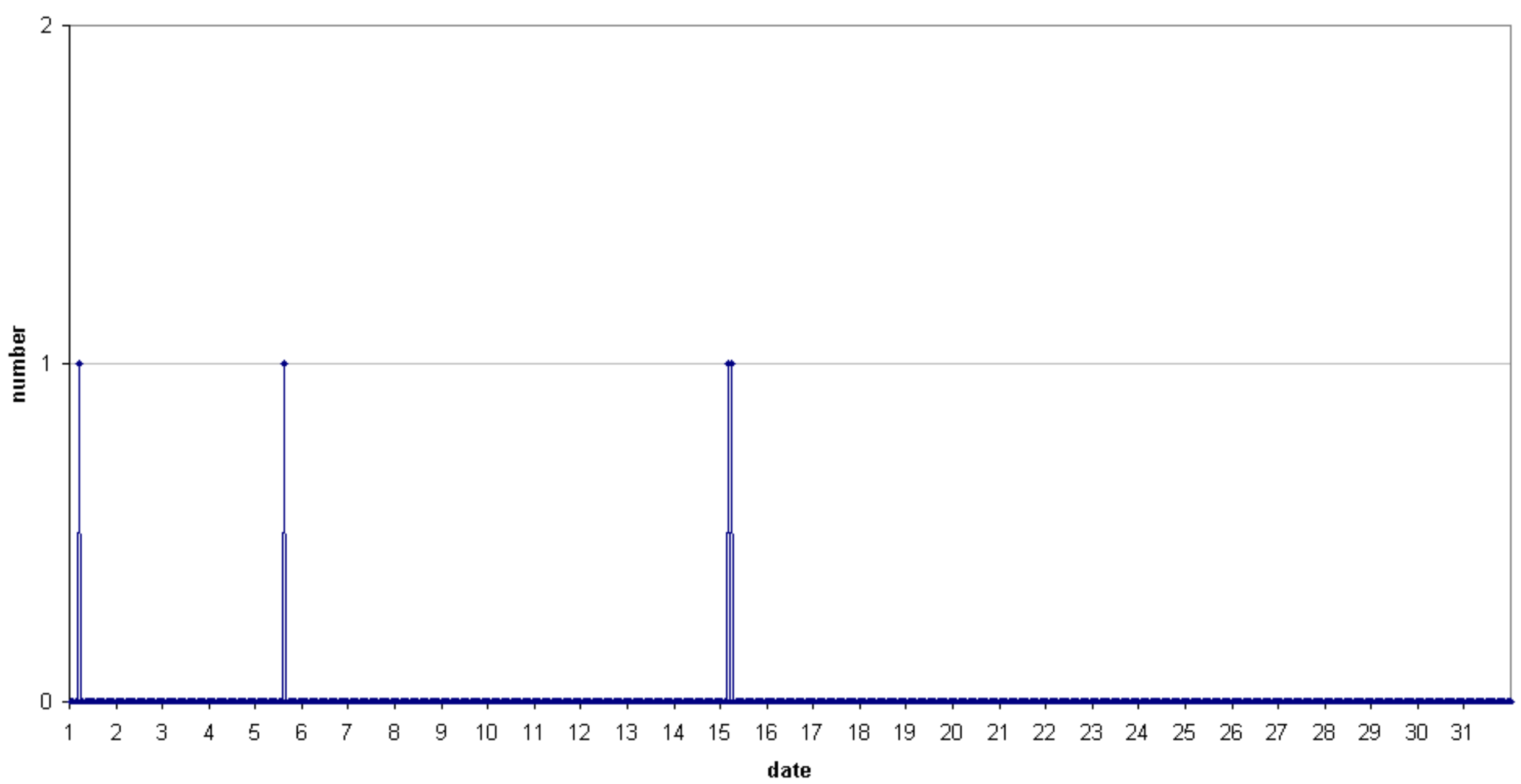
49.99MHz - RadioMeteors January 2019 hourly totals of overdense reflections longer than 1 minute Felix Verbelen (Kampenhout/BE)
