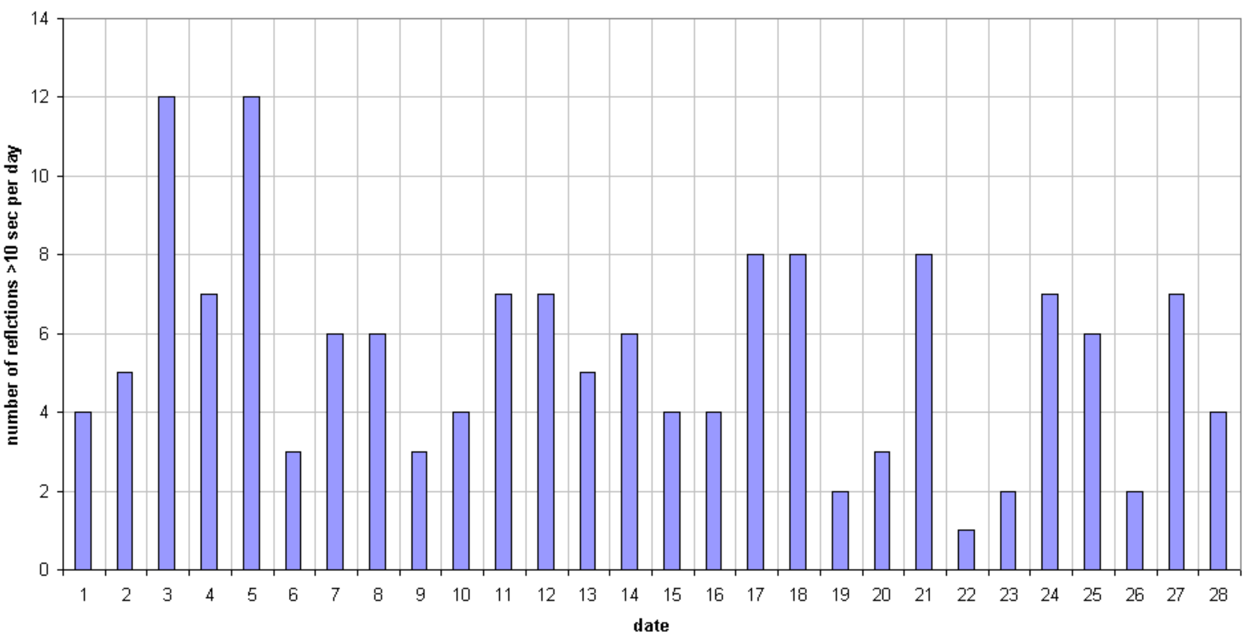
49.99MHz - RadioMeteors February 2019 daily totals of reflections longer than 10 seconds Felix Verbelen (Kampenhout)
