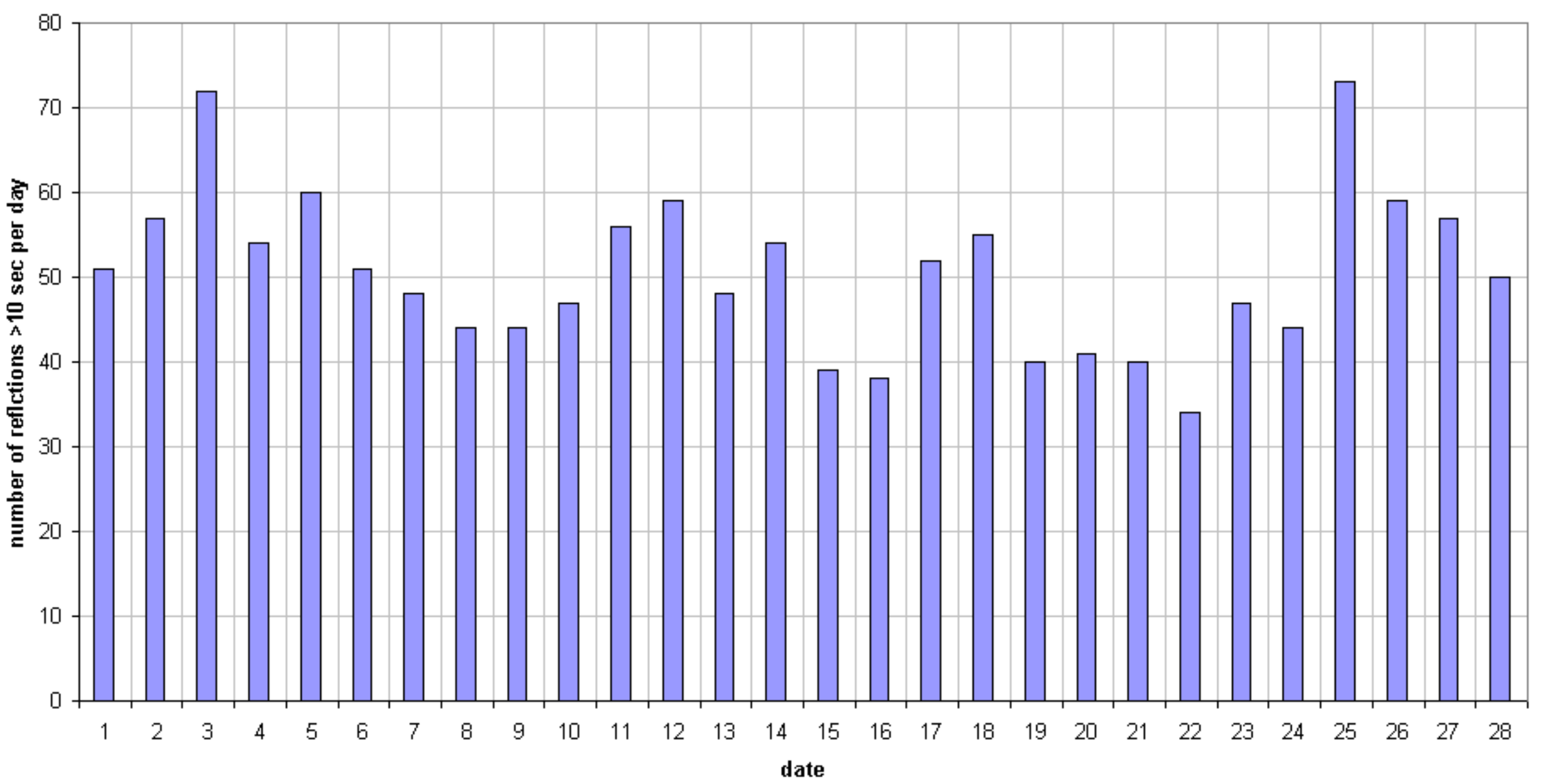
49.99MHz - RadioMeteors February 2019 daily totals of all overdense reflections Felix Verbelen (Kampenhout)
