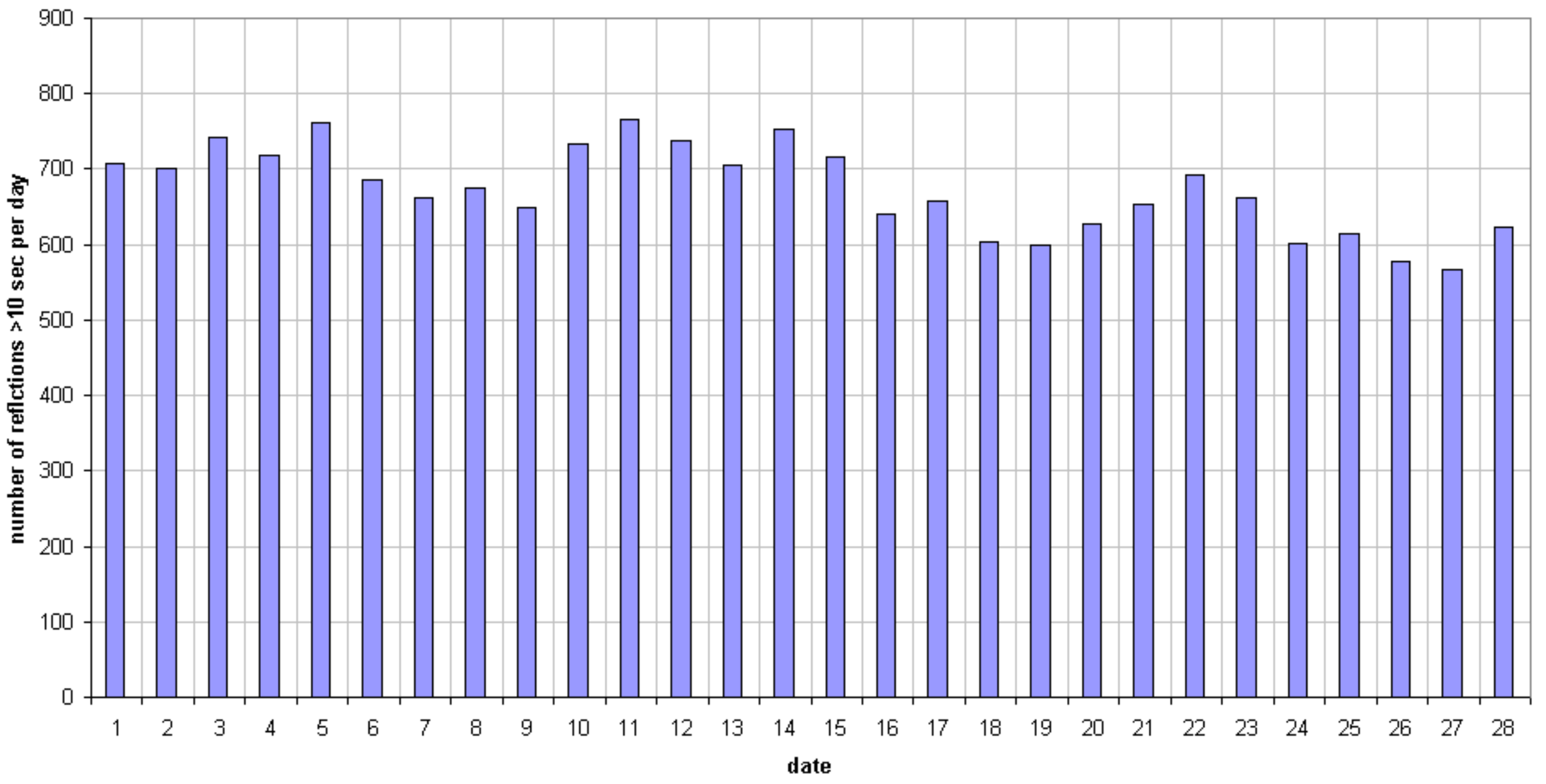
49.99MHz - RadioMeteors February 2019 daily totals of "all" reflections (automatic count_Mette15_7Hz) Felix Verbelen (Kampenhout)
