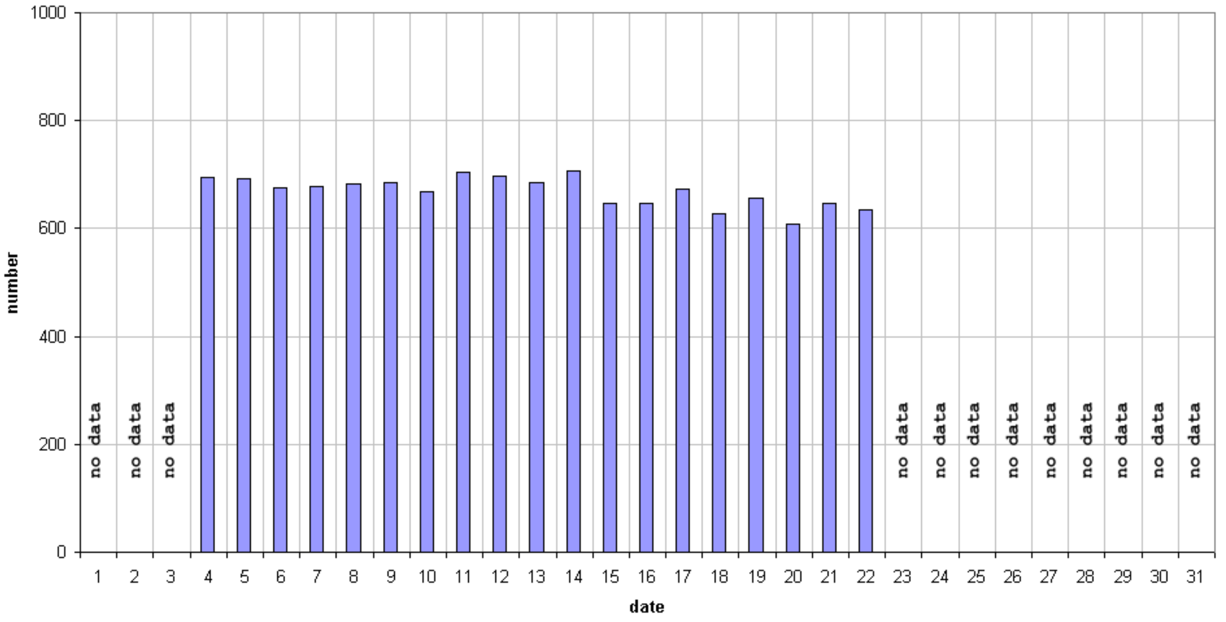
49.99MHz - RadioMeteors March 2019 daily totals of all overdense reflections Felix Verbelen (Kampenhout)
