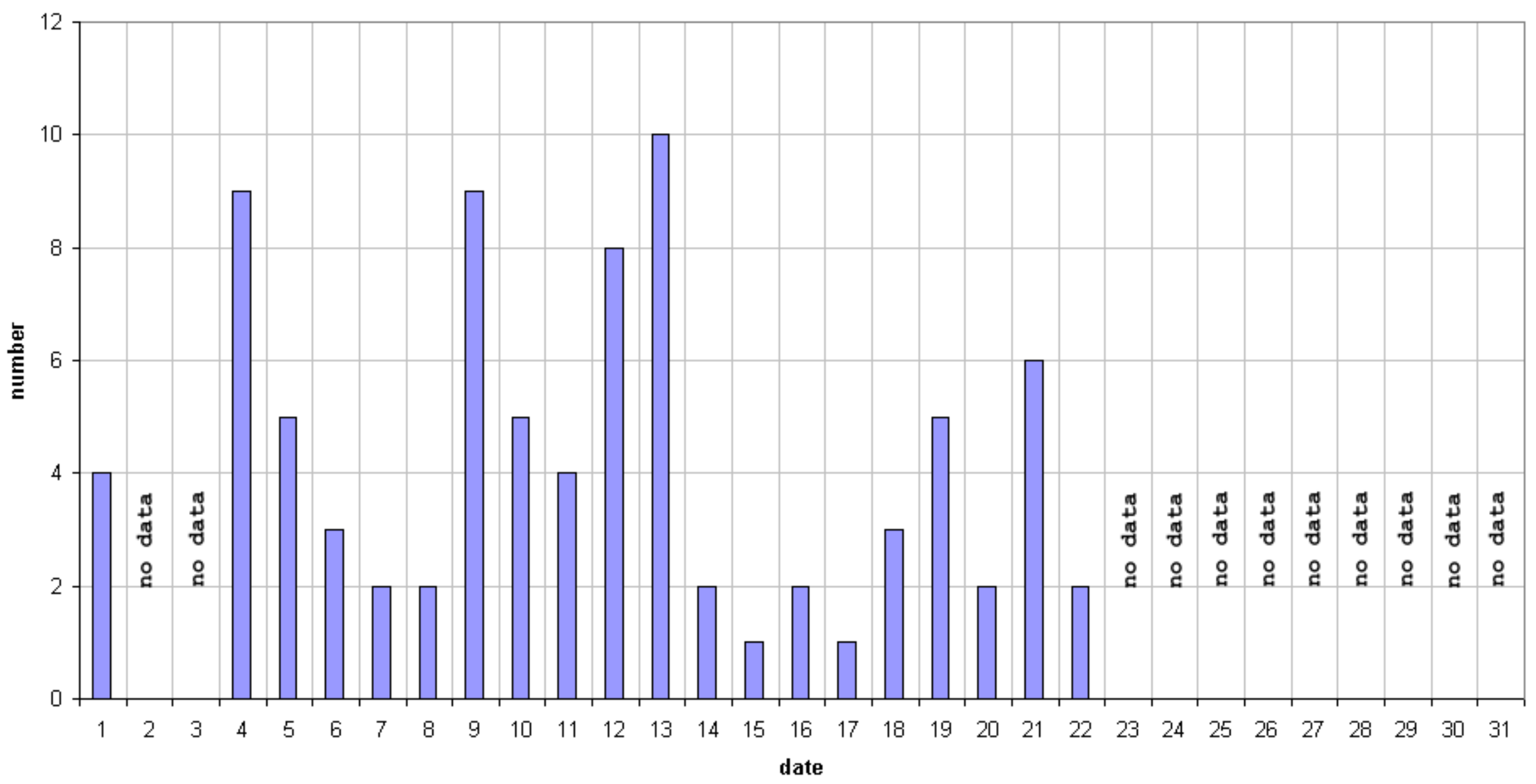
49.99MHz - RadioMeteors March 2019 daily totals of reflections longer than 10 seconds Felix Verbelen (Kampenhout)
