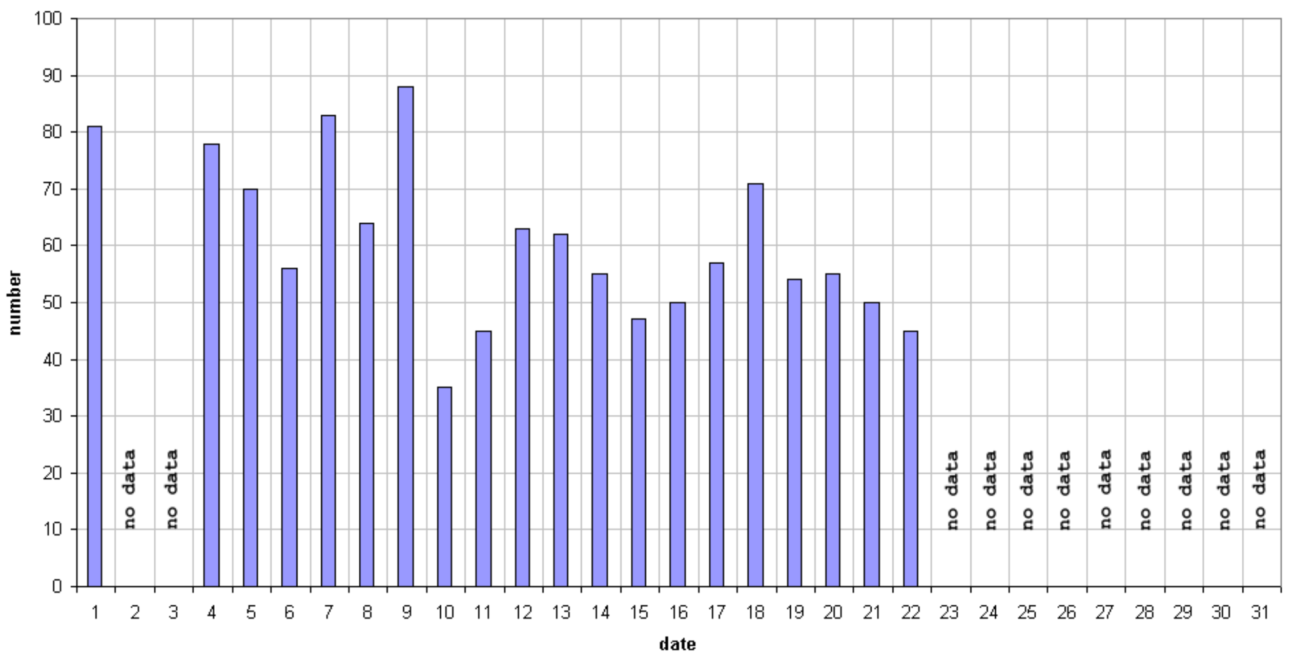
49.99MHz - RadioMeteors March 2019 daily totals of all overdense reflections Felix Verbelen (Kampenhout)
