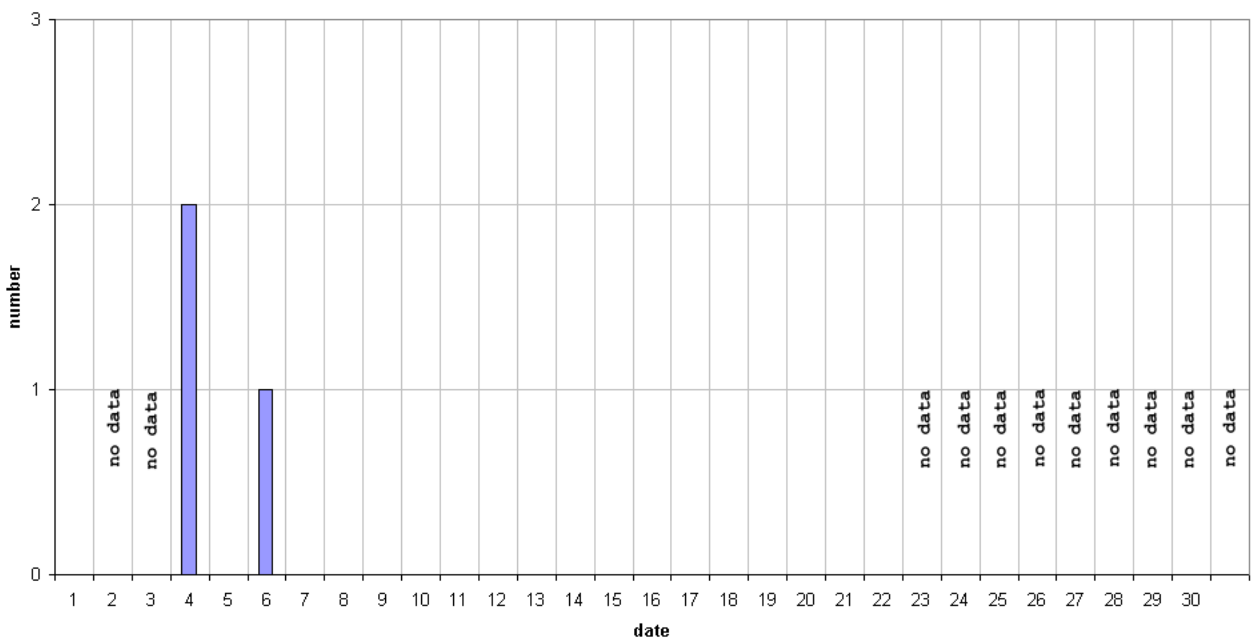
49.99MHz - RadioMeteors March 2019 daily totals of reflections longer than 1 minute Felix Verbelen (Kampenhout)
