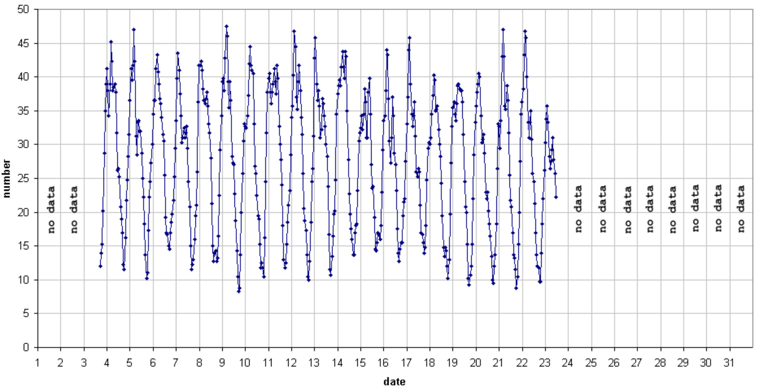
49.99 MHz - RadioMeteors March 2019 number of "all" reflections per hour (weighted average) (automatic count_Mette5_7Hz) Felix Verbelen (Kamphenhout)
