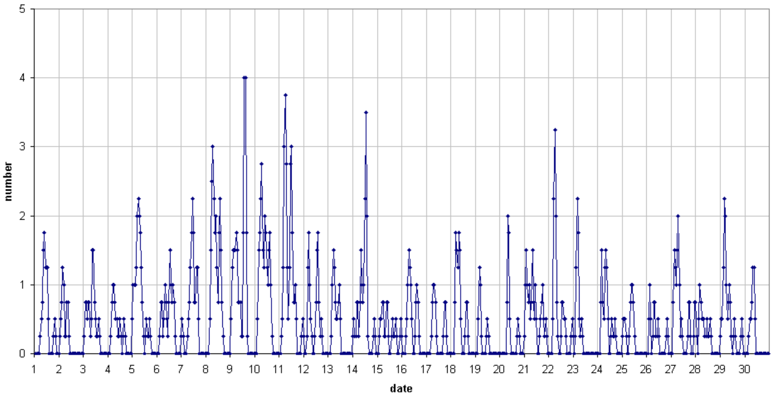
49.99MHz - Radiometeors June 2019 number of reflections >10 seconds per hour (weighted average) Felix Verbelen (Kamphenhout)
