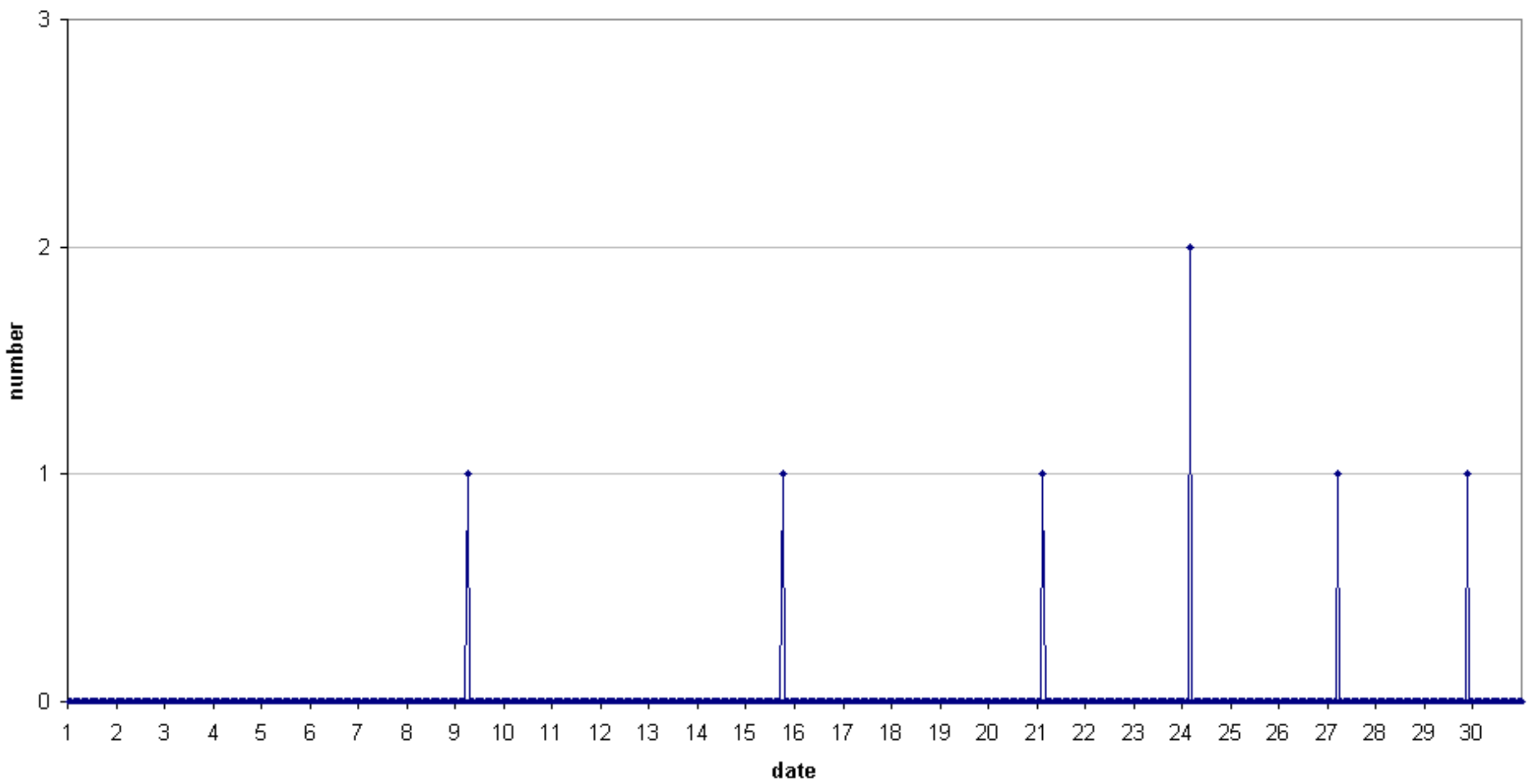
49.99MHz - Radiometeors June 2019 hourly totals of overdense reflections longer than 1 minute Felix Verbelen (Kamphenhout/BE)
