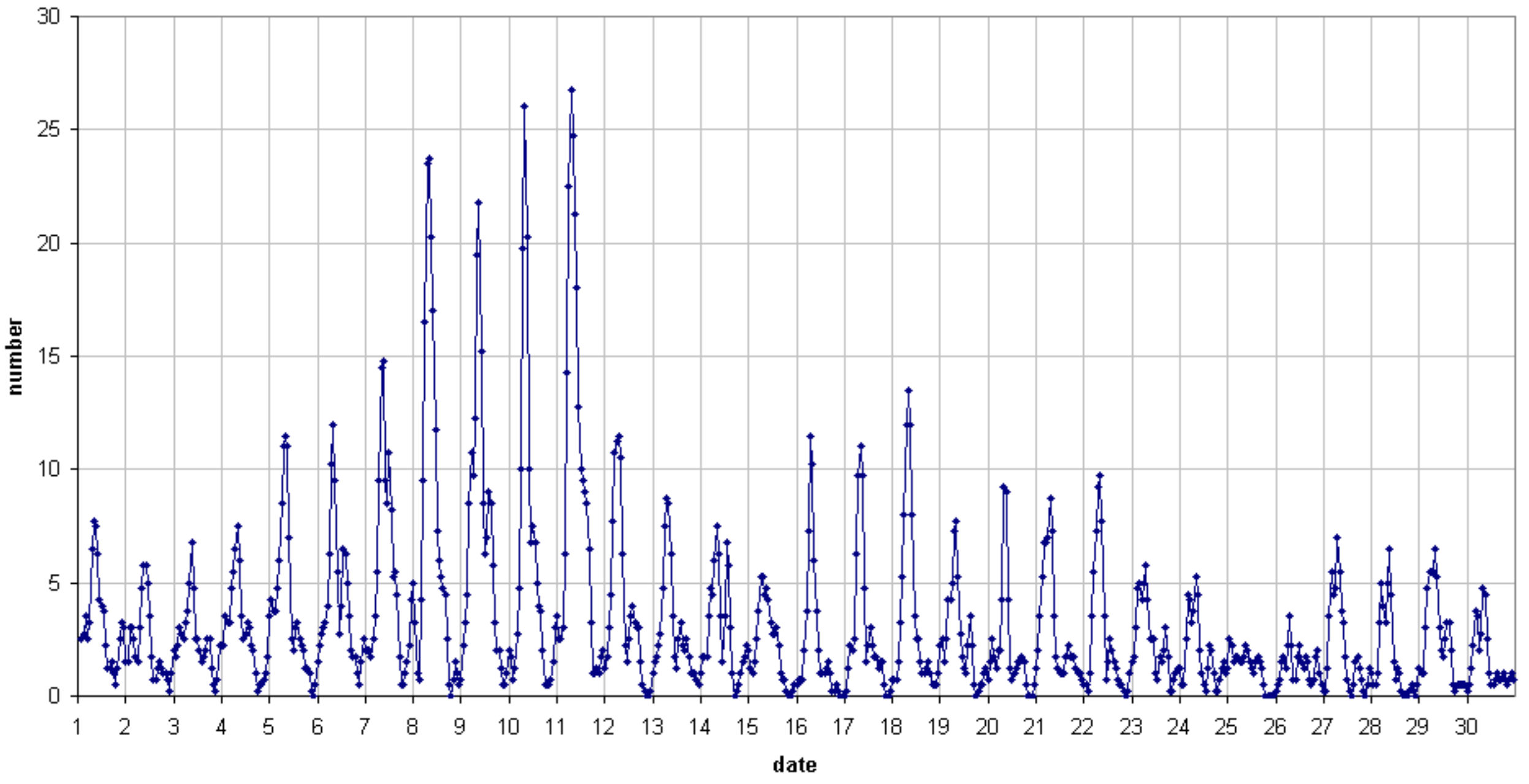
49.99MHz - Radiometeors June 2019 number of overdense reflections per hour (weighted average) Felix Verbelen (Kamphenhout)
