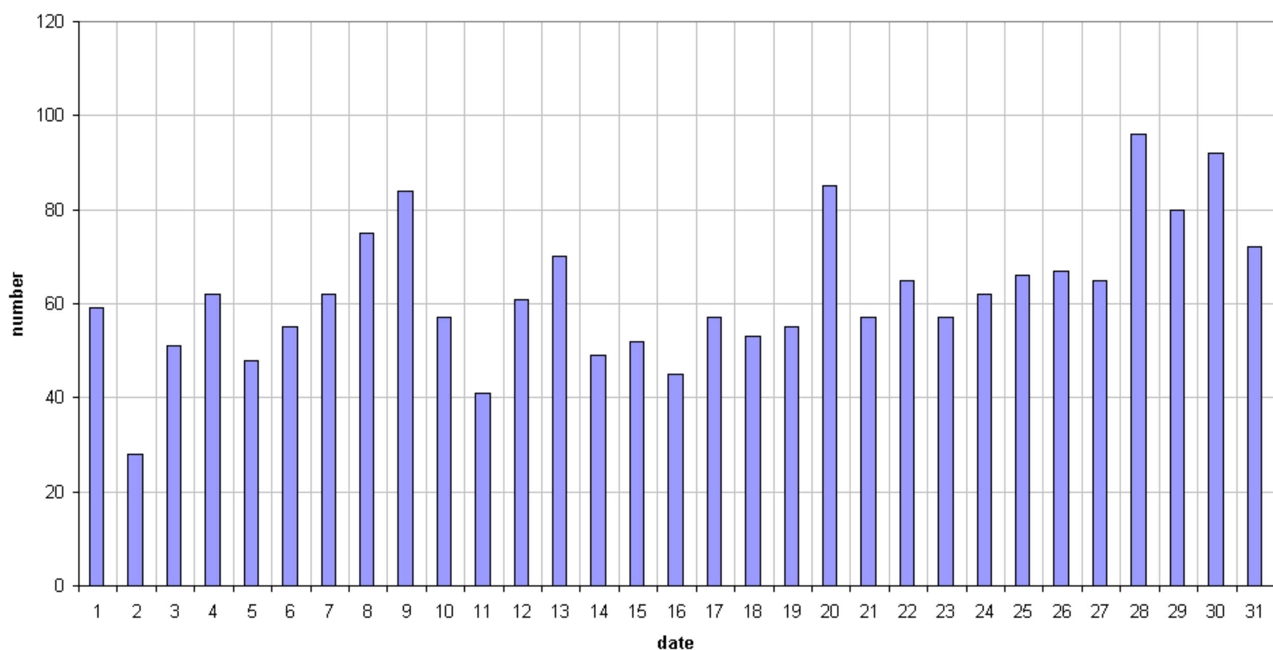
49.99MHz - RadioMeteors July 2019 daily totals of all overdense reflections Felix Verbelen (Kampenhout)
