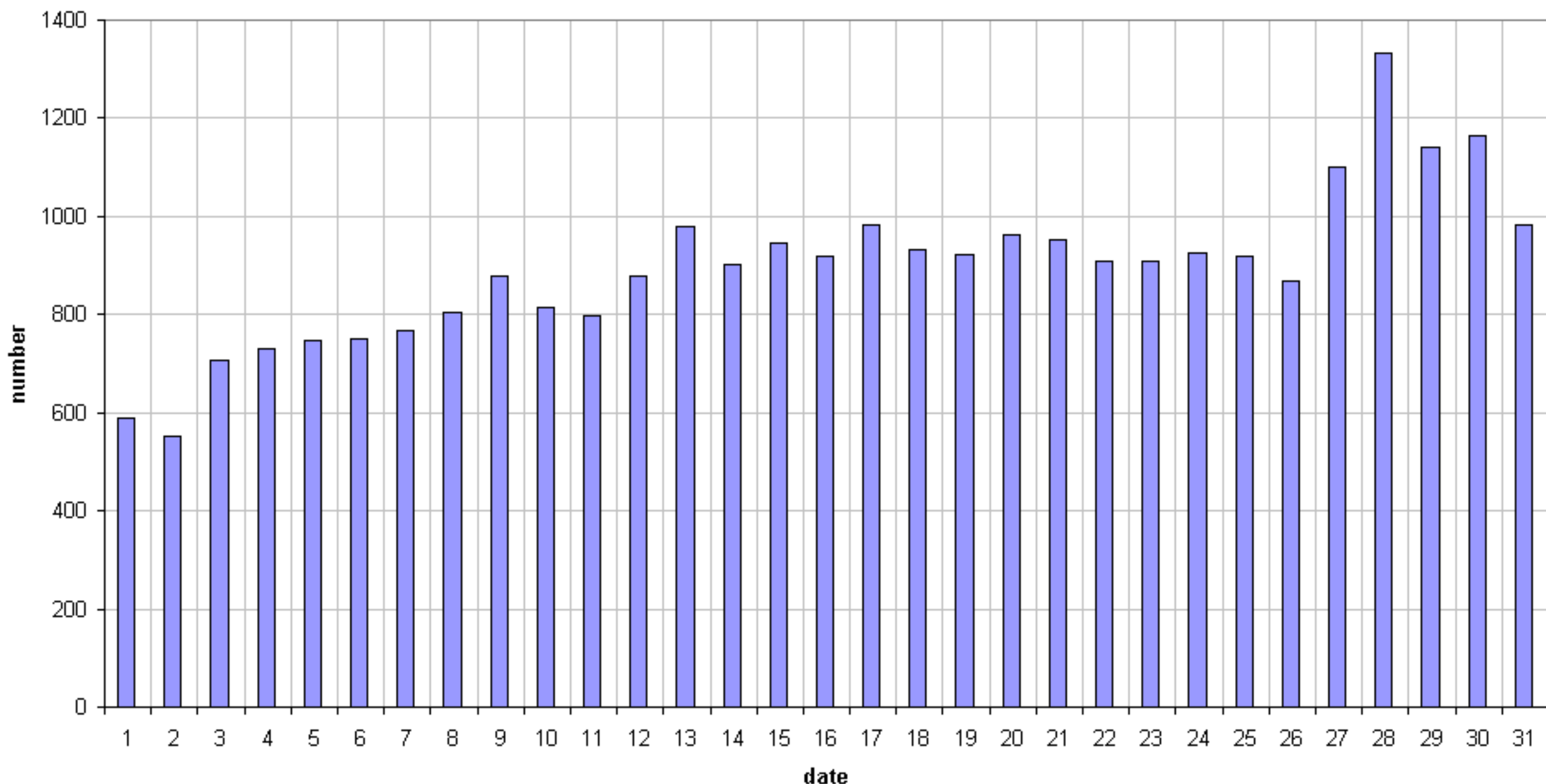
49.99MHz - RadioMeteors July 2019 daily totals of "all" reflections (automatic count_Mette15_7Hz) Felix Verbelen (Kampenhout)
