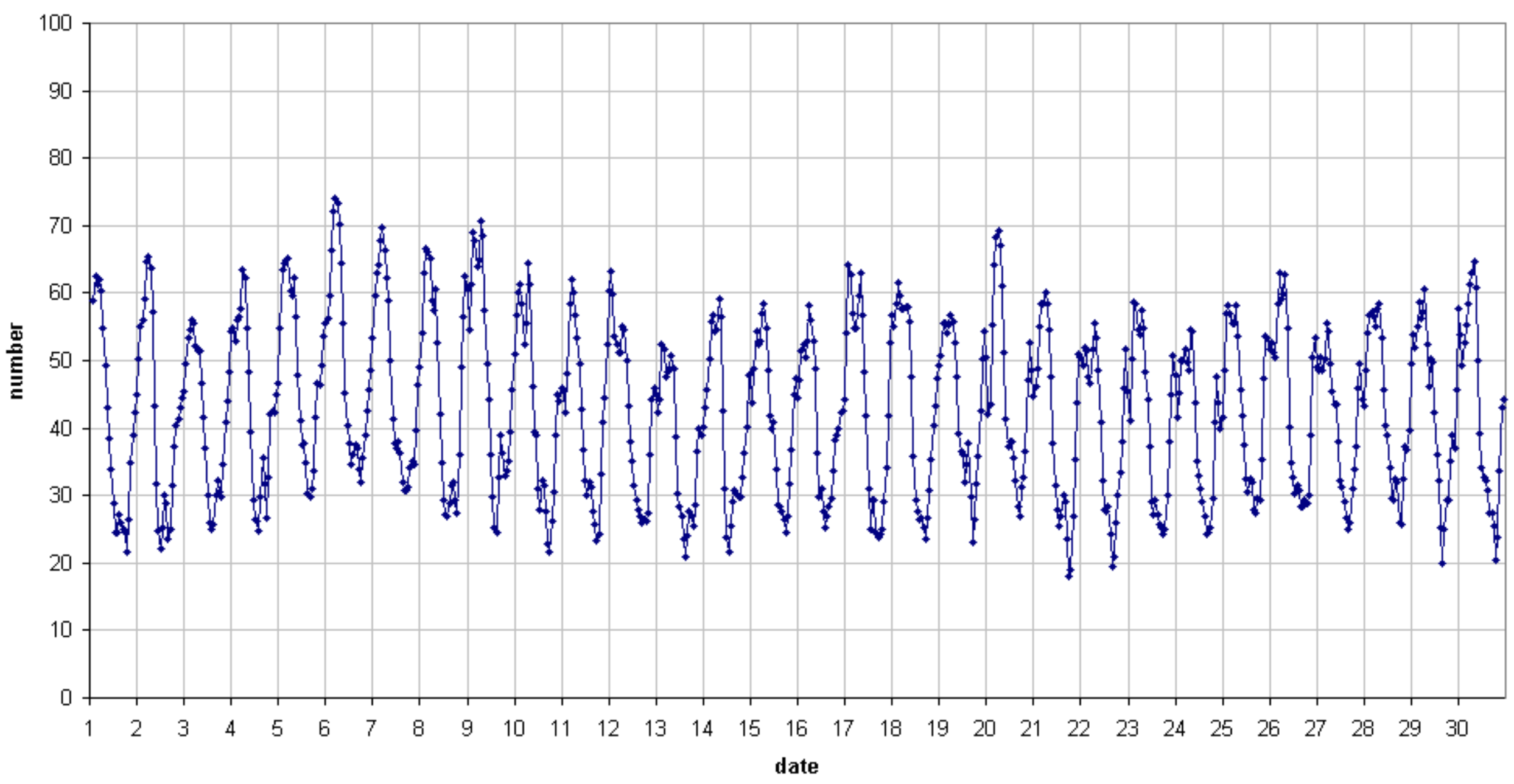
49.99 MHz - RadioMeteors September 2019 number of "all" reflections per hour (weighted average) (automatic count_Mette15_7Hz) Felix Verbelen (Kamphenhout)
