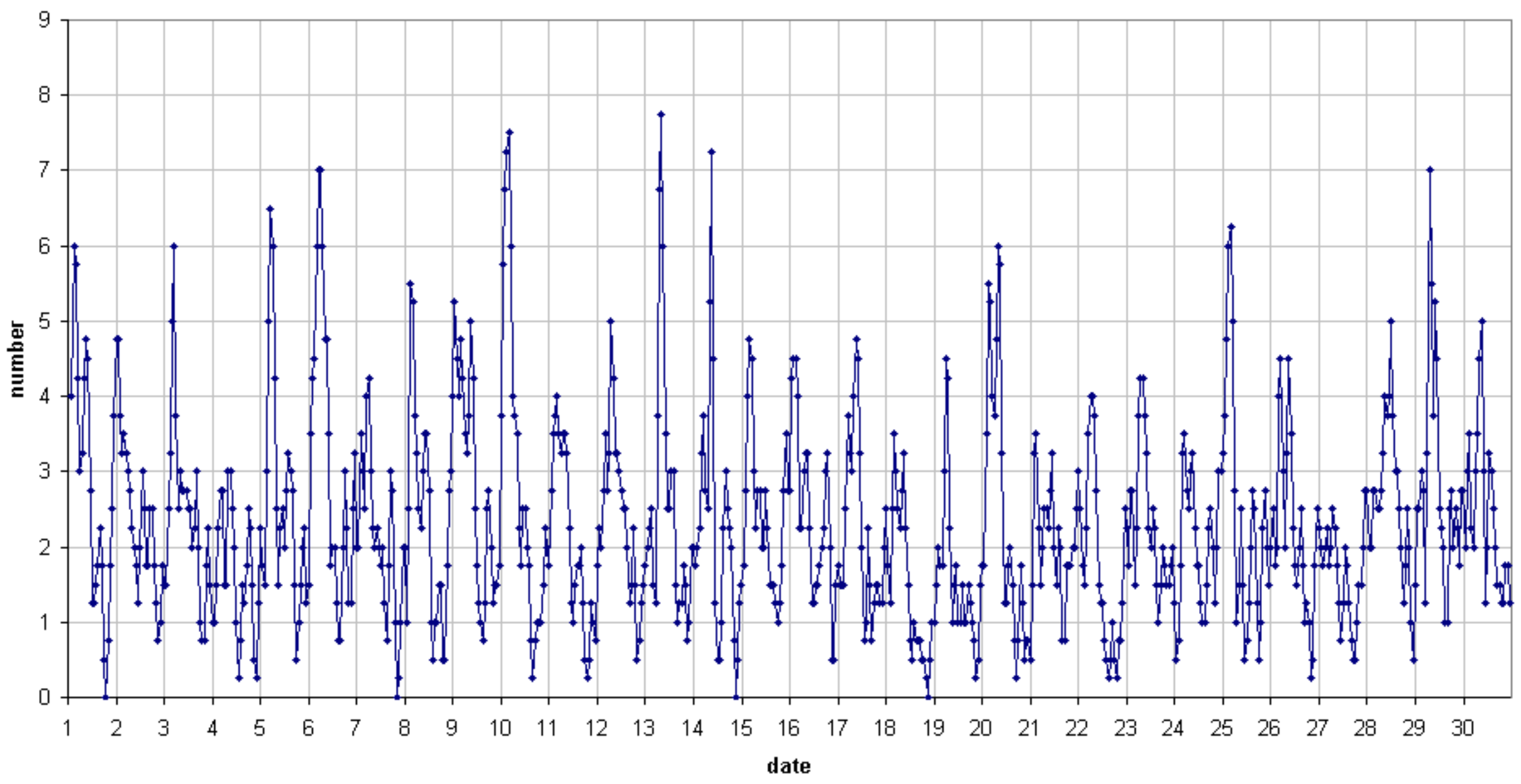
49.99MHz - RadioMeteors September 2019 number of overdense reflections per hour (weighted average) Felix Verbelen (Kamphenhout)
