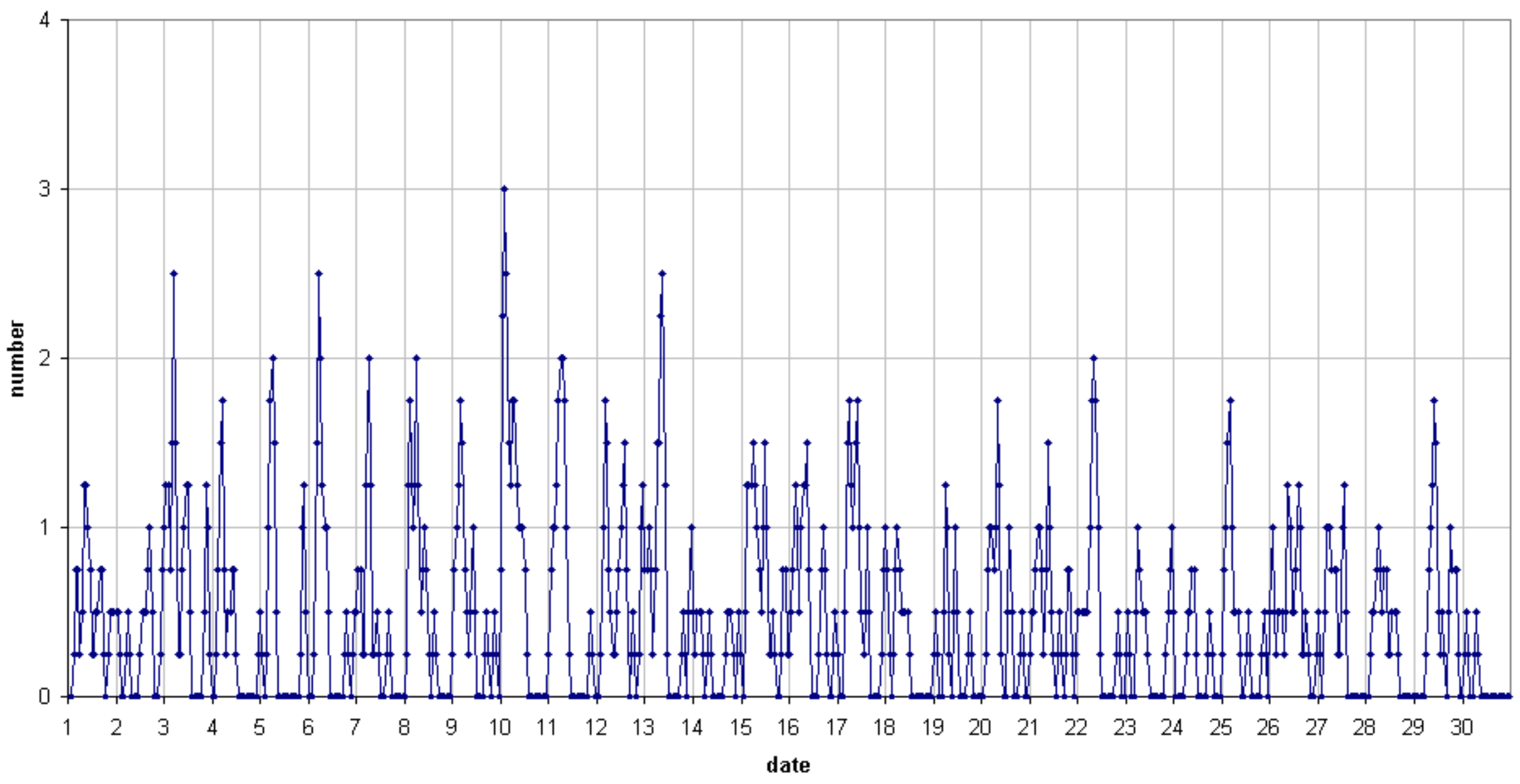
49.99MHz - RadioMeteors September 2019 number of reflections >10 seconds per hour (weighted average) Felix Verbelen (Kamphenhout)
