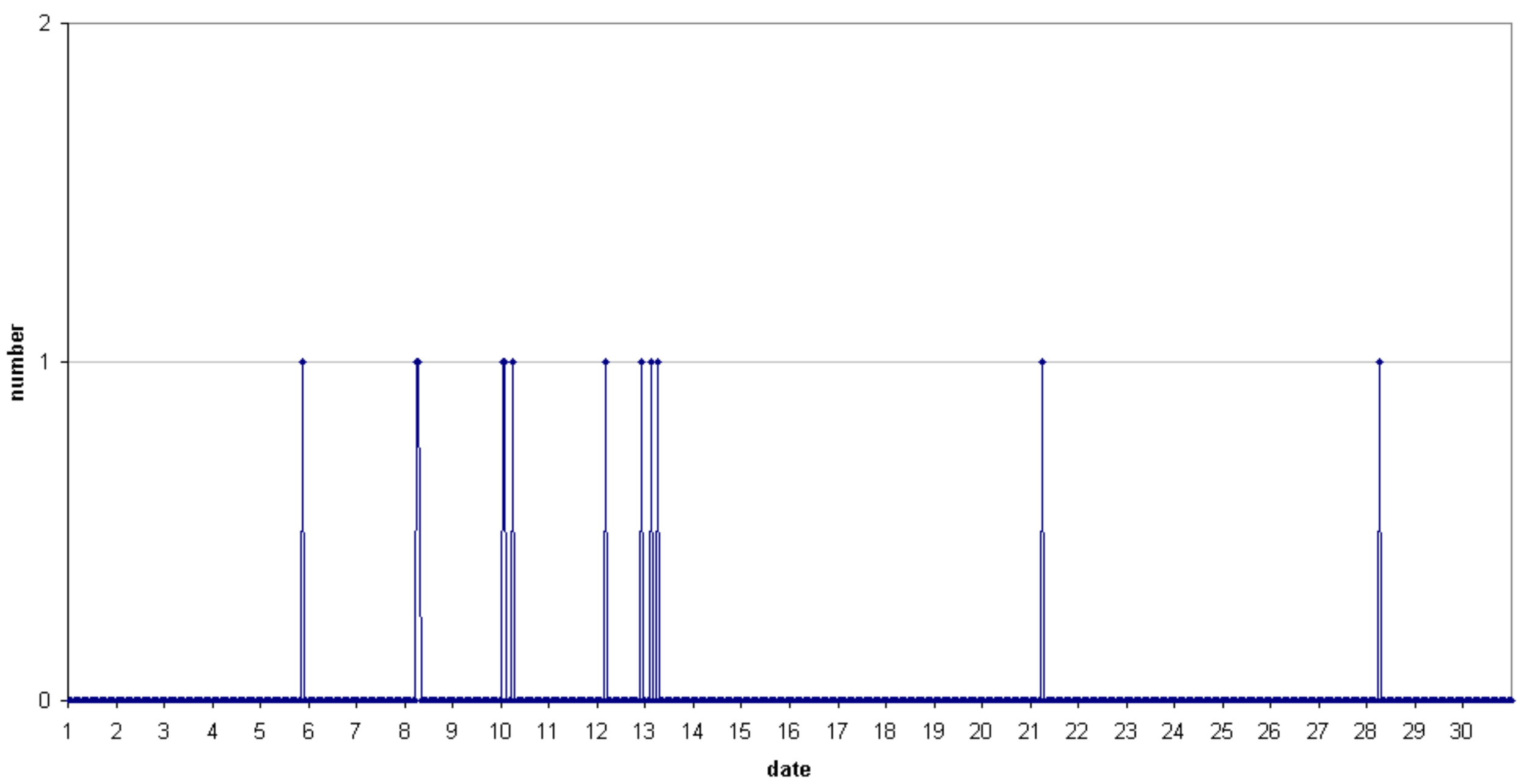
49.99MHz - RadioMeteors September 2019 hourly totals of overdense reflections longer than 1 minute Felix Verbelen (Kamphenhout/BE)
