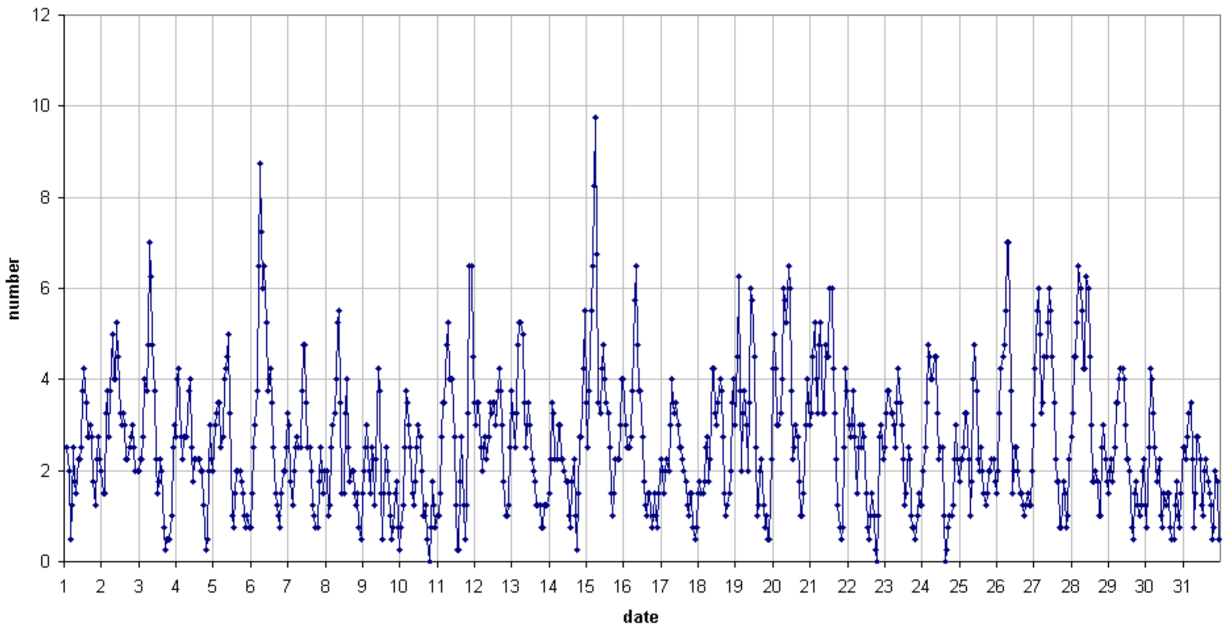
49.99MHz - RadioMeteors October 2019 number of overdense reflections per hour (weighted average) Felix Verbelen (Kampenhout)
