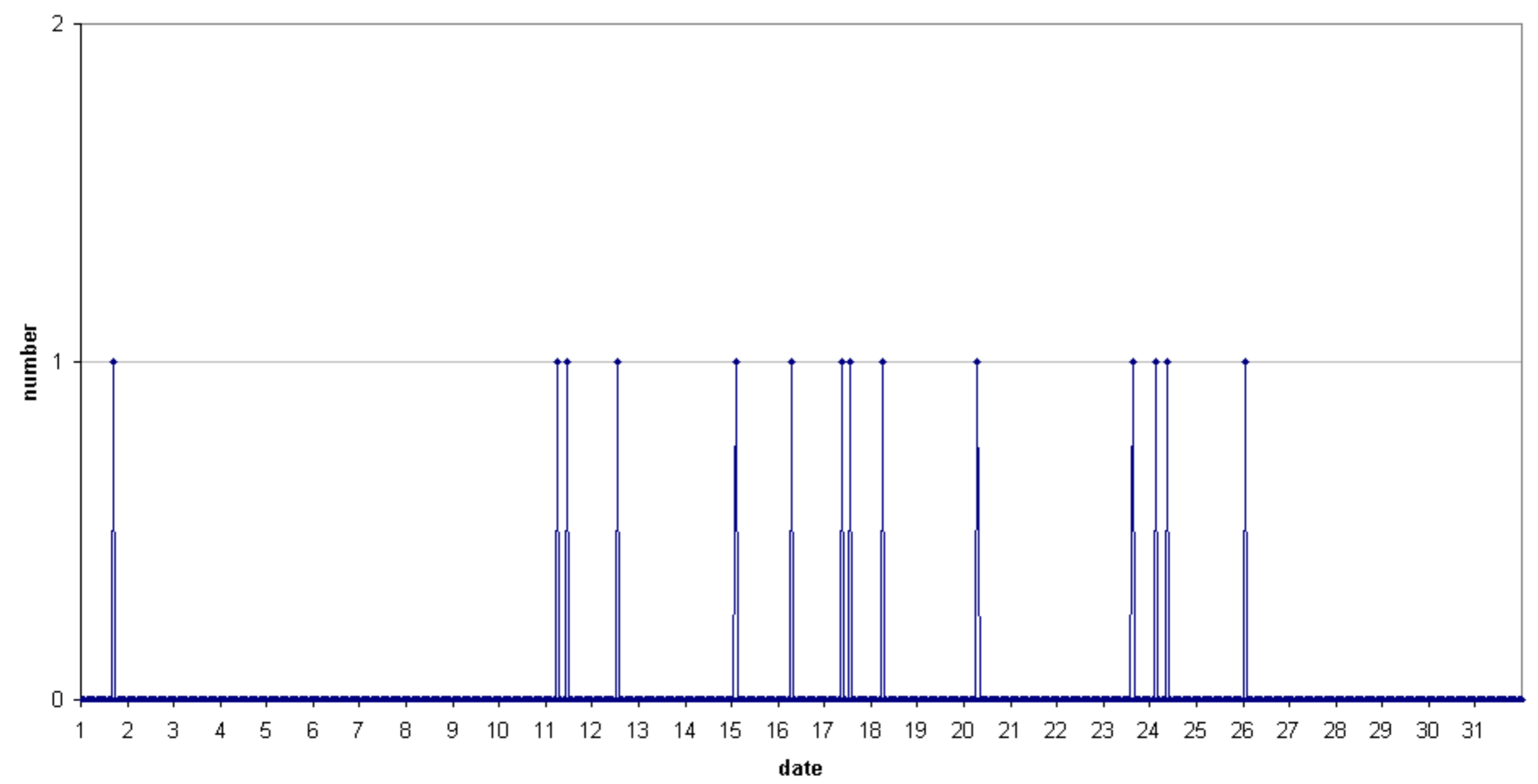
49.99MHz - RadioMeteors October 2019 hourly totals of overdense reflections longer than 1 minute Felix Verbelen (Kampenhout/BE)
