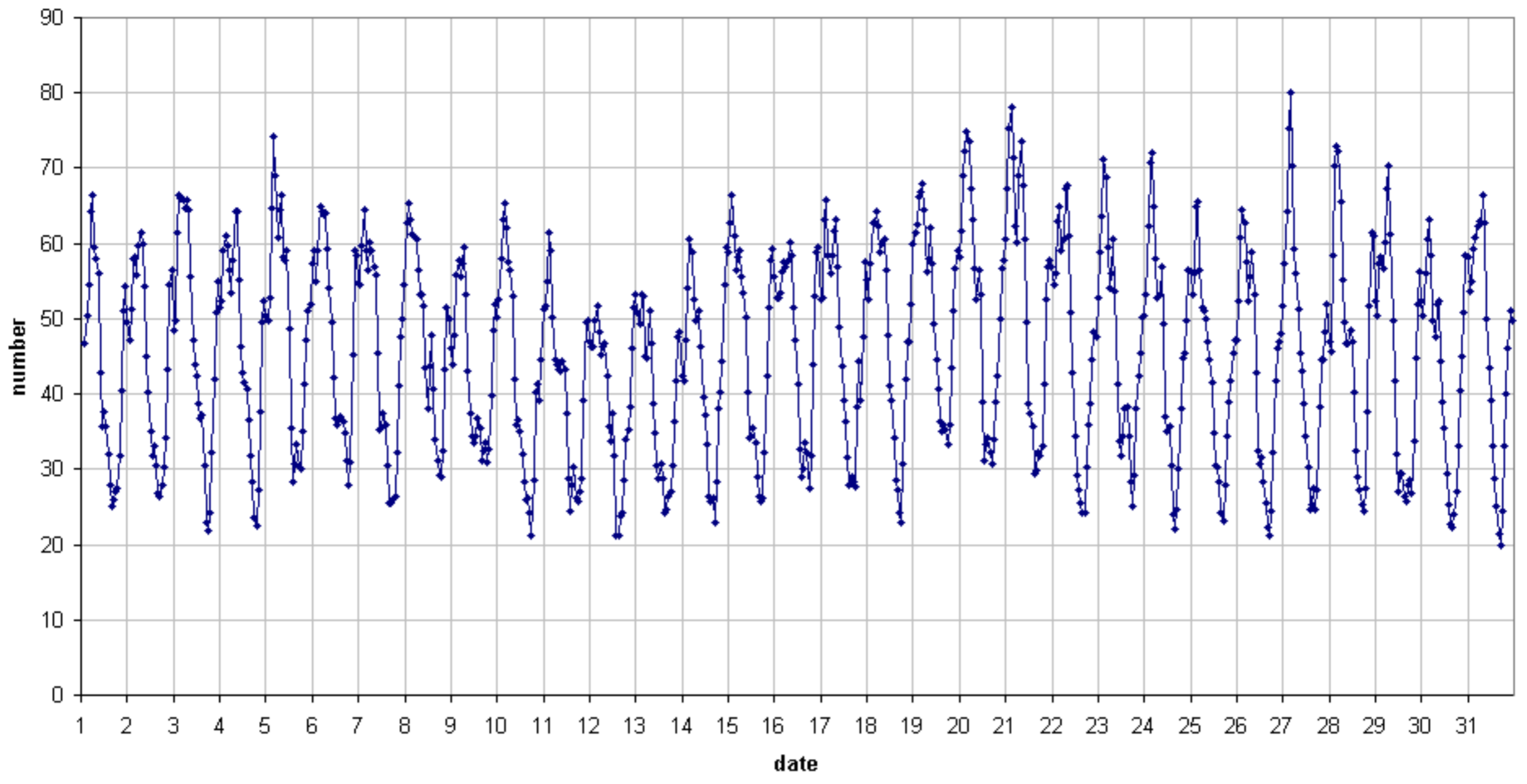
49.99 MHz - RadioMeteors October 2019 number of "all" reflections per hour (weighted average) (automatic count_Mette15_7Hz) Felix Verbelen (Kampenhout)
