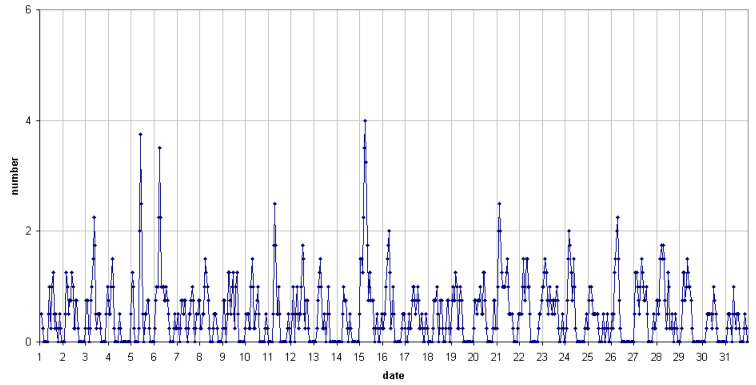
49.99MHz - RadioMeteors October 2019 number of reflections >10 seconds per hour (weighted average) Felix Verbelen (Kampenhout)
