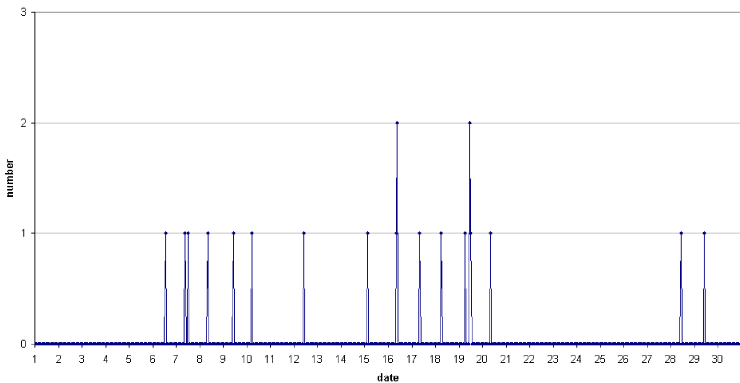
49.99MHz - RadioMeteors November 2019 hourly totals of overdense reflections longer than 1 minute Felix Verbelen (Kampenhout/BE)
