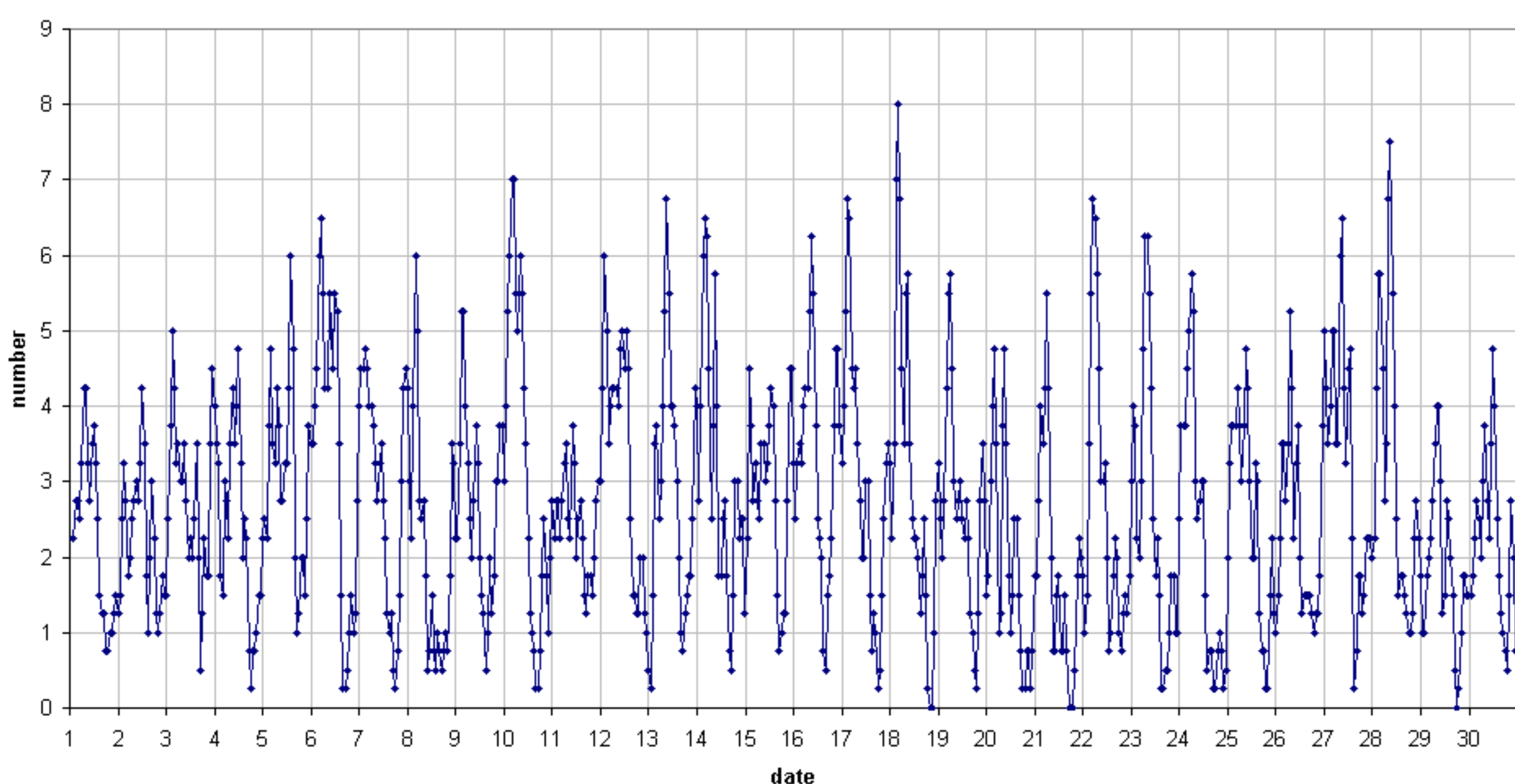
49.99MHz - RadioMeteors November 2019 number of overdense reflections per hour (weighted average) Felix Verbelen (Kampenhout)
