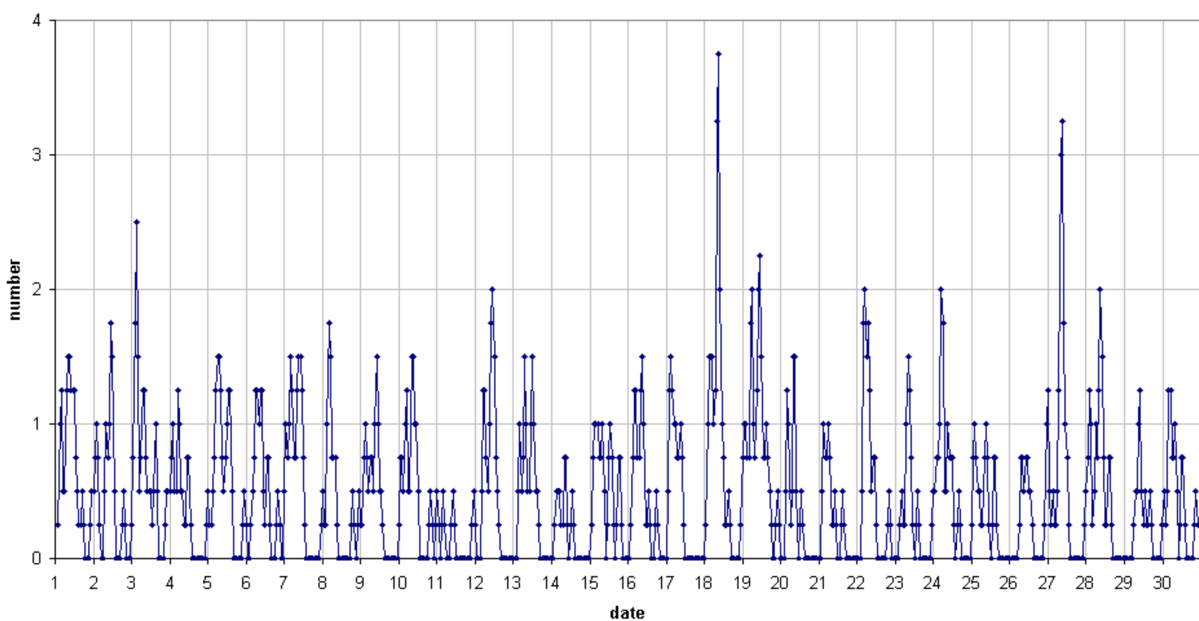
49.99MHz - RadioMeteors November 2019 number of reflections >10 seconds per hour (weighted average) Felix Verbelen (Kampenhout)
