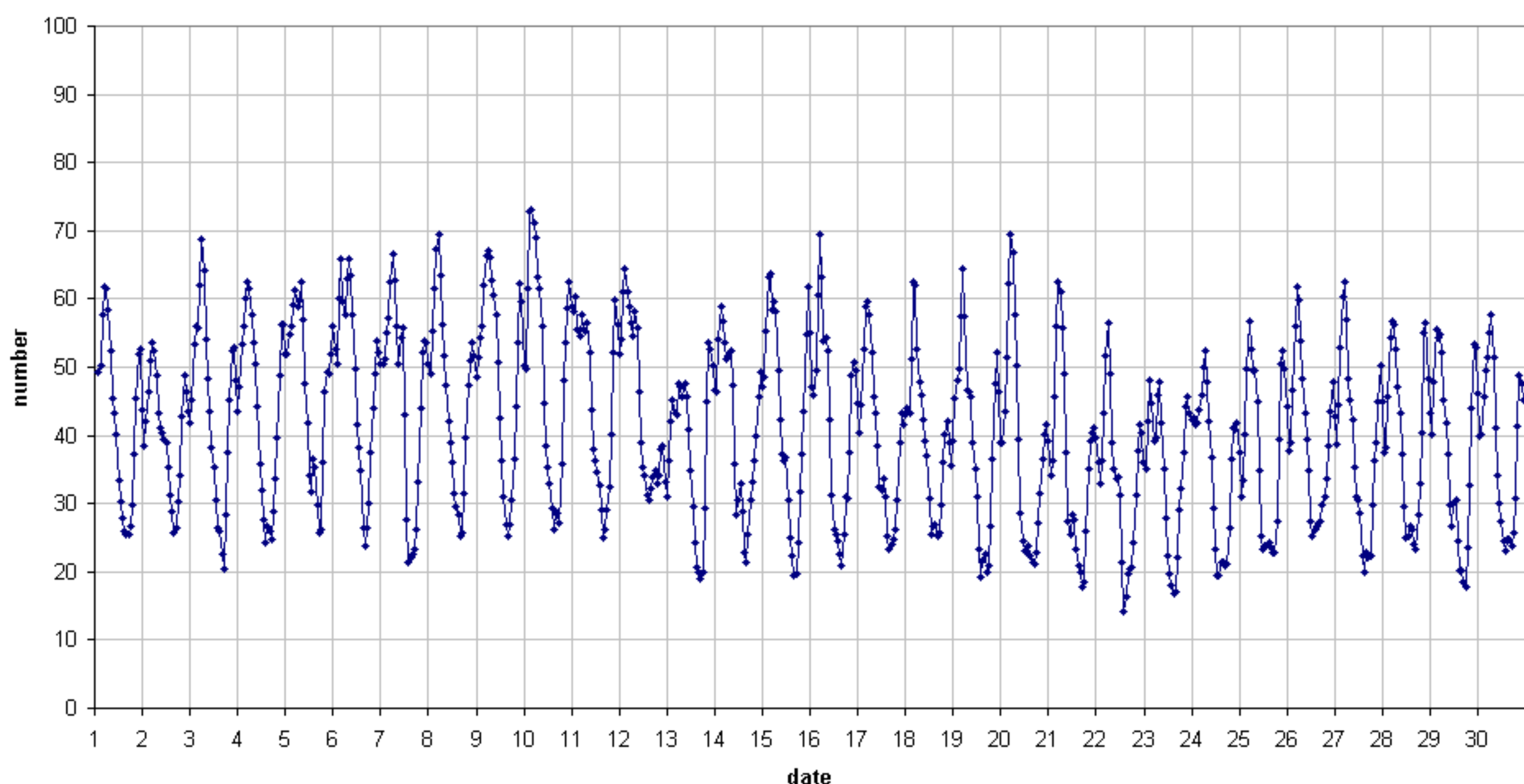
49.99 MHz - RadioMeteors November 2019 number of "all" reflections per hour (weighted average) (automatic count_Mette15_7Hz) Felix Verbelen (Kampenhout)
