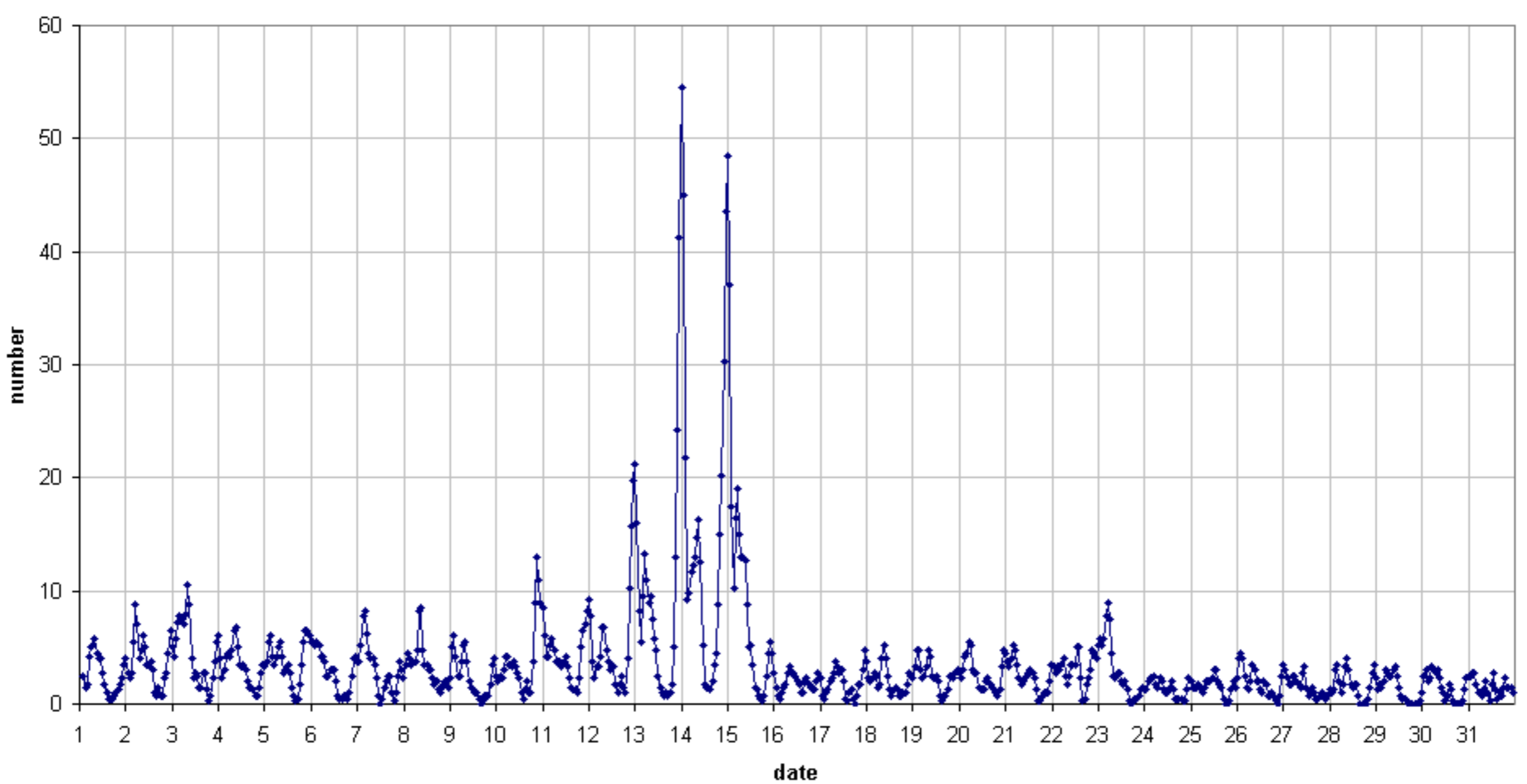
49.99MHz - RadioMeteors December 2019 number of overdense reflections per hour (weighted average) Felix Verbelen (Kampenhout)
