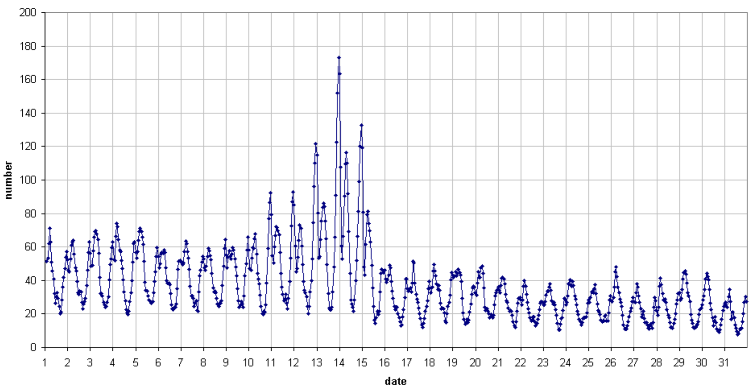
49.99 MHz - RadioMeteors December 2019 number of "all" reflections per hour (weighted average) (automatic count_Mette/5_7Hz) Felix Verbelen (Kampenhout)
