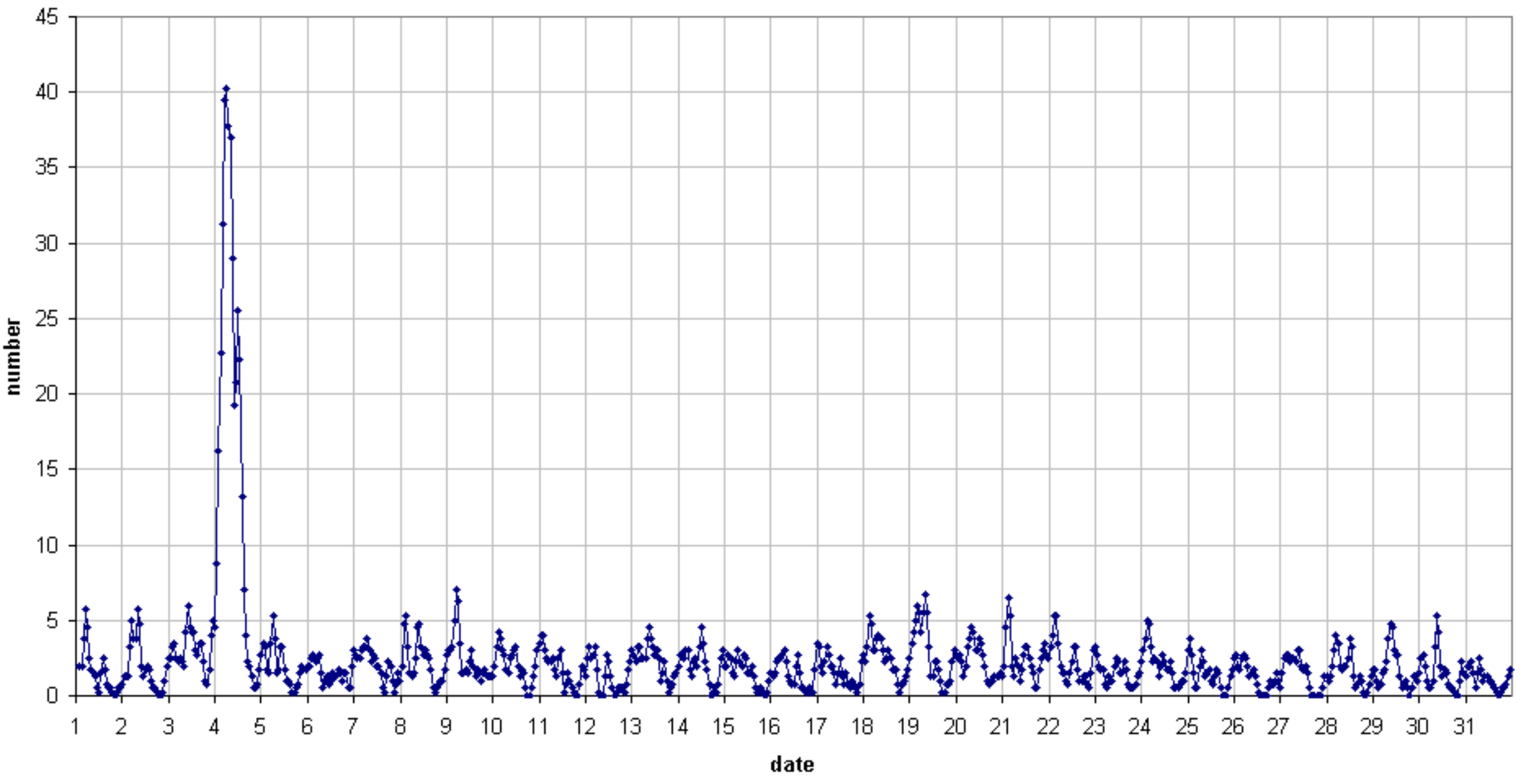
49.99MHz - RadioMeteors January 2020 number of overdense reflections per hour (weighted average) Felix Verbelen (Kampenhout)
