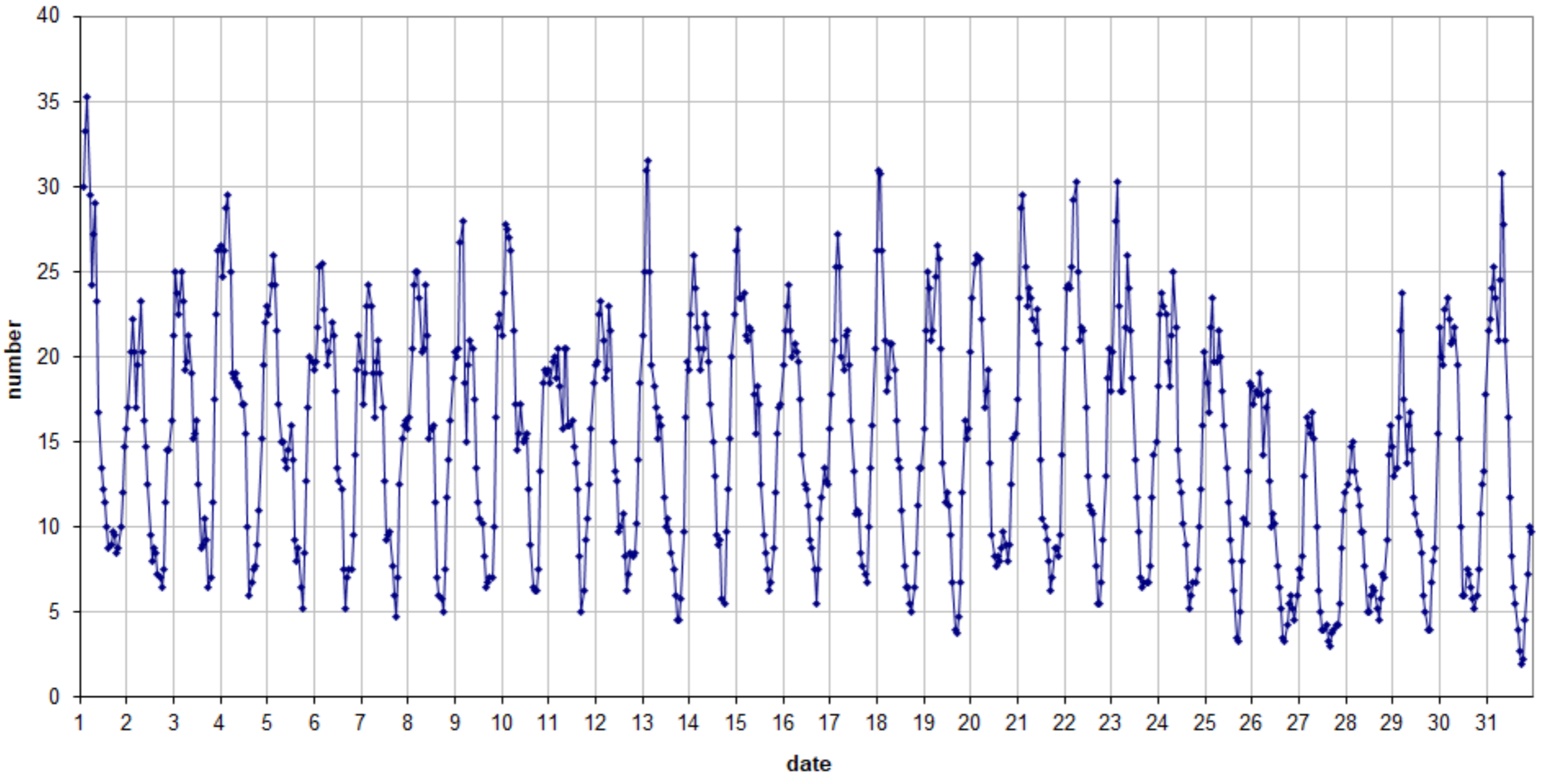
49.99 MHz - RadioMeteors March 2020 number of "all" reflections per hour (weighted average) (automatic count_Mette15_7Hz) Felix Verbelen (Kampenhout)
