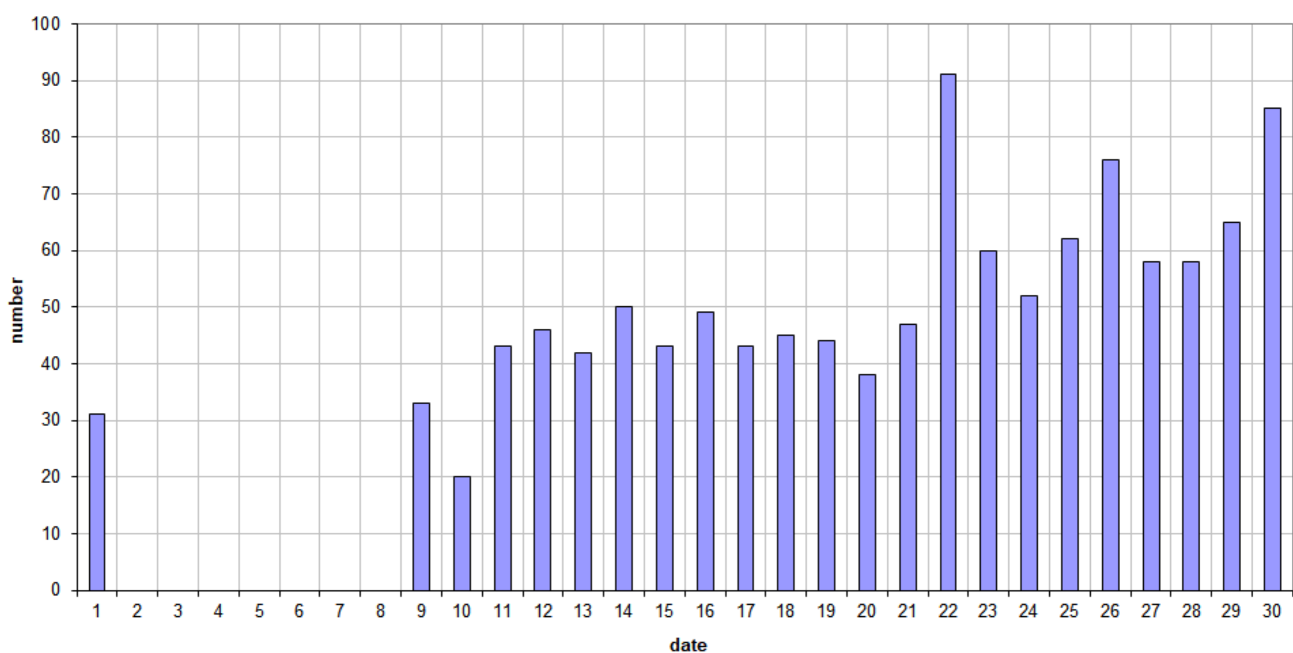
49.99MHz - RadioMeteors April 2020 daily totals of all overdense reflections Felix Verbelen (Kampenhout)
