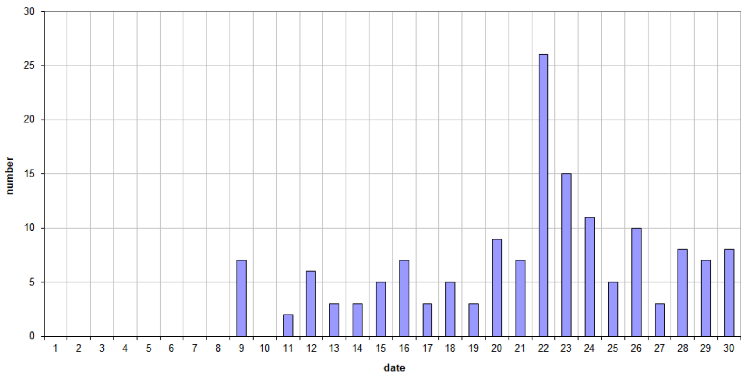
49.99MHz - RadioMeteors April 2020 daily totals of reflections longer than 1 minute Felix Verbelen (Kampenhout)
