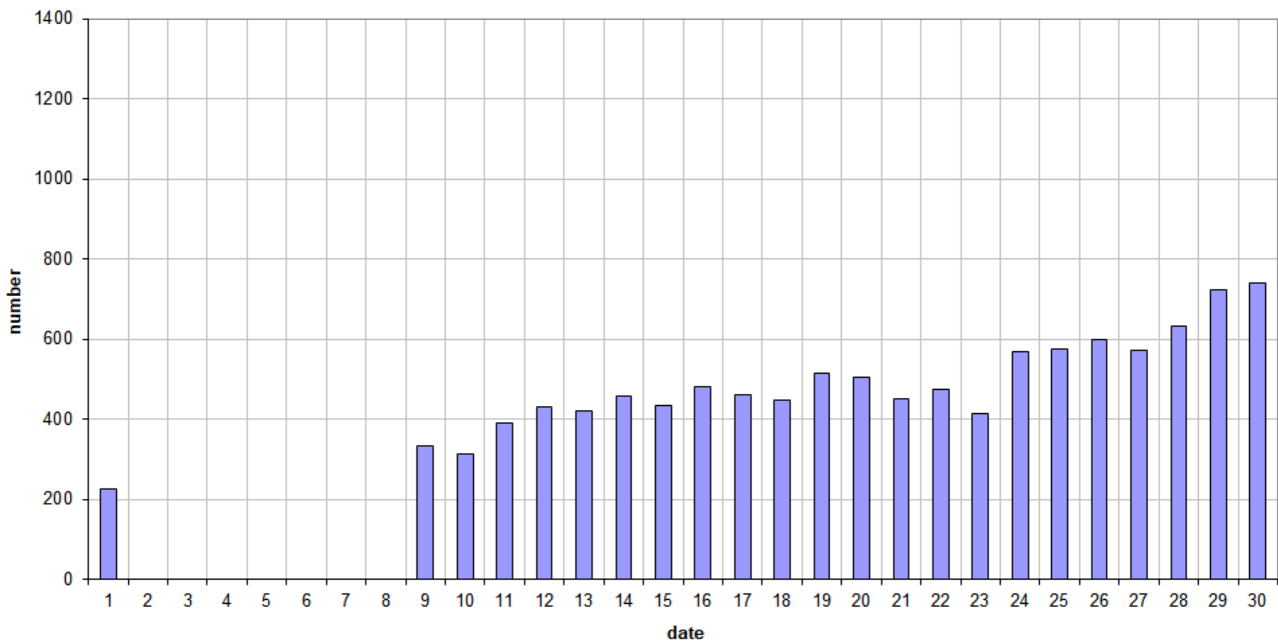
49.99MHz - RadioMeteors April 2020 daily totals of "all" reflections (automatic count_MetteI5_7Hz) Felix Verbelen (Kampenhout)
