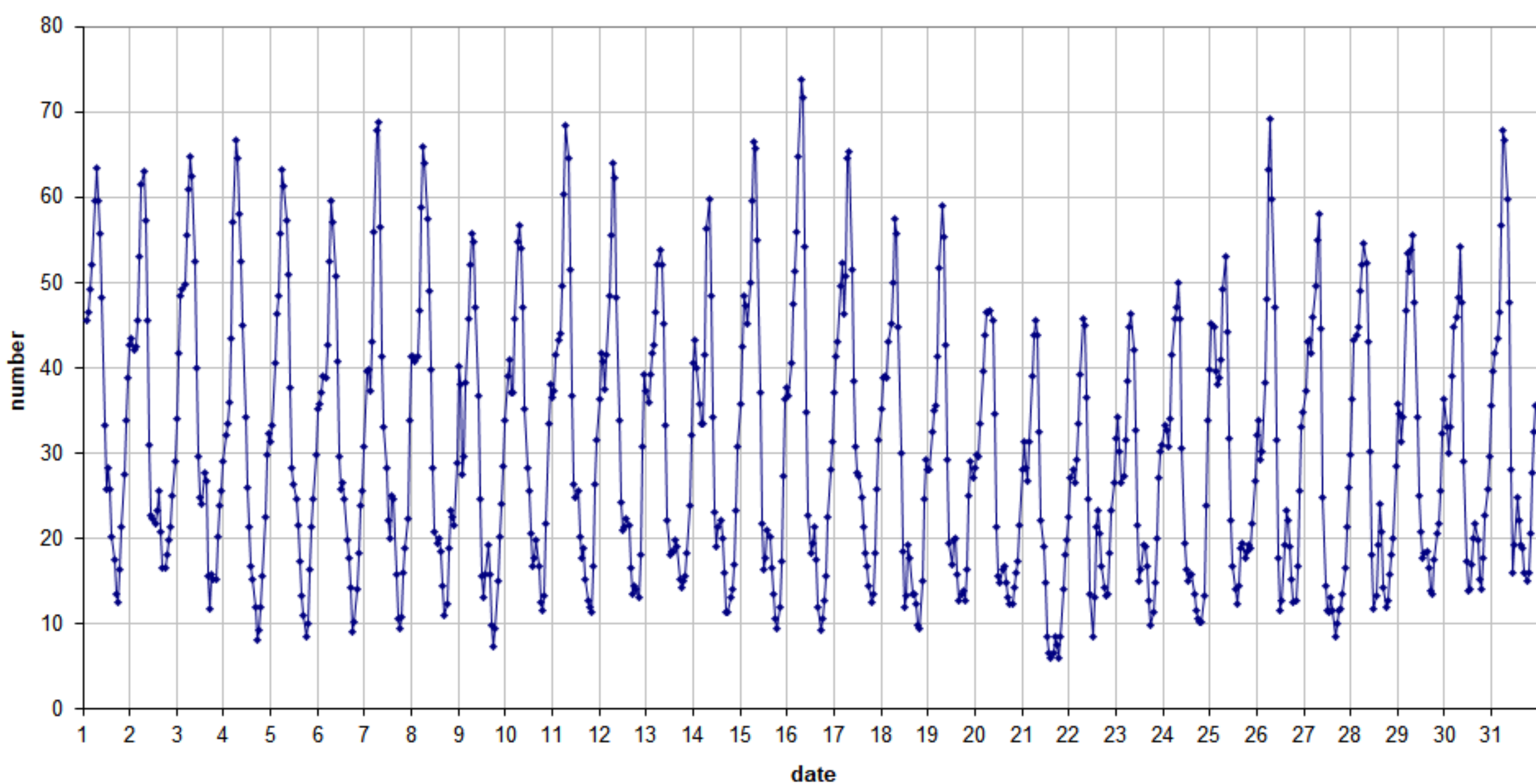
49.99 MHz - RadioMeteors May 2020 number of "all" reflections per hour (weighted average) (automatic count_MetteI5_7Hz) Felix Verbelen (Kamphenhout)
