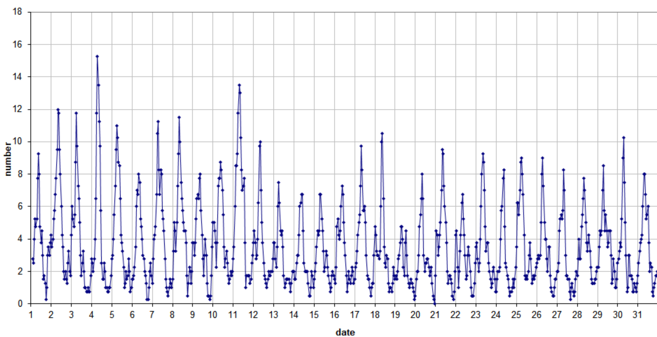
49.99MHz - RadioMeteors May 2020 number of overdense reflections per hour (weighted average) Felix Verbelen (Kamphenhout)
