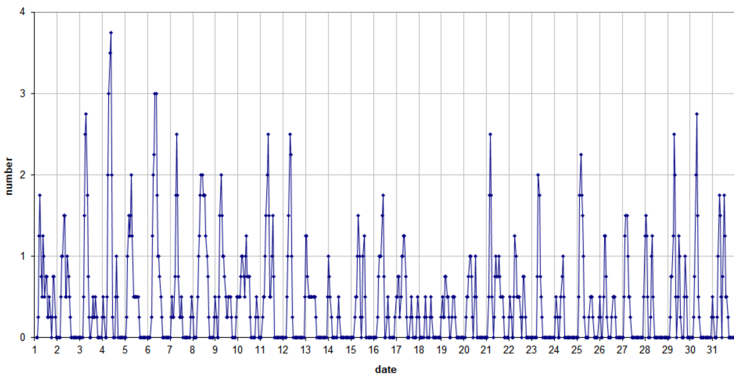
49.99MHz - RadioMeteors May 2020 number of reflections >10 seconds per hour (weighted average) Felix Verbelen (Kamphenhout)
