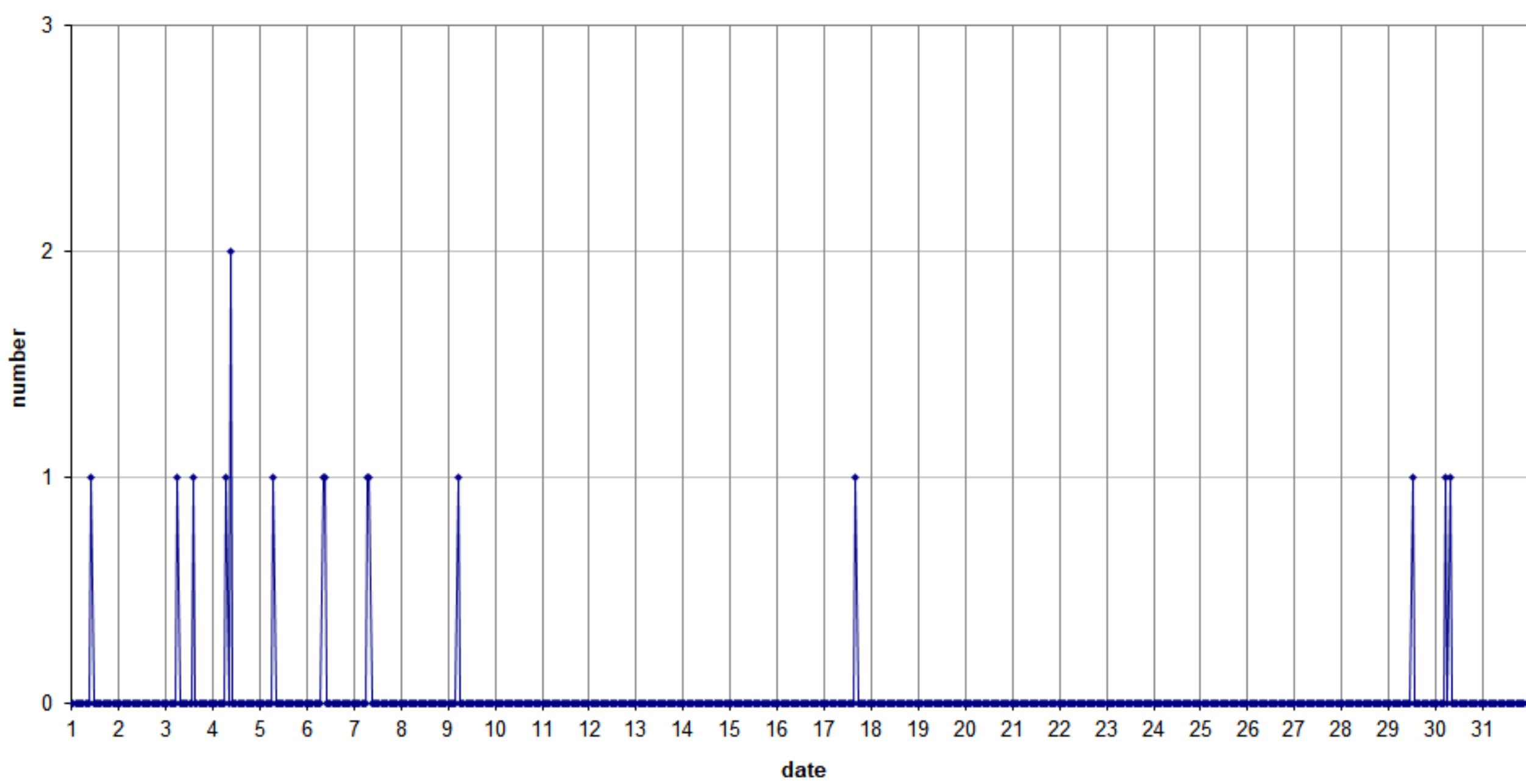
49.99MHz - RadioMeteors May 2020 hourly totals of overdense reflections longer than 1 minute Felix Verbelen (Kamphenhout/BE)
