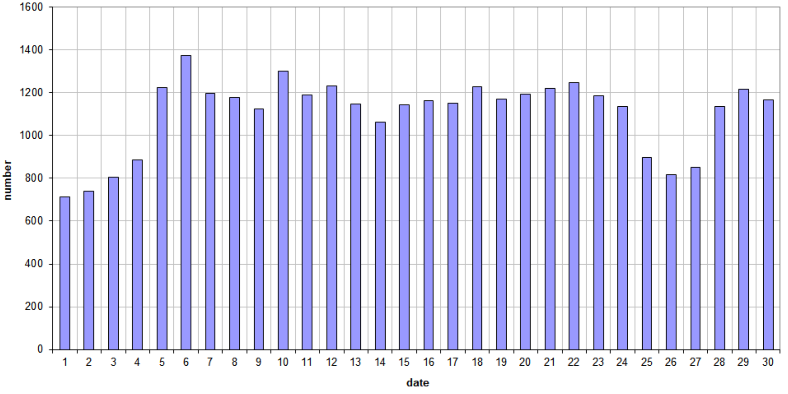
49.99MHz - RadioMeteors June 2020 daily totals of "all" reflections (automatic count_Mettel5_7Hz) Felix Verbelen (Kamphenhout)
