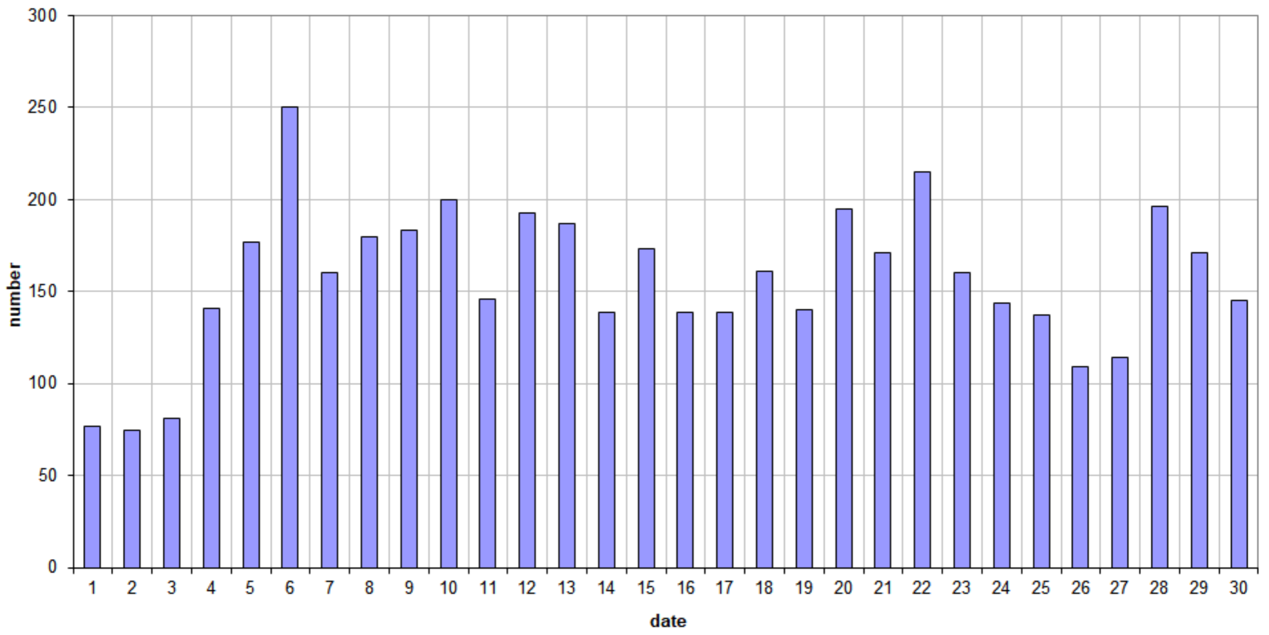
49.99MHz - RadioMeteors June 2020 daily totals of all overdense reflections Felix Verbelen (Kamphenhout)
