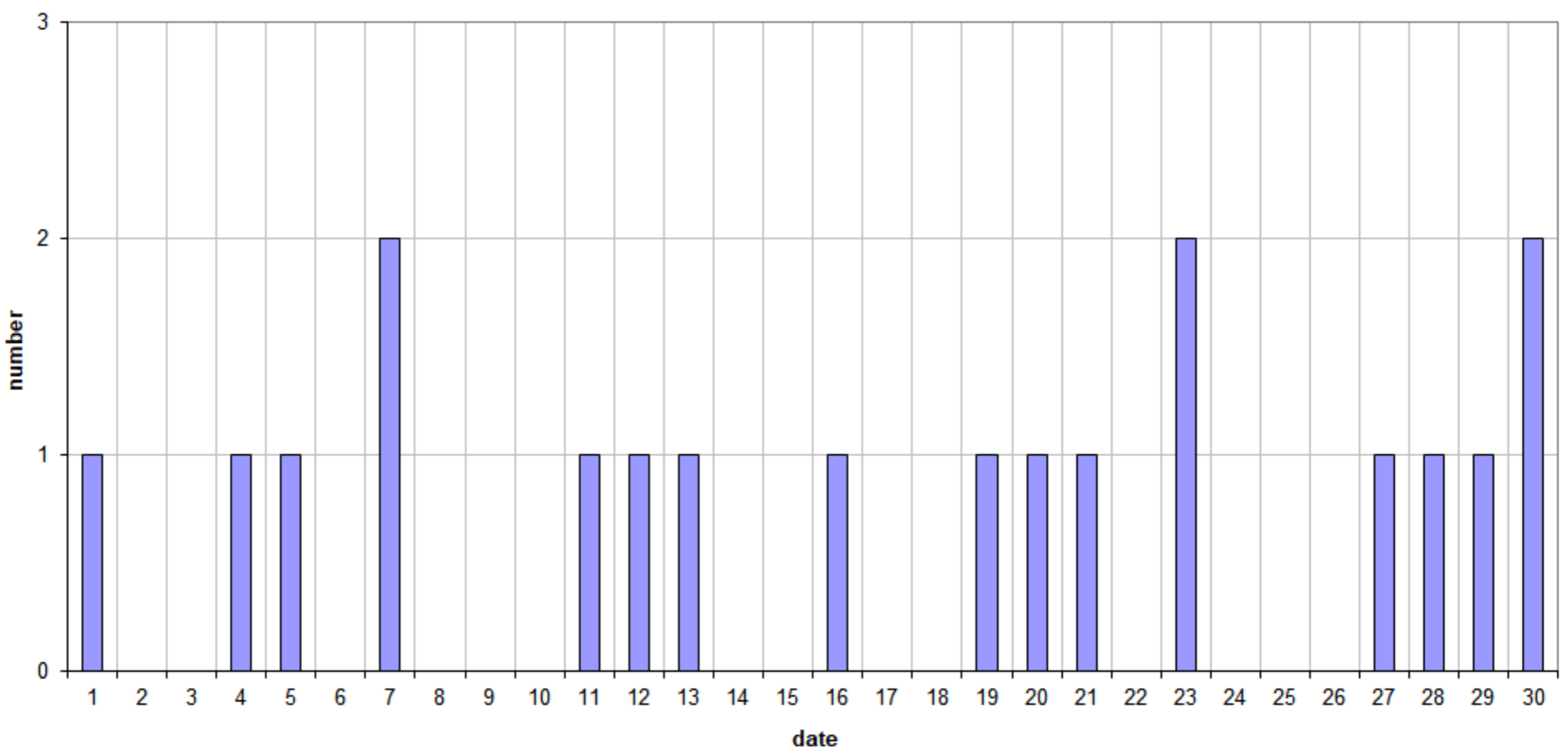
49.99MHz - RadioMeteors June 2020 daily totals of reflections longer than 1 minute Felix Verbelen (Kamphenhout)
