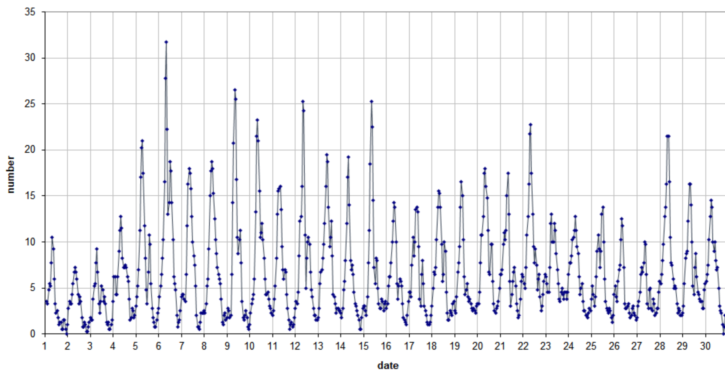
49.99MHz - RadioMeteors June 2020 number of overdense reflections per hour (weighted average) Felix Verbelen (Kamphenhout)
