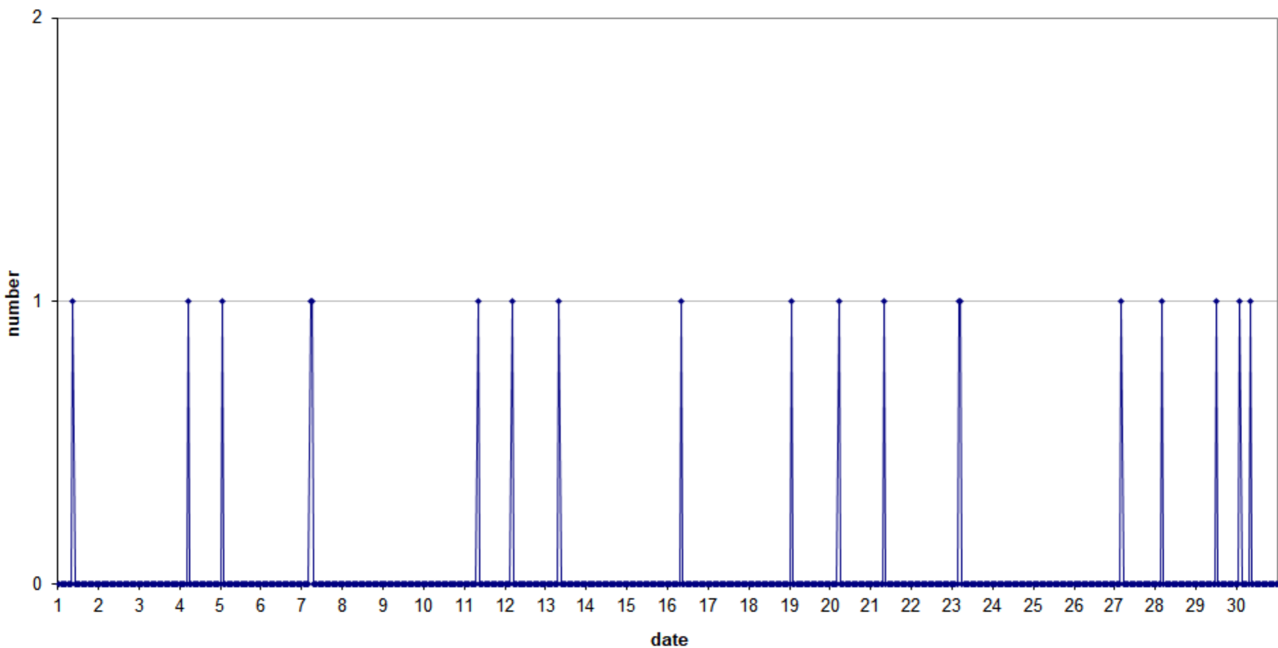
49.99MHz - RadioMeteors June 2020 hourly totals of overdense reflections longer than 1 minute Felix Verbelen (Kamphenhout/BE)
