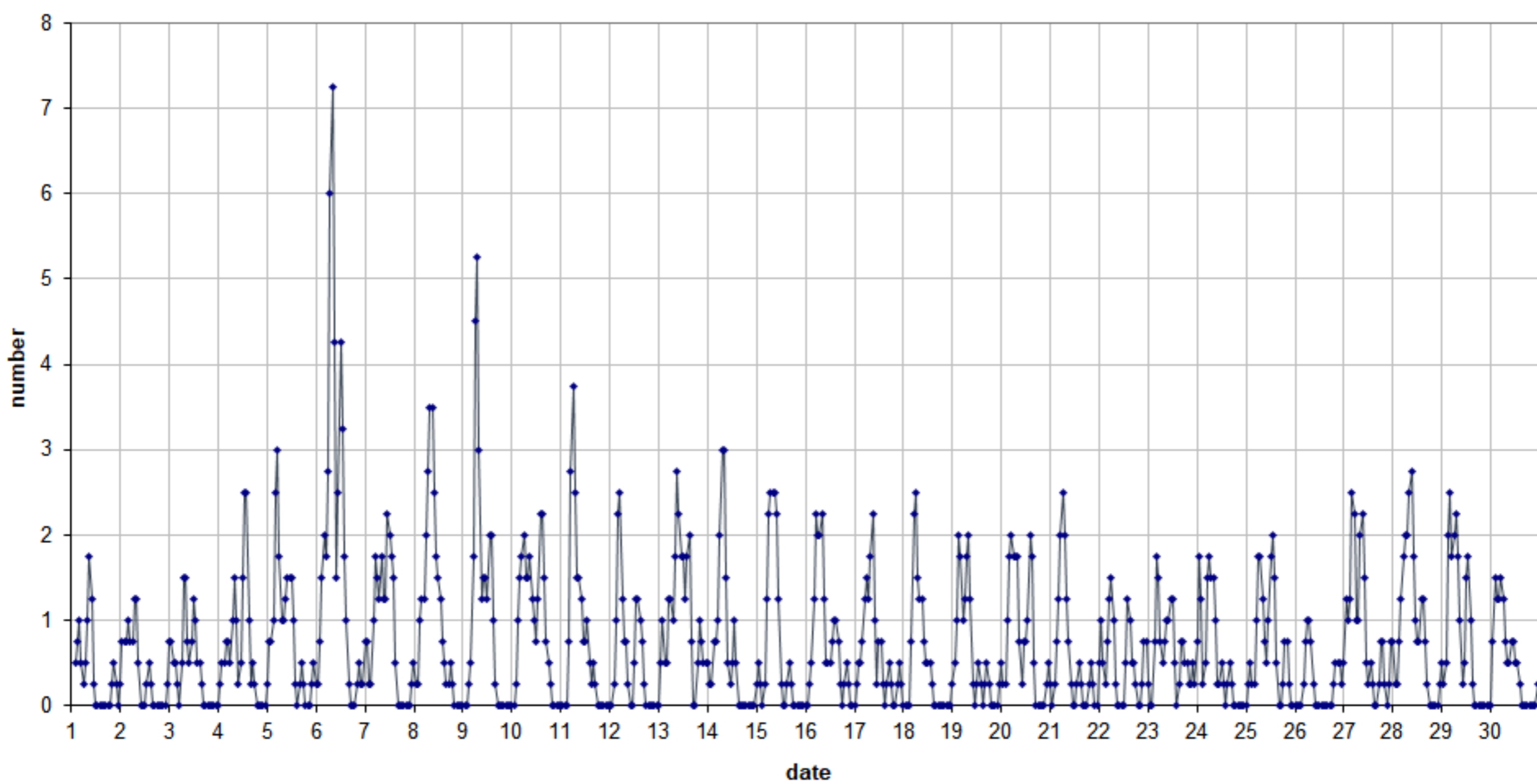
49.99MHz - RadioMeteors June 2020 number of reflections >10 seconds per hour (weighted average) Felix Verbelen (Kamphenhout)
