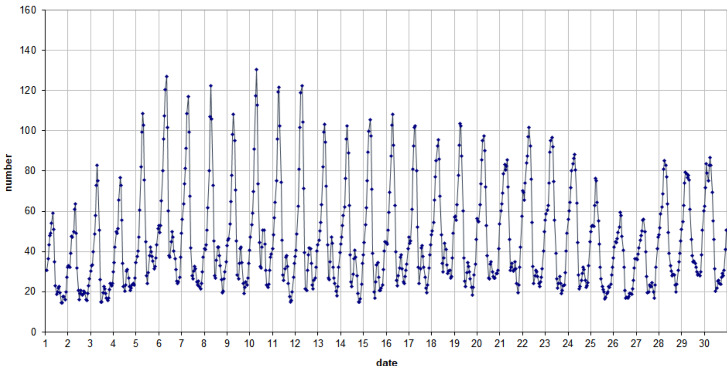
49.99 MHz - RadioMeteors June 2020 number of "all" reflections per hour (weighted average) (automatic count_Mette15_7Hz) Felix Verbelen (Kamphenhout)
