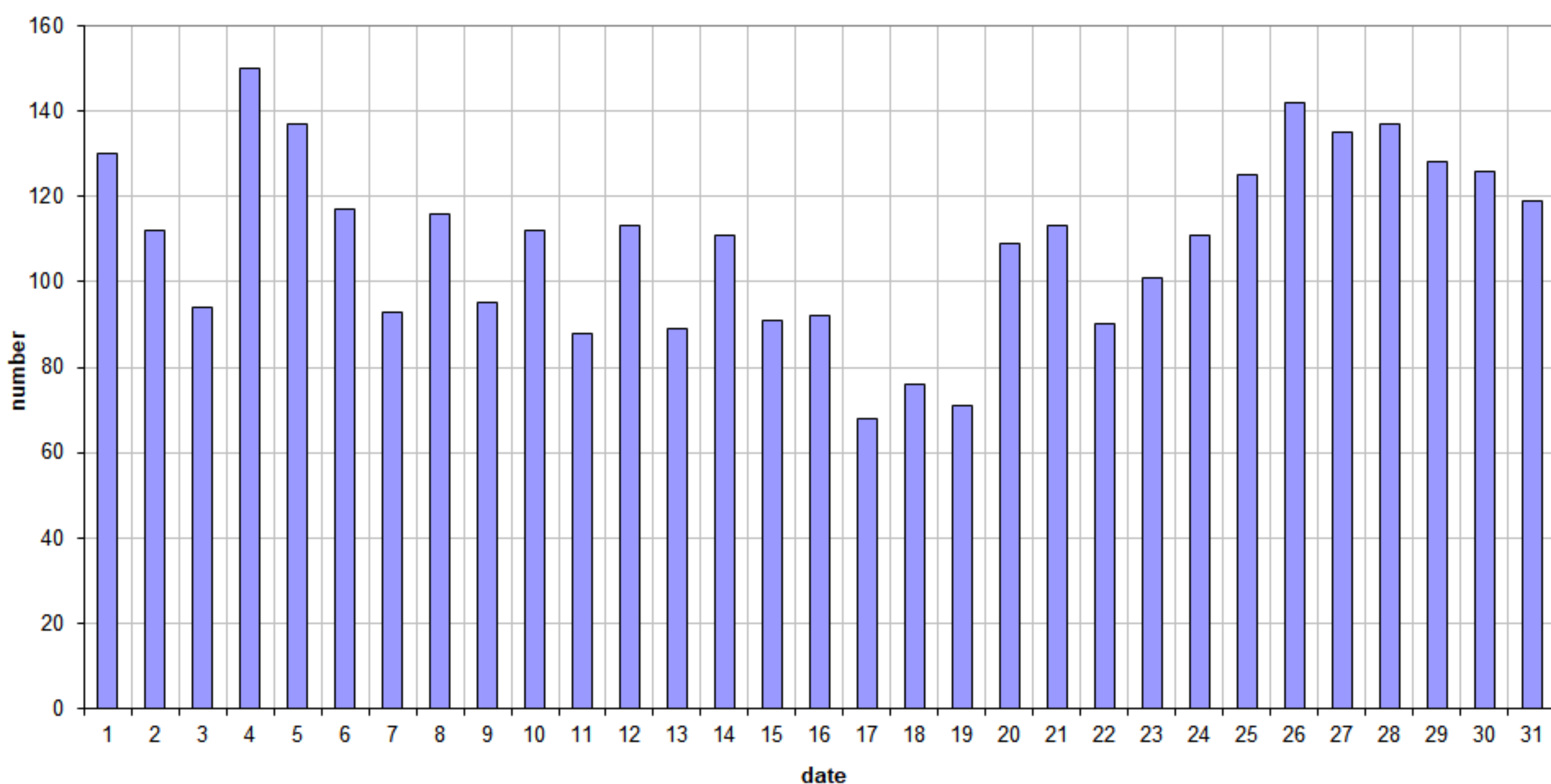
49.99MHz - RadioMeteors July 2020 daily totals of all overdense reflections Felix Verbelen (Kampenhout)
