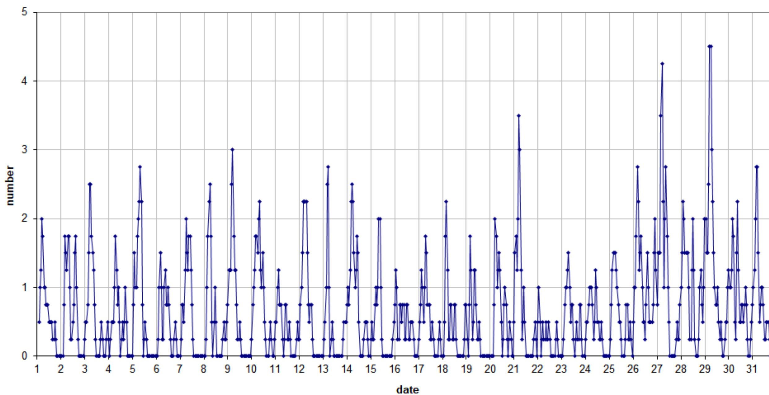
49.99MHz - RadioMeteors July 2020 number of reflections >10 seconds per hour (weighted average) Felix Verbelen (Kamphenhout)
