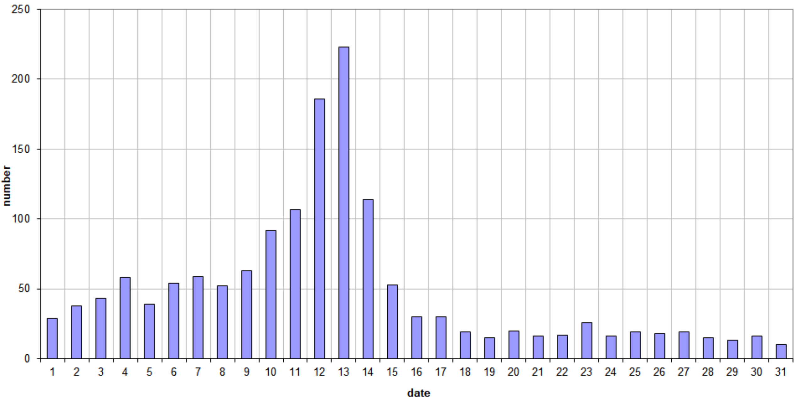
49.99MHz - RadioMeteors August 2020 daily totals of reflections longer than 10 seconds Felix Verbelen (Kamphenhout)
