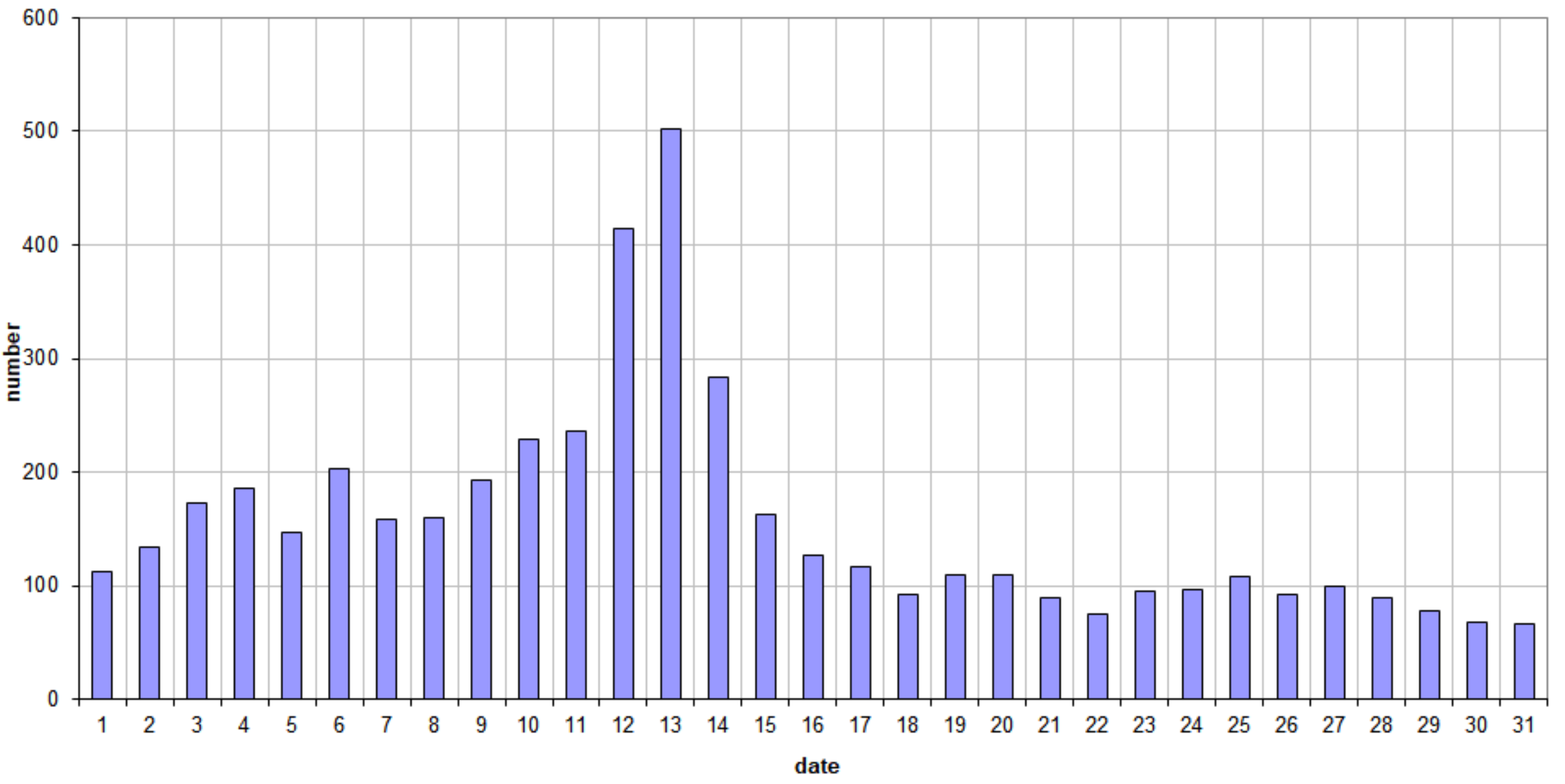
49.99MHz - RadioMeteors August 2020 daily totals of all overdense reflections Felix Verbelen (Kamphenhout)
