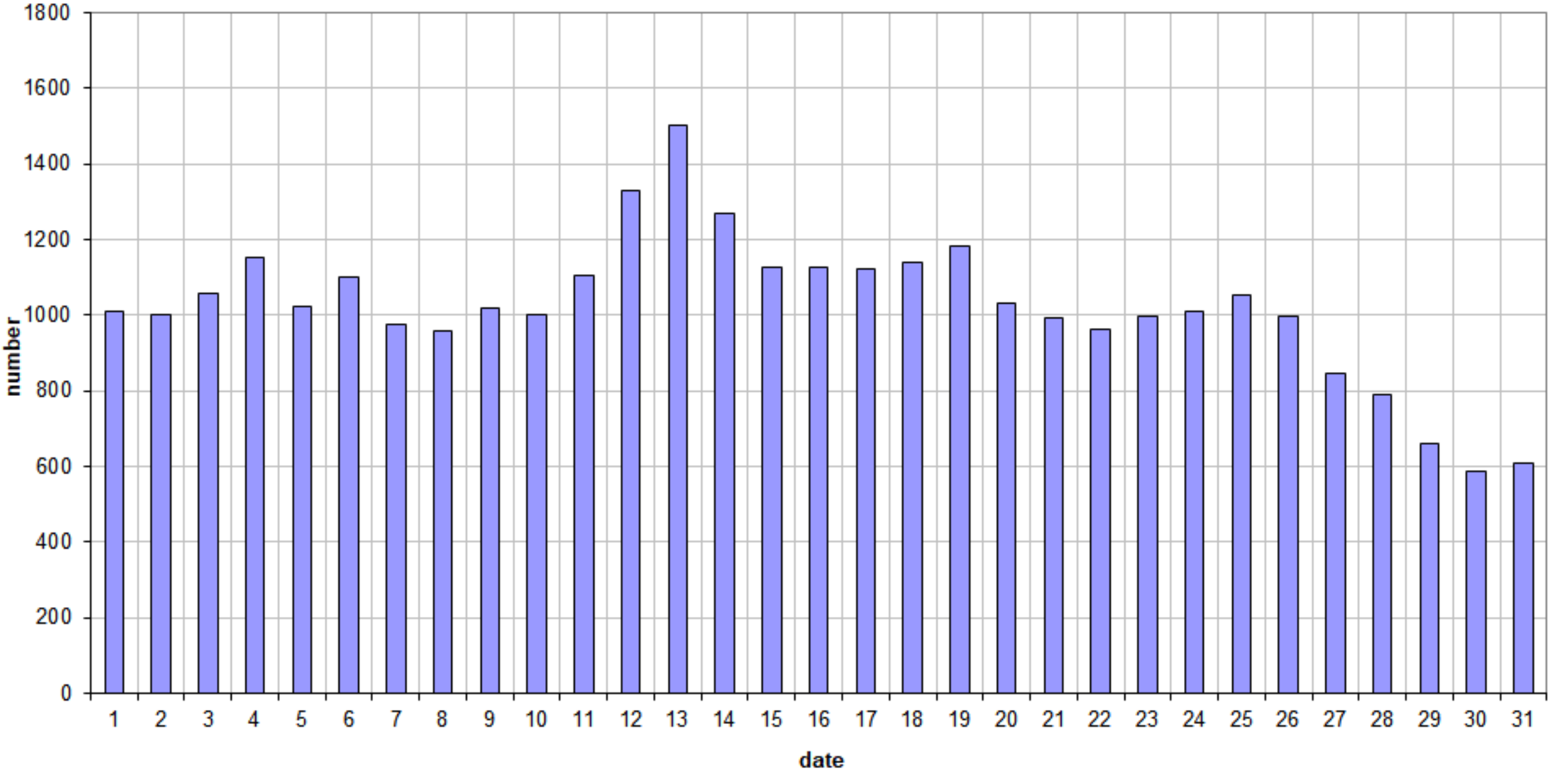
49.99MHz - RadioMeteors August 2020 daily totals of "all" reflections (automatic count_Mettel5_7Hz) Felix Verbelen (Kamphenhout)
