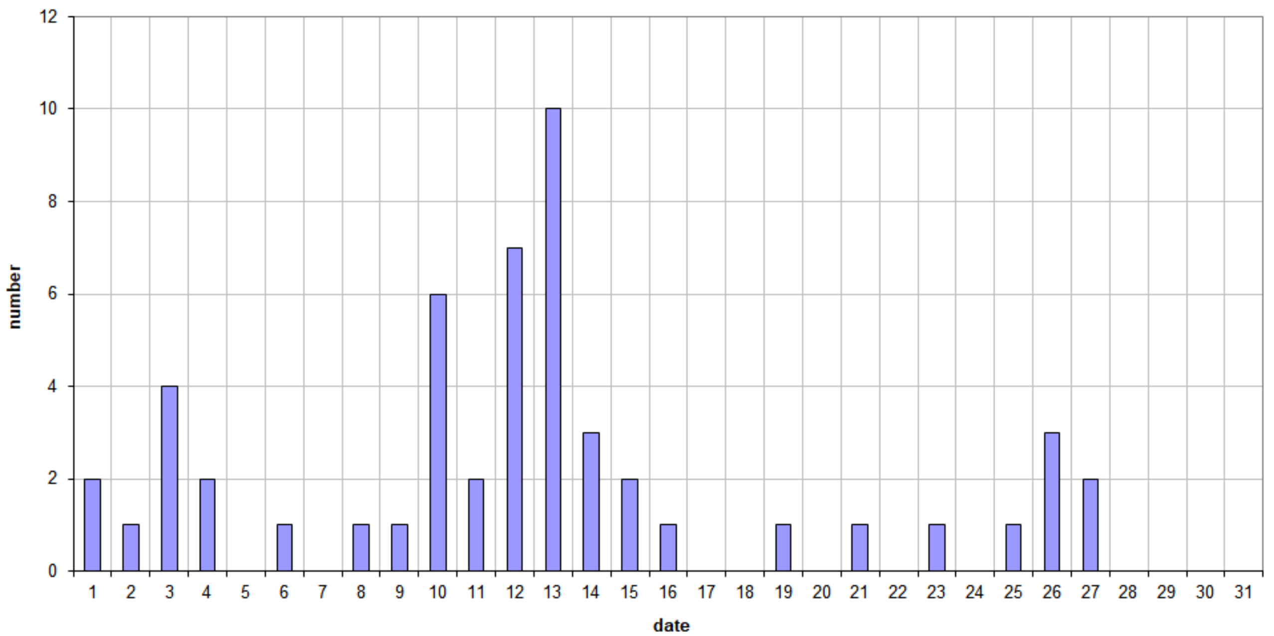
49.99MHz - RadioMeteors August 2020 daily totals of reflections longer than 1 minute Felix Verbelen (Kamphenhout)
