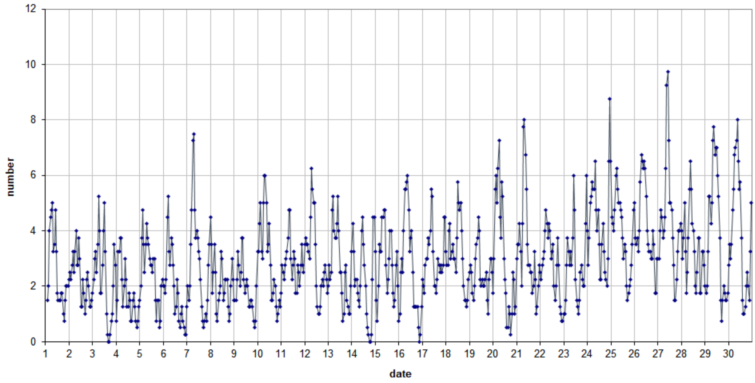
49.99MHz - RadioMeteors September 2020 number of overdense reflections per hour (weighted average) Felix Verbelen (Kampenhout)
