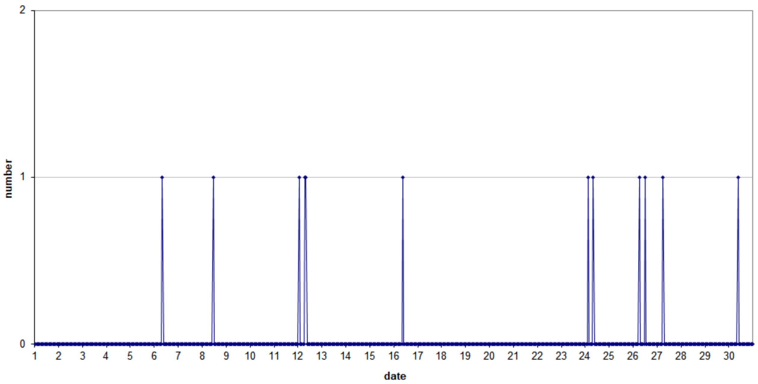
49.99MHz - RadioMeteors September 2020 hourly totals of overdense reflections longer than 1 minute Felix Verbelen (Kampenhout/BE)
