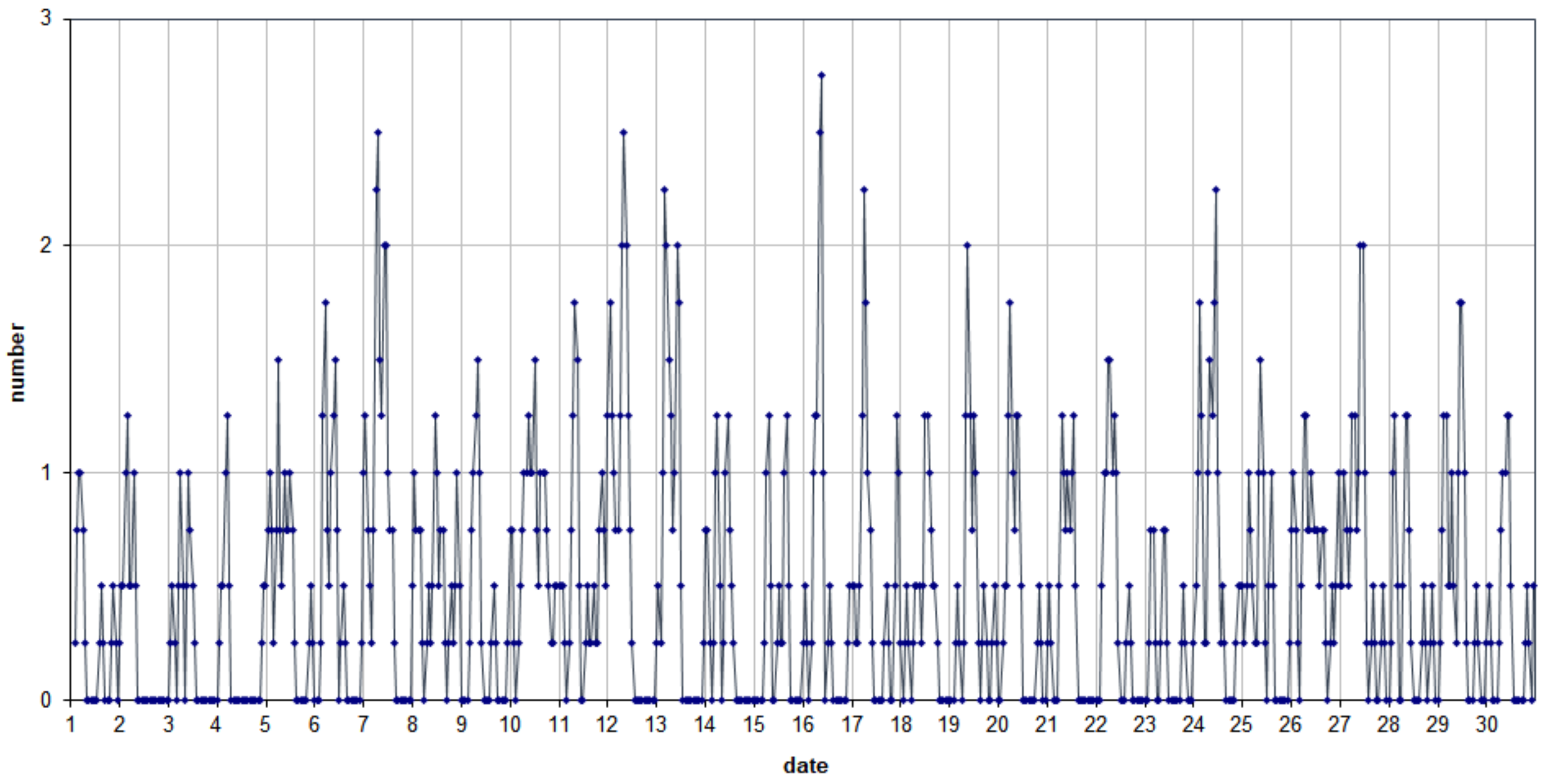
49.99MHz - RadioMeteors September 2020 number of reflections >10 seconds per hour (weighted average) Felix Verbelen (Kampenhout)
