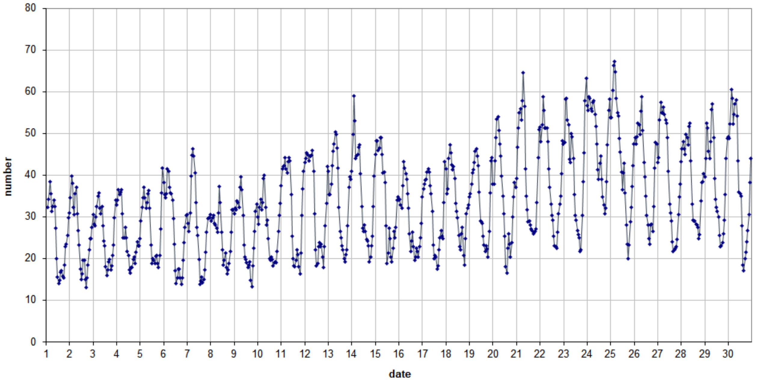
49.99 MHz - RadioMeteors September 2020 number of "all" reflections per hour (weighted average) (automatic count_Mettel5_7Hz) Felix Verbelen (Kampenhout)
