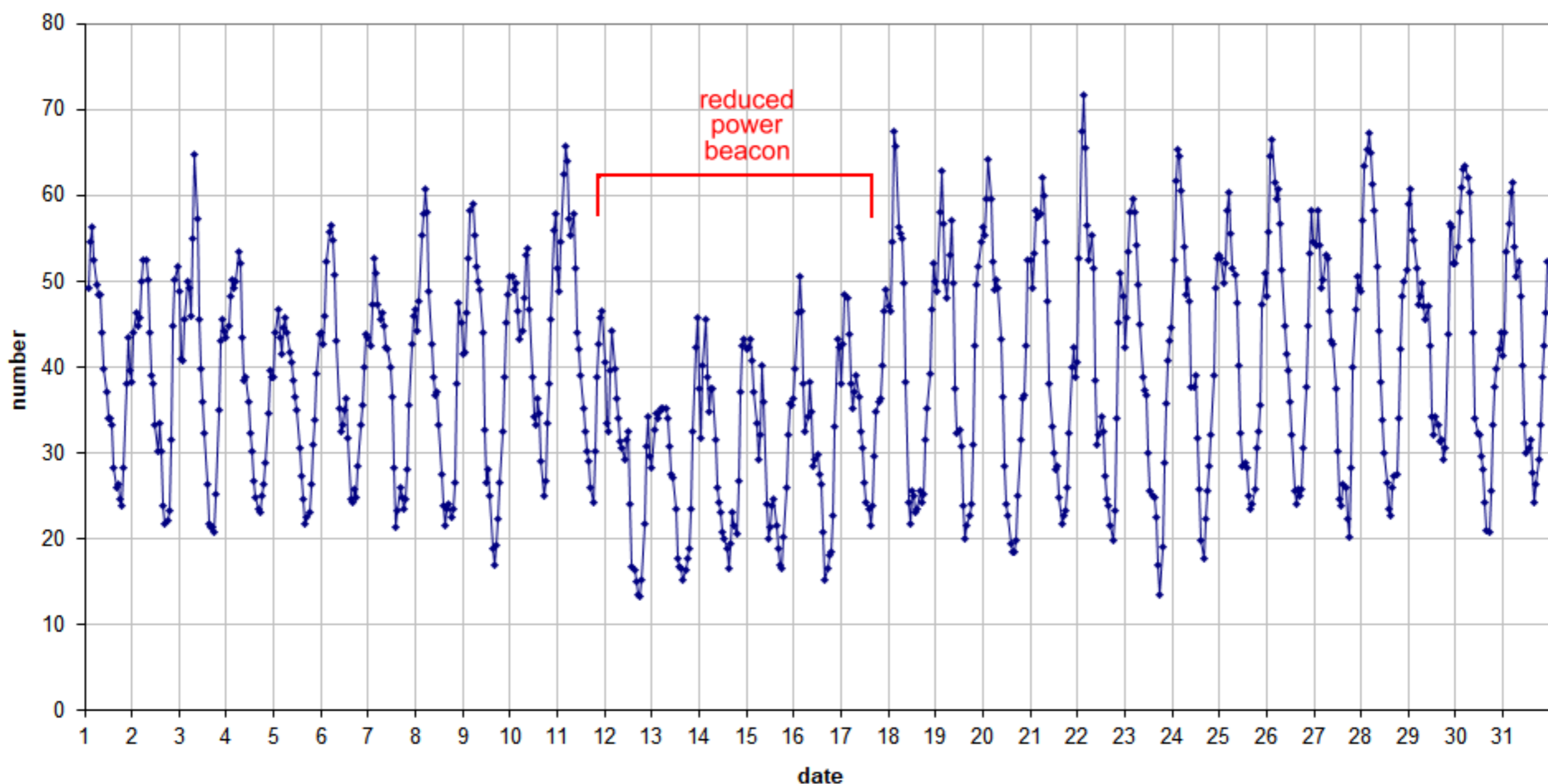
49.99 MHz - RadioMeteors October 2020 number of "all" reflections per hour (weighted average) (automatic count_Mettel5_7Hz) Felix Verbelen (Kamphenhout)
