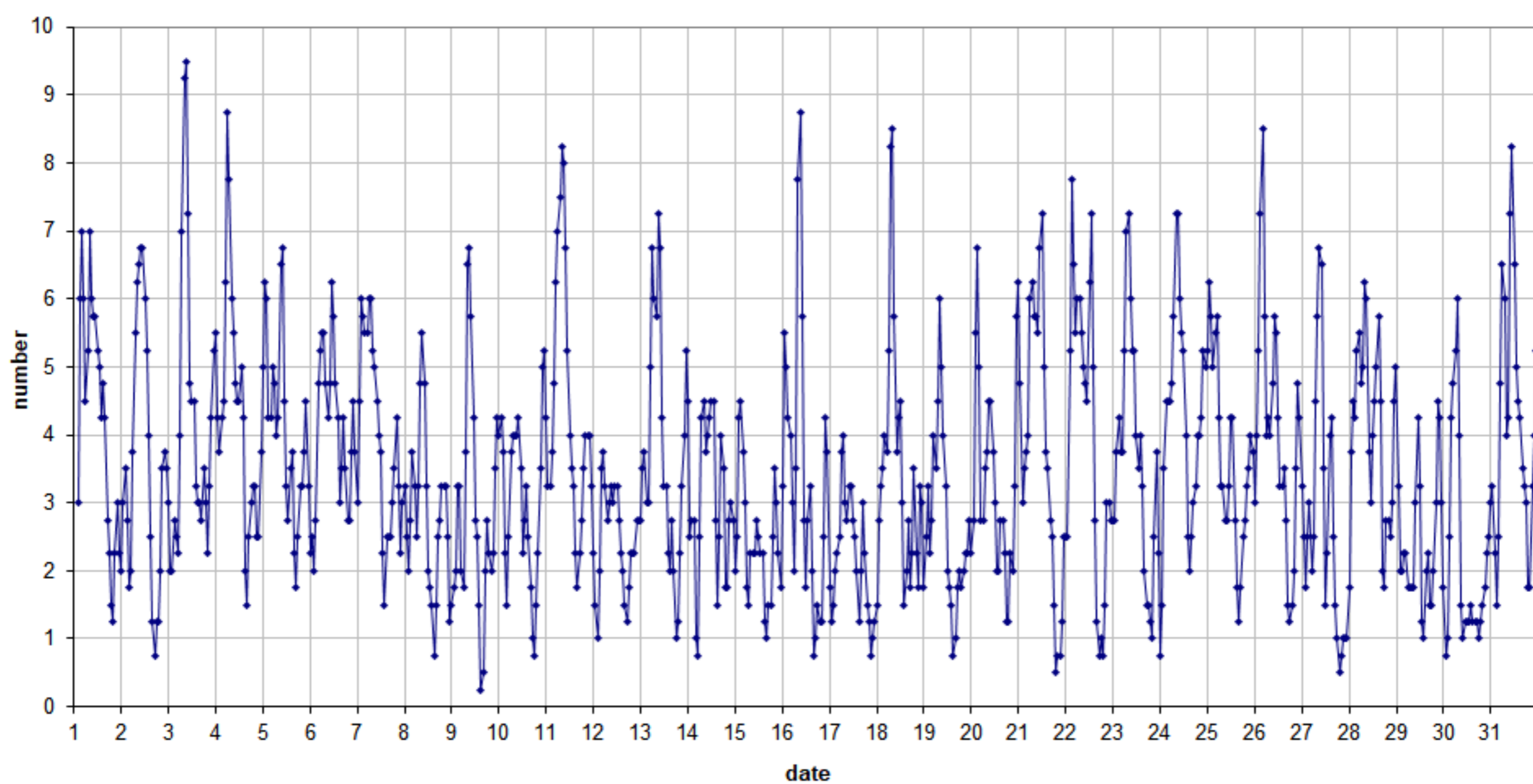
49.99MHz - RadioMeteors October 2020 number of overdense reflections per hour (weighted average) Felix Verbelen (Kamphenhout)
