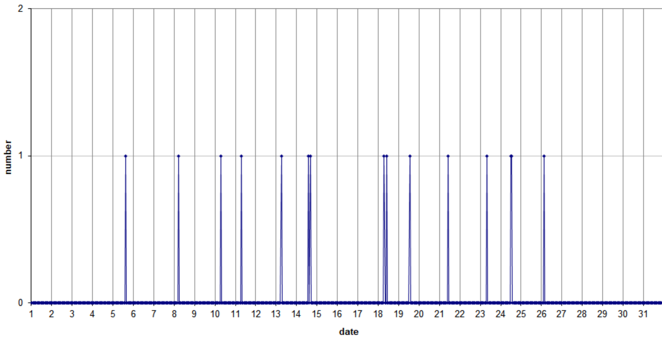
49.99MHz - RadioMeteors October 2020 hourly totals of overdense reflections longer than 1 minute Felix Verbelen (Kamphenhout/BE)
