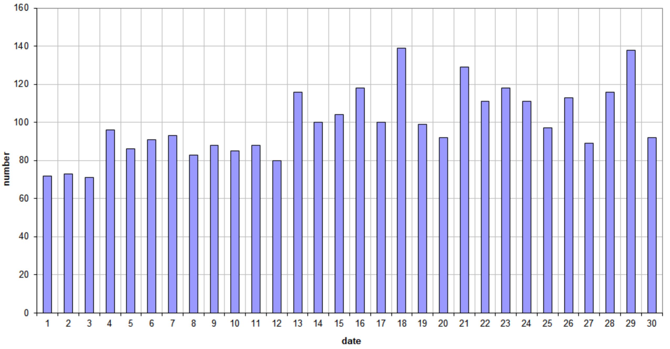
49.99MHz - RadioMeteors November 2020 daily totals of all overdense reflections Felix Verbelen (Kamphenhout)
