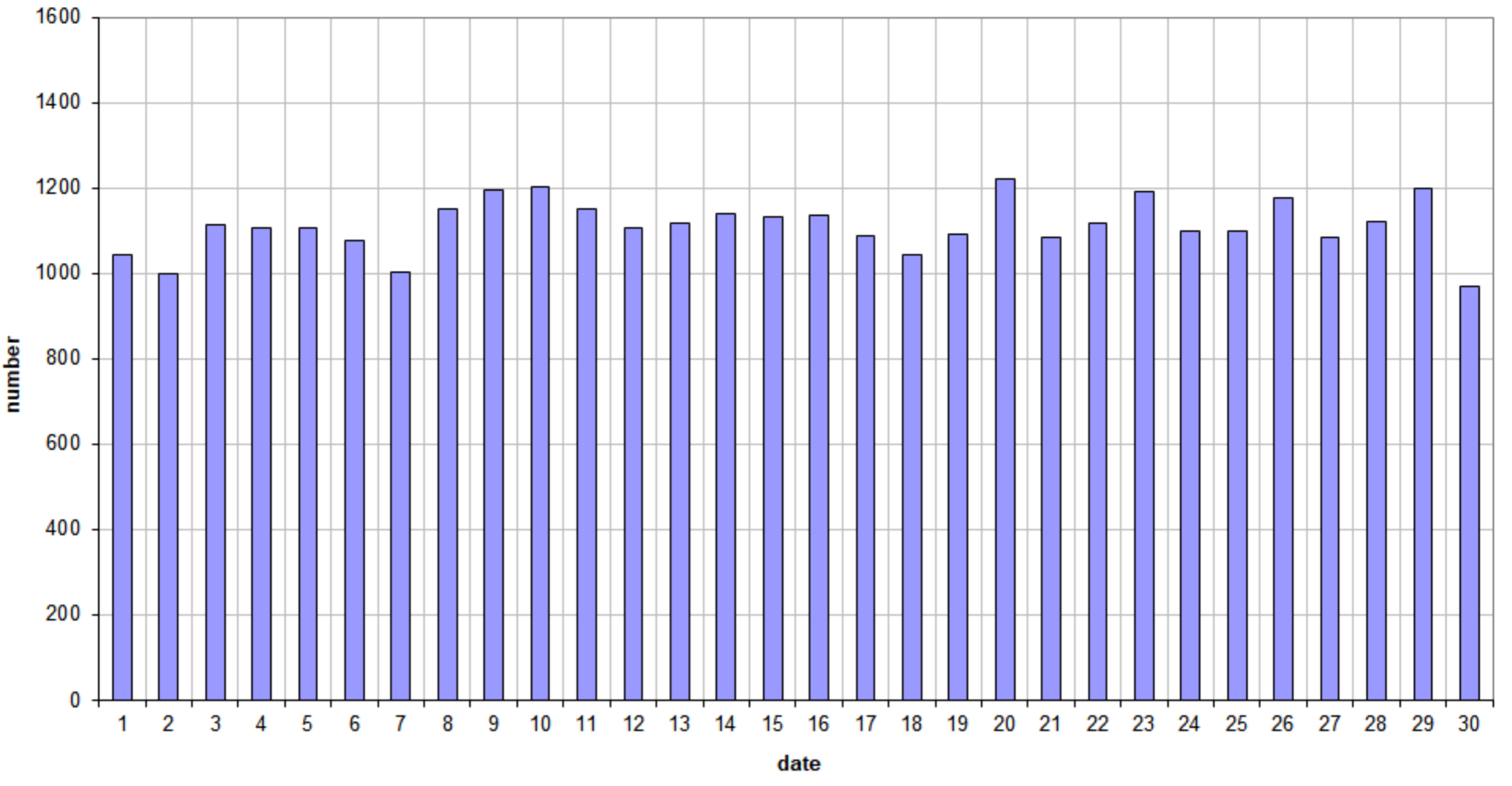
49.99MHz - RadioMeteors November 2020 daily totals of "all" reflections (automatic count_Mettel5_7Hz) Felix Verbelen (Kamphenhout)
