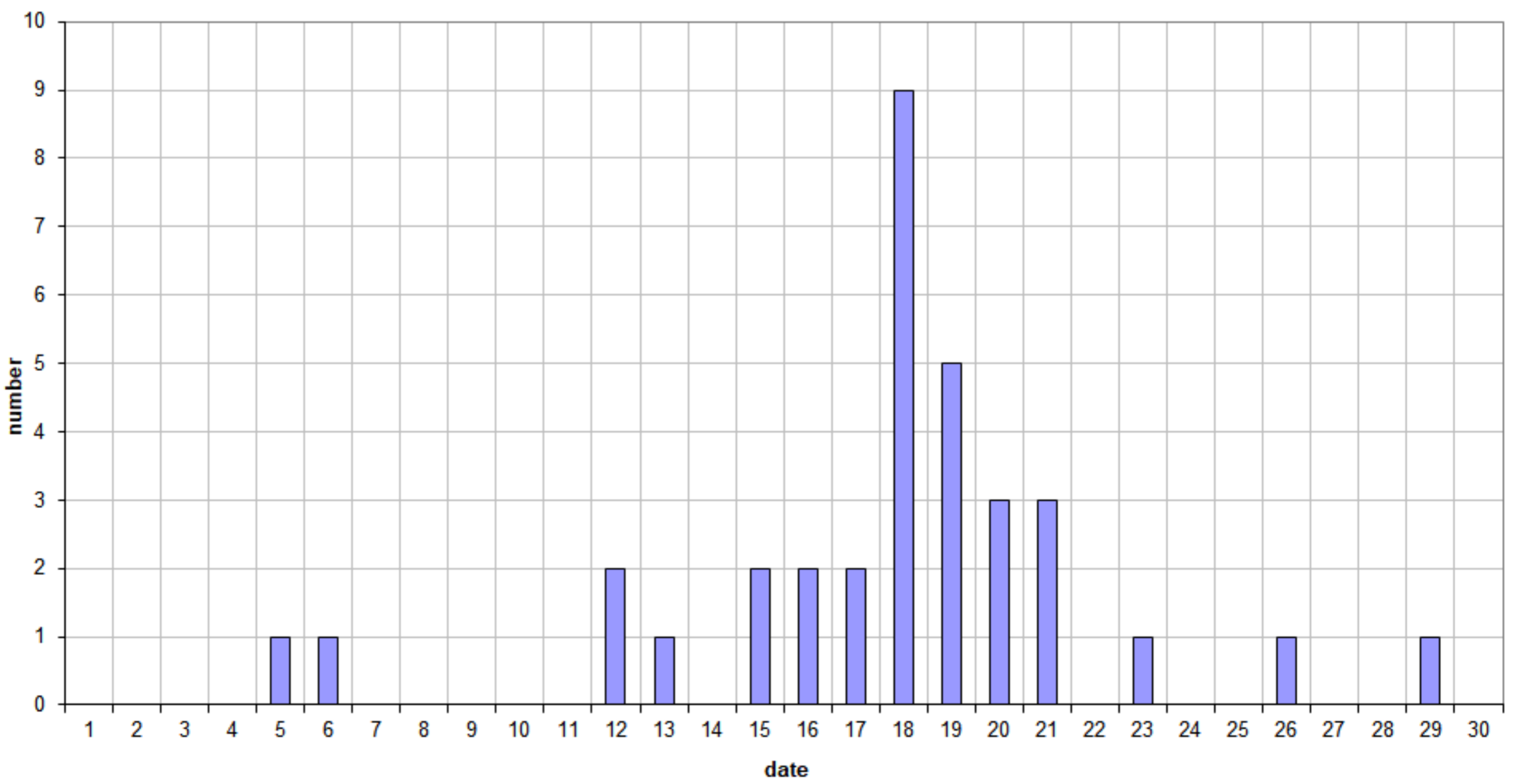
49.99MHz - RadioMeteors November 2020 daily totals of reflections longer than 1 minute Felix Verbelen (Kamphenhout)
