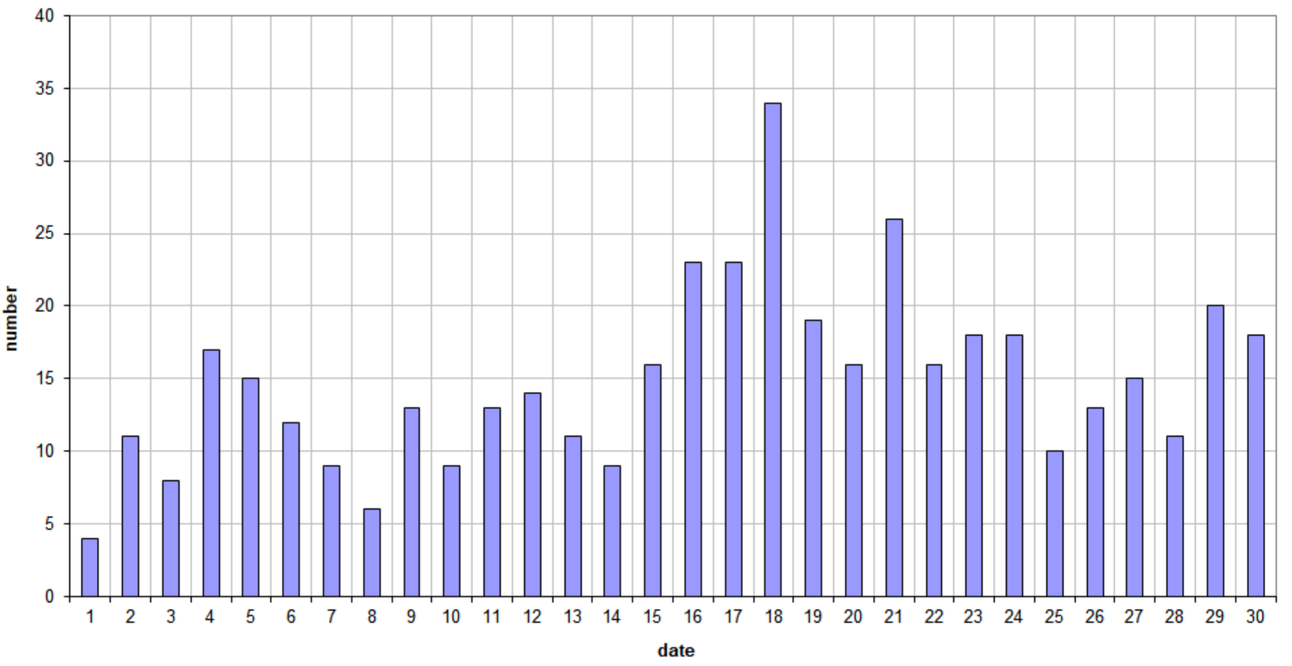
49.99MHz - RadioMeteors November 2020 daily totals of reflections longer than 10 seconds Felix Verbelen (Kamphenhout)
