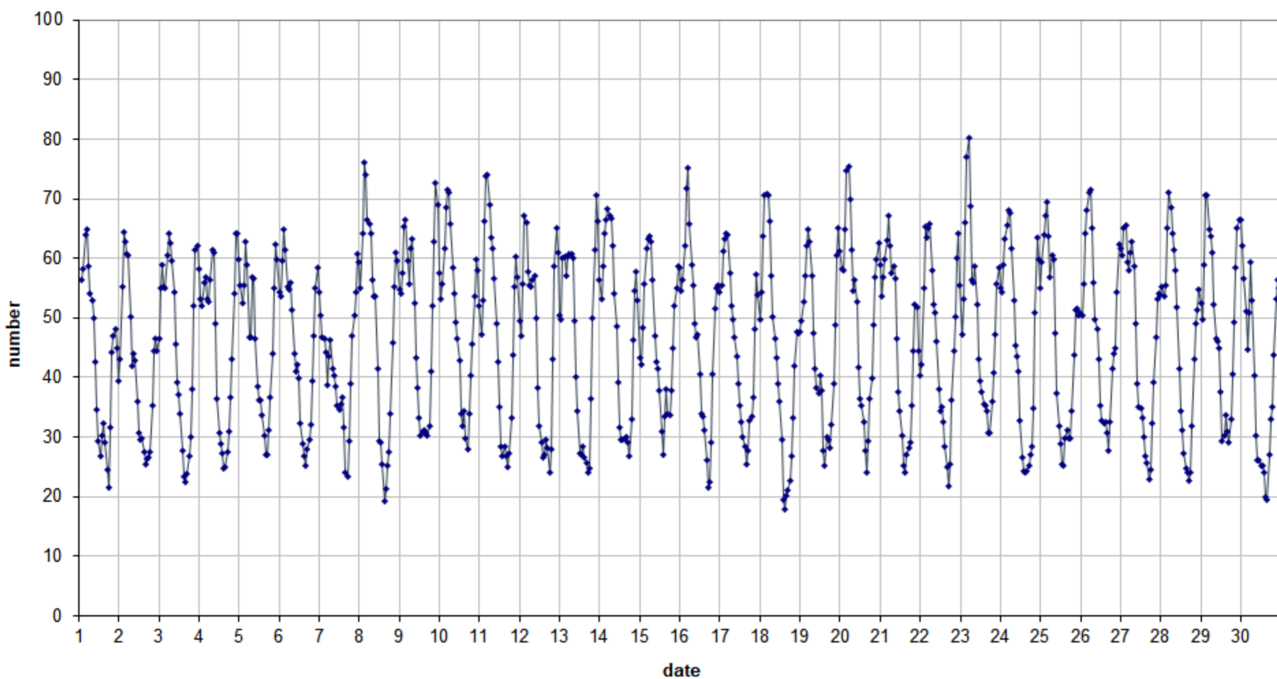
49.99 MHz - RadioMeteors November 2020 number of "all" reflections per hour (weighted average) (automatic count_Mette15_7Hz) Felix Verbelen (Kampenhout)
