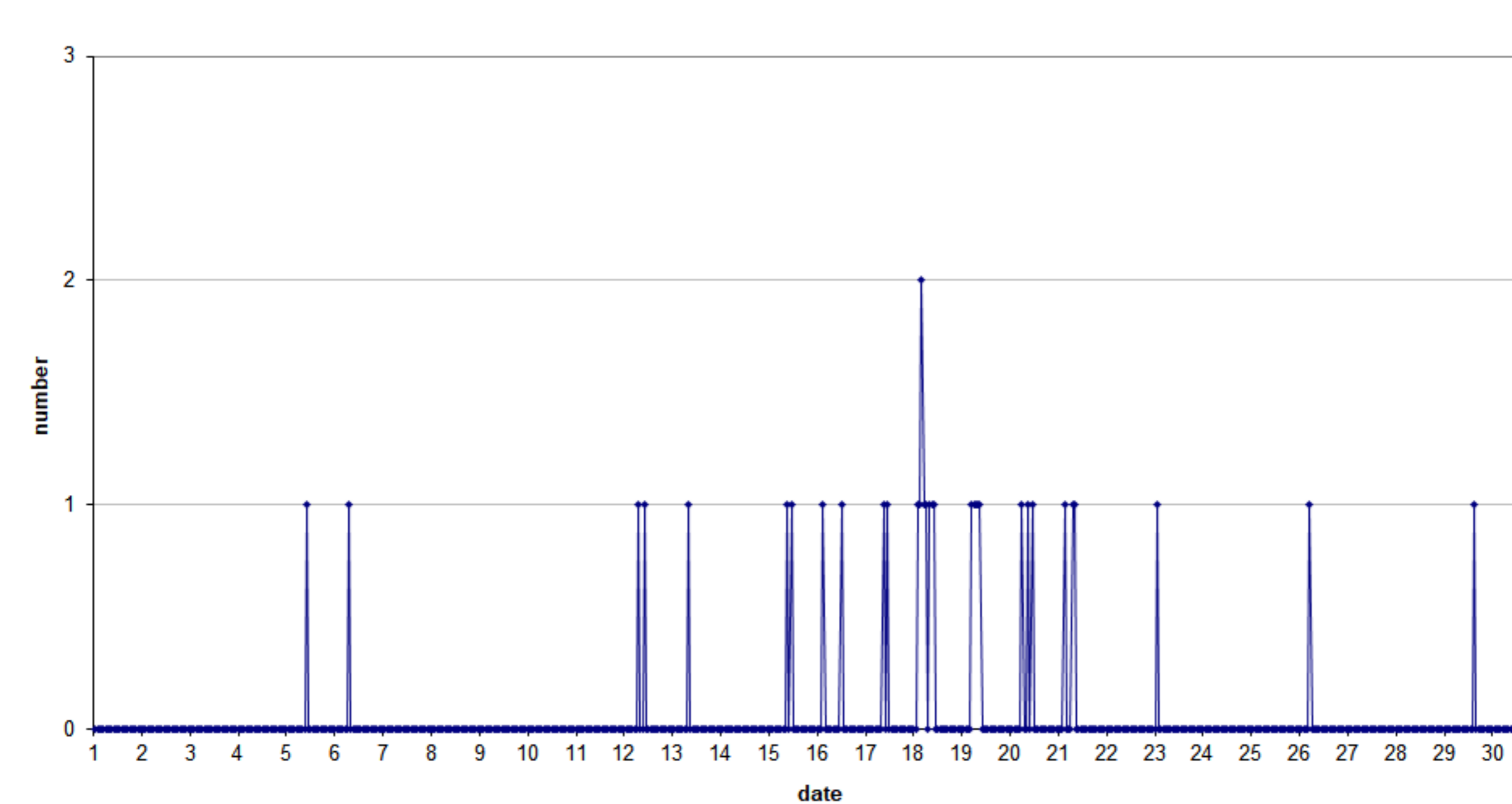
49.99MHz - RadioMeteors November 2020 hourly totals of overdense reflections longer than 1 minute Felix Verbelen (Kampenhout/BE)
