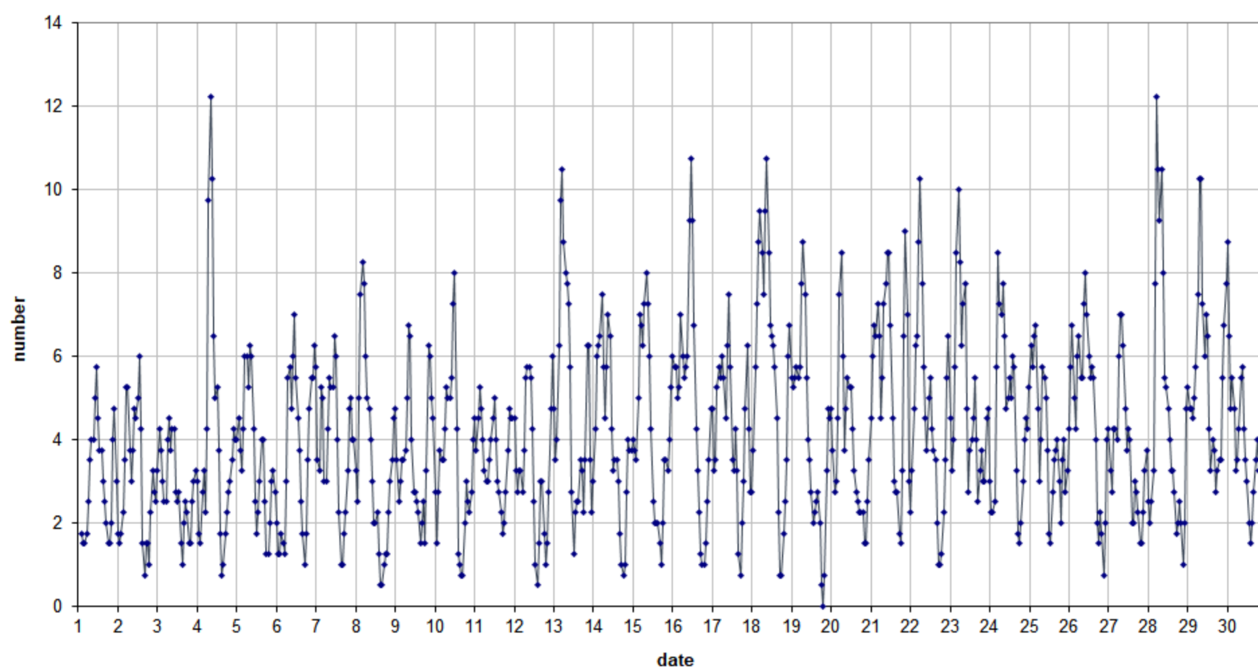
49.99MHz - RadioMeteors November 2020 number of overdense reflections per hour (weighted average) Felix Verbelen (Kampenhout)
