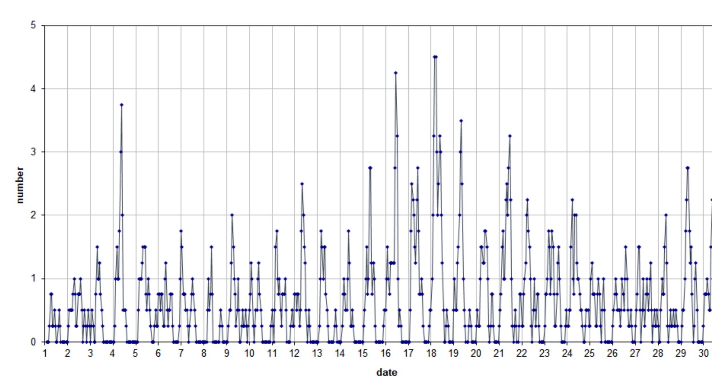
49.99MHz - RadioMeteors November 2020 number of reflections >10 seconds per hour (weighted average) Felix Verbelen (Kampenhout)
