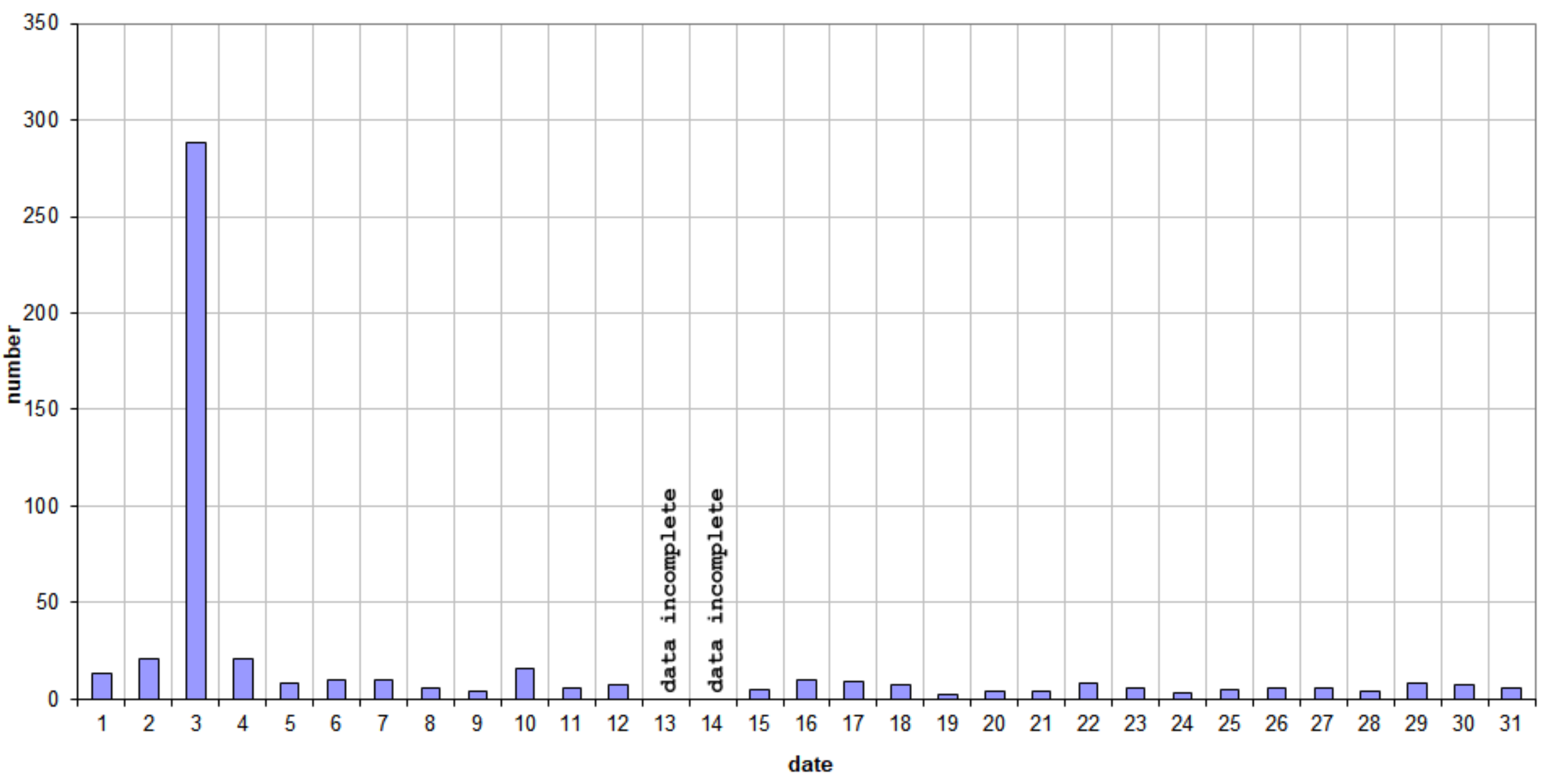
49.99MHz - RadioMeteors January 2021 daily totals of reflections longer than 10 seconds Felix Verbelen (Kamphenhout)
