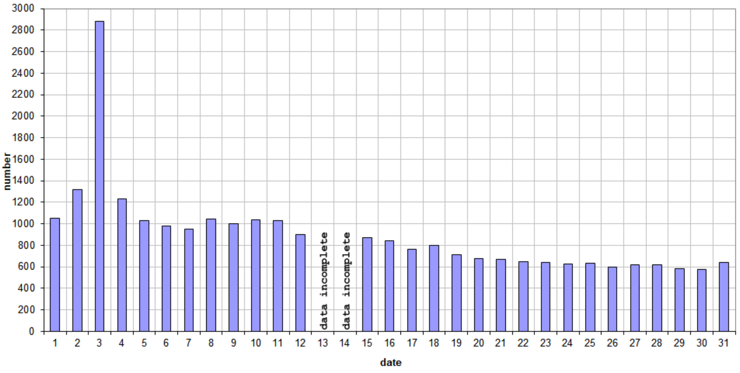
49.99MHz - RadioMeteors January 2021 daily totals of "all" reflections (automatic count_Mettel5_7Hz) Felix Verbelen (Kamphenhout)
