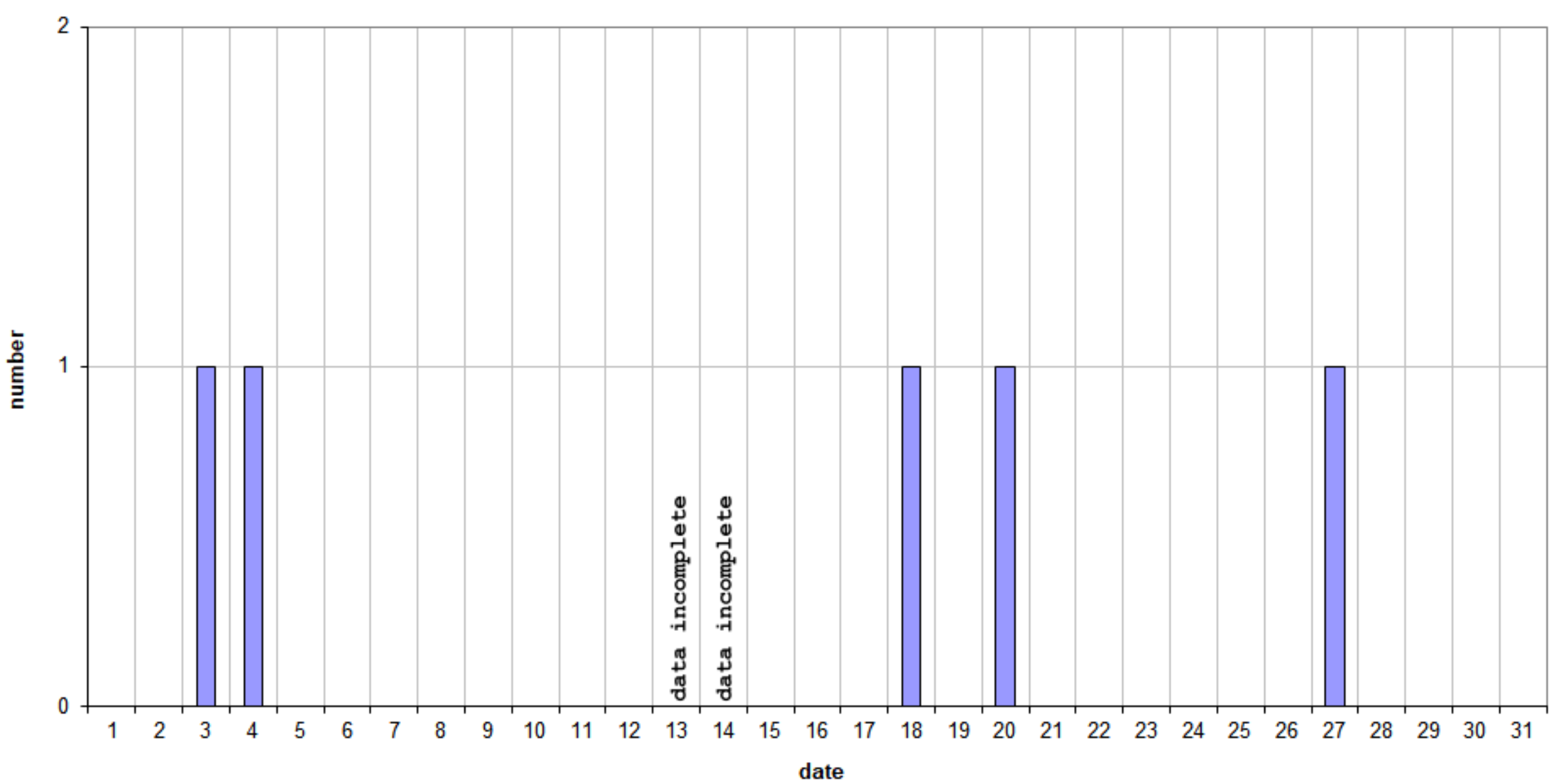
49.99MHz - RadioMeteors January 2021 daily totals of reflections longer than 1 minute Felix Verbelen (Kamphenhout)
