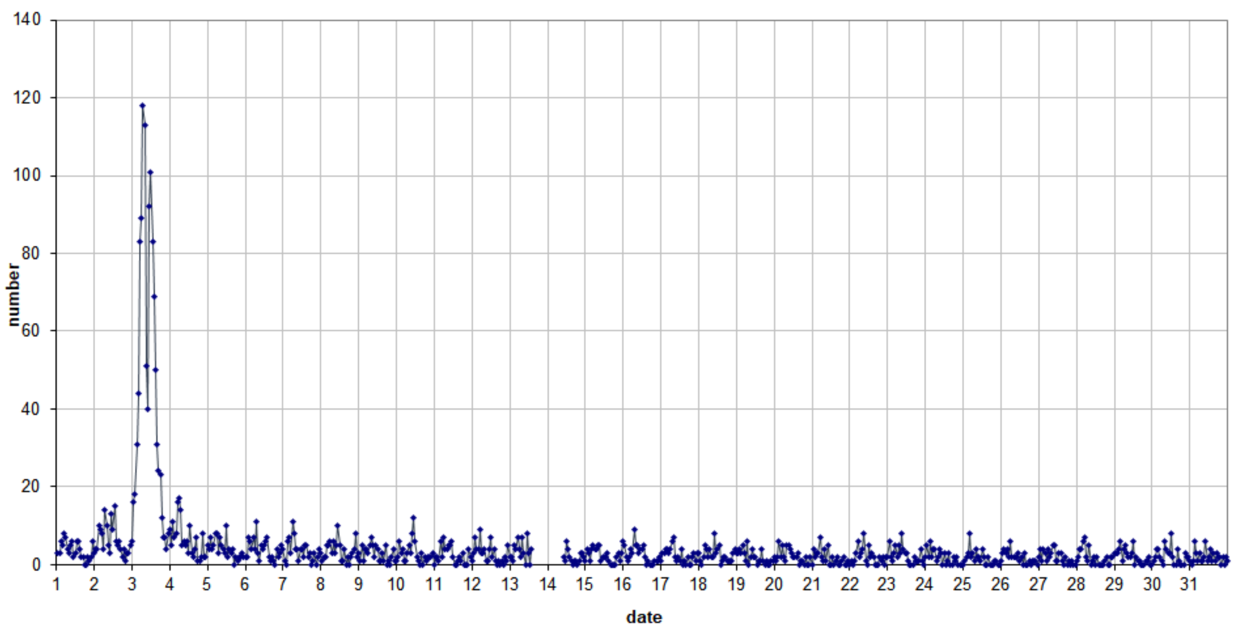
49.99MHz - RadioMeteors January 2021 number of reflections >10 sec per hour Felix Verbelen (Kamphenhout)
