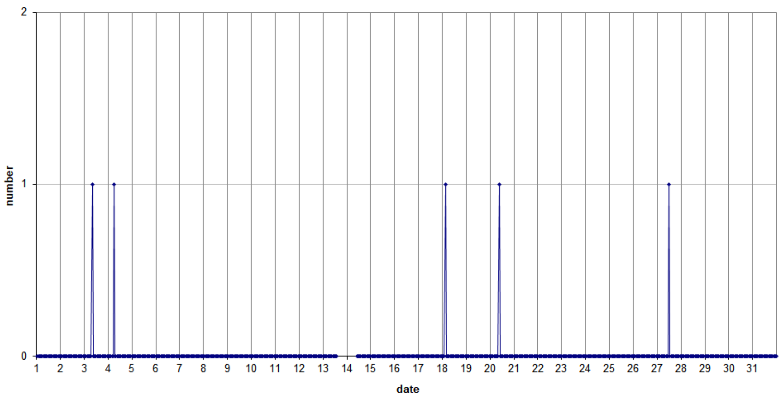
49.99MHz - RadioMeteors January 2021 hourly totals of overdense reflections longer than 1 minute Felix Verbelen (Kamphenhout/BE)
