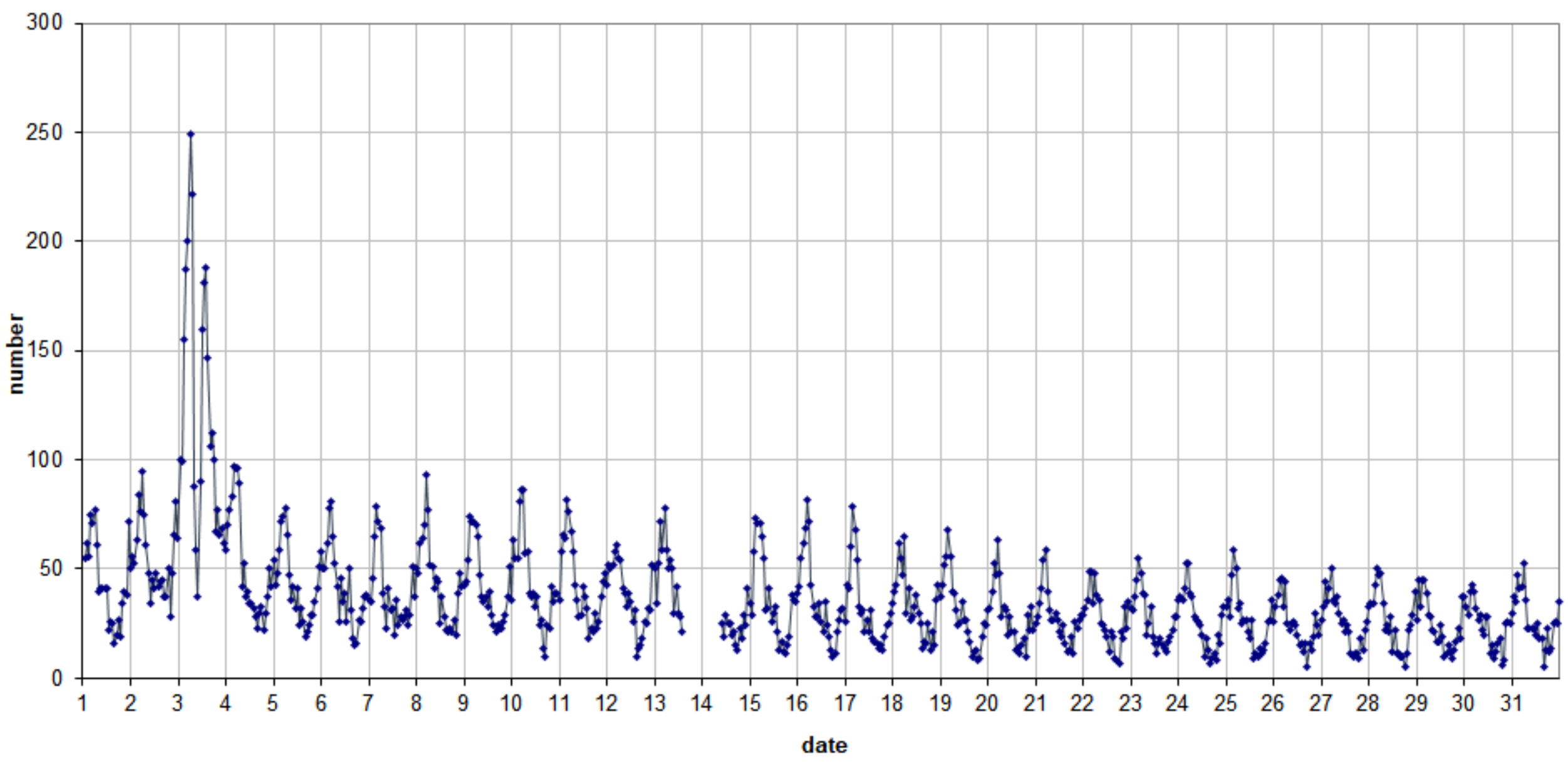
49.99MHz - RadioMeteors January 2021 number of overdense reflections per hour Felix Verbelen (Kamphenhout)
