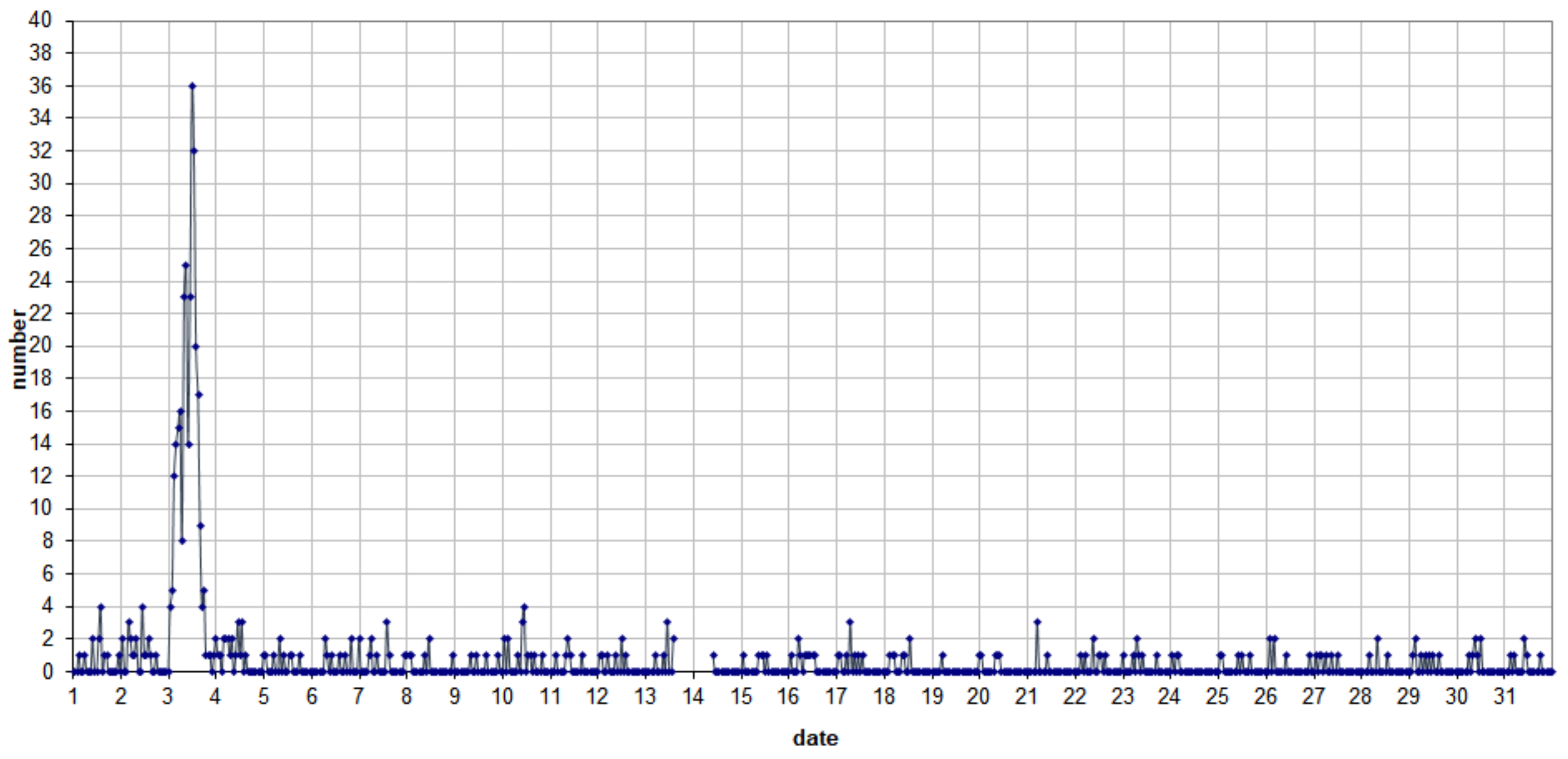
49.99MHz - RadioMeteors January 2021 hourly totals of overdense reflections longer than 1 minute Felix Verbelen (Kamphenhout/BE)
